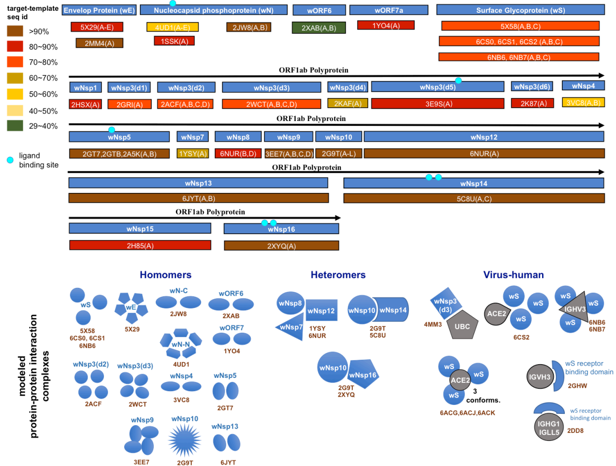
Figure 1. Structural genomics and interactomics road map. Shown are the individual proteins and protein complexes that were targeted for structural characterization together with PDB ID of their templates from Protein Data Bank (PDB).
