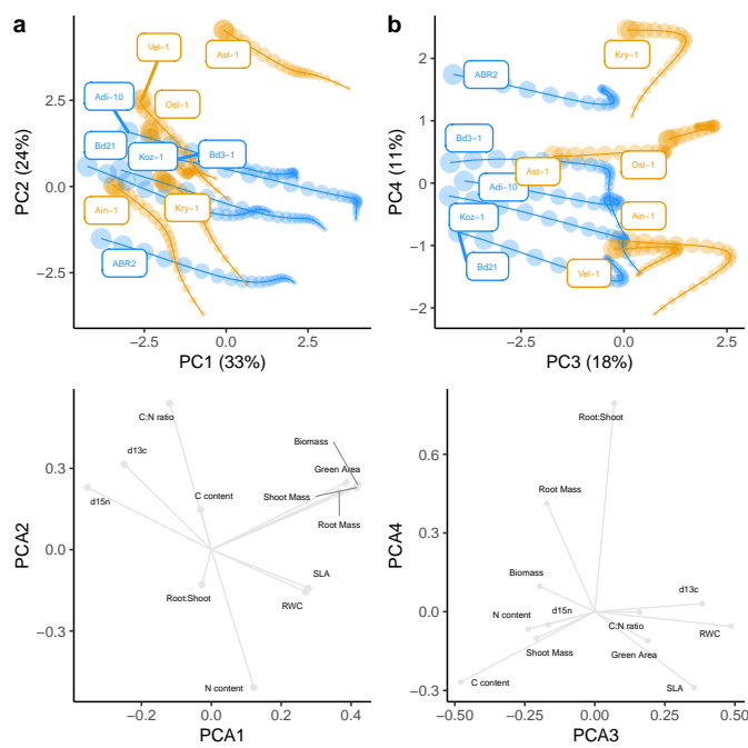
Figure S5. Plasticity through multivariate trait space. Principal component analysis of scaled phenotypic responses to soil moisture gradient among genotypes of both species. Upper panels show genotype means across soil moisture content. Percent values in axis titles indicate percent variance explained by that principal component. Lower panels show eigenvectors of each trait. (a) PC1 and PC2. (b) PC3 and PC4. B. sylvaticum is colored in orange and B. distachyon blue.
