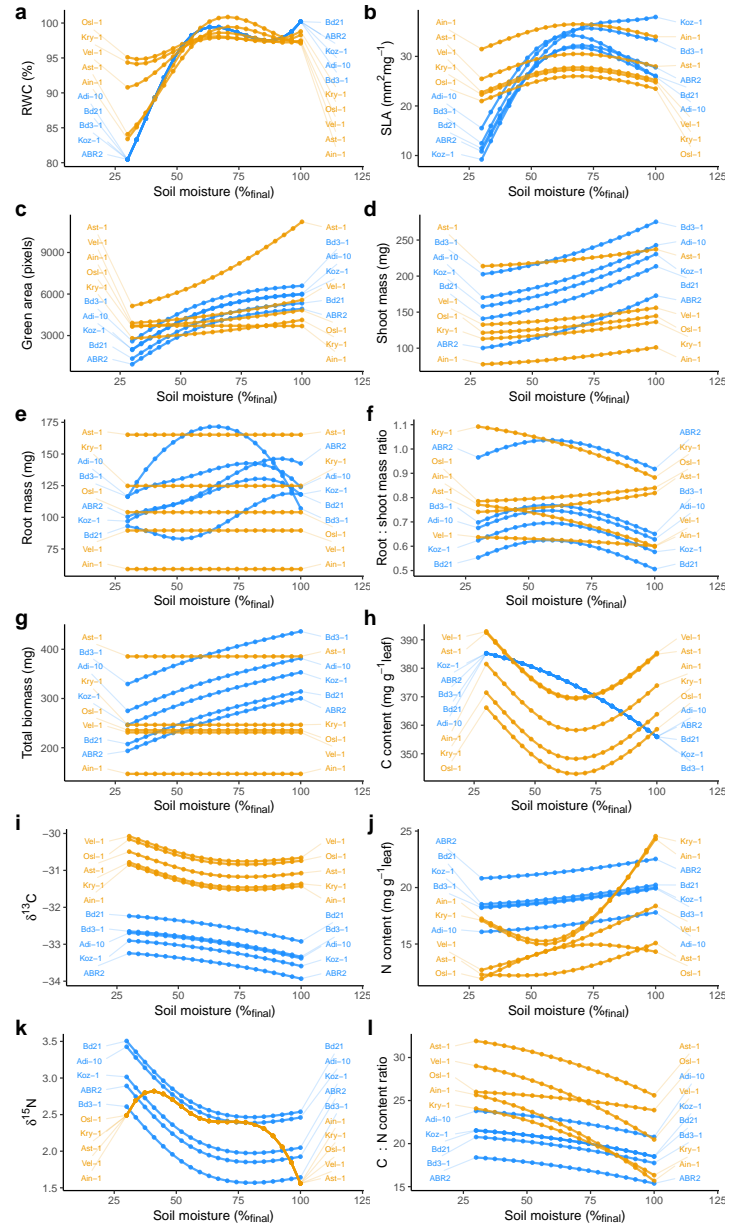
Figure 2. Variation in phenotypic responses to soil moisture gradient as function-valued traits. Points and the lines connecting them indicate predicted values at different levels of gravimetric soil moisture content from 30% to 100%. B. sylvaticum genotypes are colored orange and B. distachyon blue. (a) RWC (b) SLA (c) Green Area (d) Shoot Mass (e) Root Mass (f) Root:Shoot (g) Biomass (h) C content (i) \delta^{13}C (j) N content (k) \delta^{15}N (l) C:N ratio
