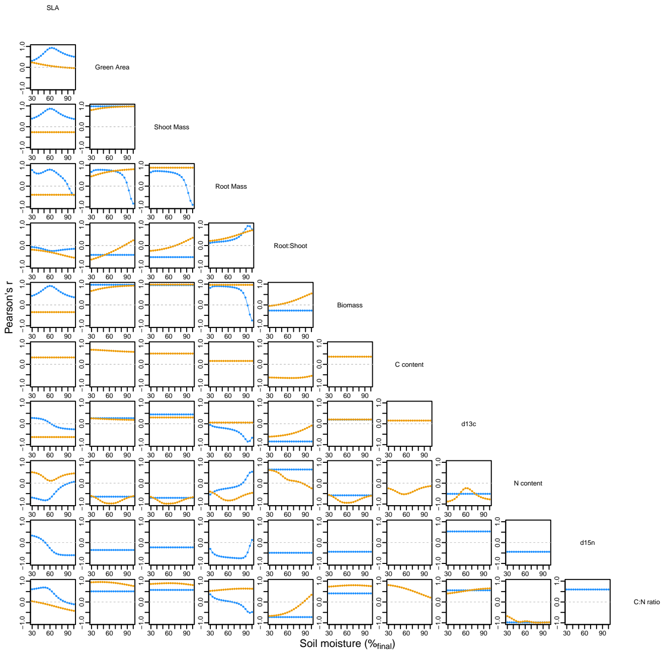
Figure 4. Relationships between trait correlations and soil moisture content. Each point is a correlation coefficient calculated across five genotypes between the intersection of the two traits labeled on the diagonal. Correlations were calculated among genotypes by species (blue = B. distachyon , orange = B. sylvaticum ). Correlations are not shown for traits in species where genotype was not included in final model (Table 1).
