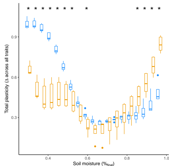
Figure 3. Plasticity through multivariate trait space. (a) Plasticity across all traits was calculated as distance between scaled phenotype for each genotype between different levels of soil moisture. Box plots indicate species median and 25th and 75th percentiles with whiskers extending to 1.5 times the interquartile range. "*" indicates significant differences between species (t-test, \alpha < 0.05 ). B. sylvaticum is colored in orange and B. distachyon blue.
