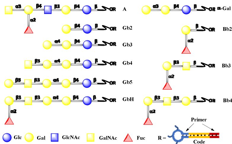
Figure 3. Glycans used in DEGL-10. Globo-series (GbH, Gb5, Gb4, Gb3, Gb2, Bb4, Bb3 and Bb2), blood group A glycan (A antigen) and \alpha -Gal.
