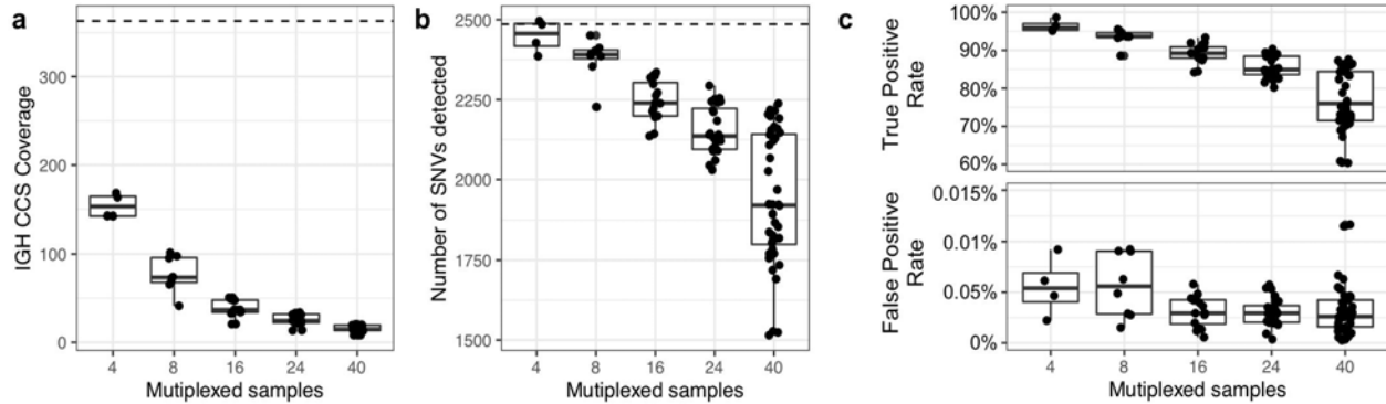
Fig 6. Assessment of sample multiplexing on assembly coverage and variant calling
