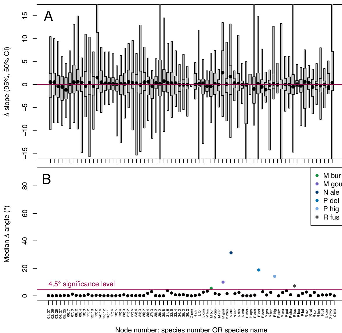
Figure 3: Phylogenetic rarefaction: boxplot showing confidence intervals (95%, 50%) and median value (black point) for each clade after 100 rarefaction replicates (A). Median delta slope angle ( ^{\circ} ) is the difference between the observed and rarefied slopes. Each point gives the clade's median delta slope as compared to the 4.5 ^{\circ} significant change in angle line (B). The x axis gives both the node number from figure 1 and the number of species included in that node from figure 1; monospecific clades have only species abbreviation. Outliers are colored and identified in the legend.
