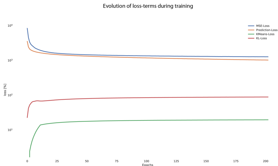
Figure S.2: Training error for all loss-terms employed in the model.
