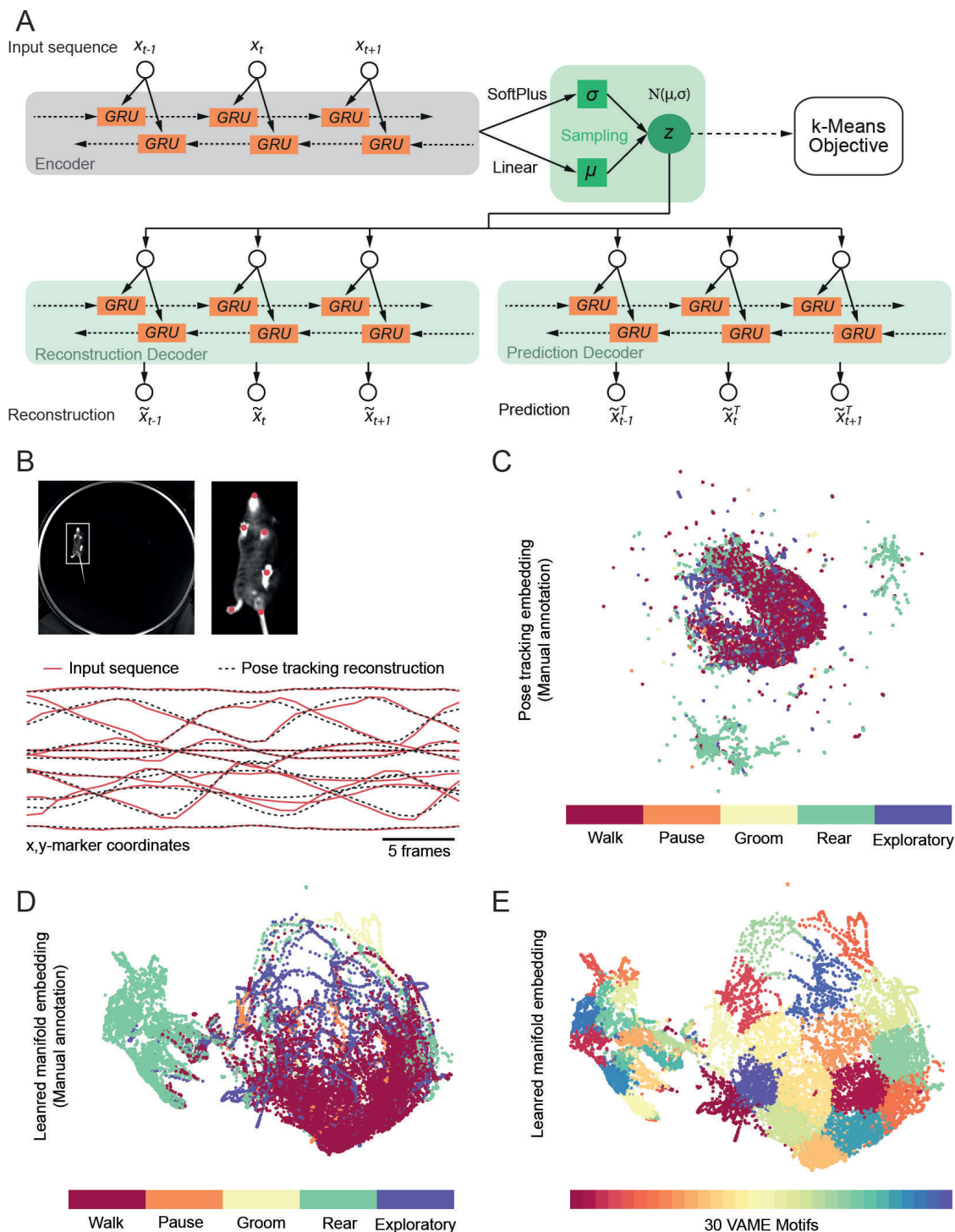
Figure 1: VAME: a machine learning model for unsupervised spatiotemporal behavior quantification. (A) Architecture of the machine learning model. The input sequence is fed into a bidirectional recurrent neural network (encoder) which learns a probabilistic representation z of the underlying hidden states. Another recurrent neural network (decoder) learns to reconstruct the original sequence from z . An additional prediction decoder can be used to anticipate the evolution of the time series. (B) Upper: Markerless pose estimation of animals performing in open-field setup, where marker positions are aligned to egocentric coordinates. Lower: Exemplary input time series reconstructed from the recurrent neuronal network decoder. (C-E) Unifold Manifold Approximation (UMAP) embeddings of the marker position input series (C) and the latent representation encoded from the RNN color-coded for 5 manually labeled behavioral classes (D). (E) Same as (D) but color-coded according to assignment into 30 VAME motifs.
