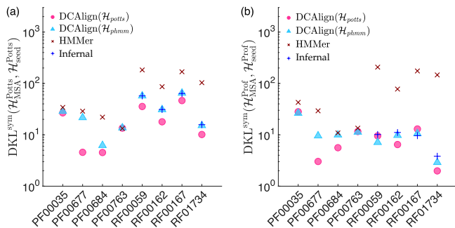
FIG. 9. Symmetric Kullback-Leibler distances. We plot the symmetric KL distance between the MSA and the seed alignment, computed via a Potts model (a) or a profile model (b), for all the families and all the alignment methods we considered.
