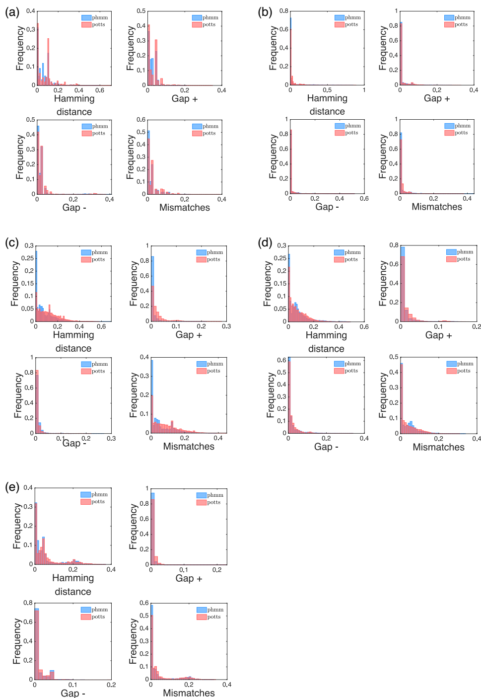
FIG. 12. Distances distribution. We plot here the histograms of the Hamming distances, Gap + , Gap - and Mismatches for the protein families PF00684 (a), PF00763 (b) using as reference the HMMer results and as target the DCAIalign results, and for RF00059 (c), RF00167 (d) and RF01734 (e) using as reference the Infernal results and as target the DCAIalign results.
