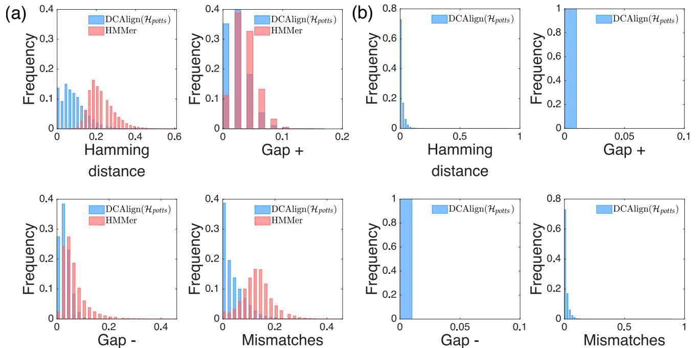
FIG. 5. Comparison between DCAAlign and HMMer for synthetic data. Panels (a) and (b) show the histograms of the normalized metrics (Hamming distance, Gap+, Gap- and Mismatches), respectively, in the case of conserved sites only, and of correlated pairwise columns only. Here, the reference is the ground truth and the target is the alignment of DCAAlign (blue) or HMMer (red). In (b) HMMer results are not shown because hmmsearch does not find any relevant hit.
