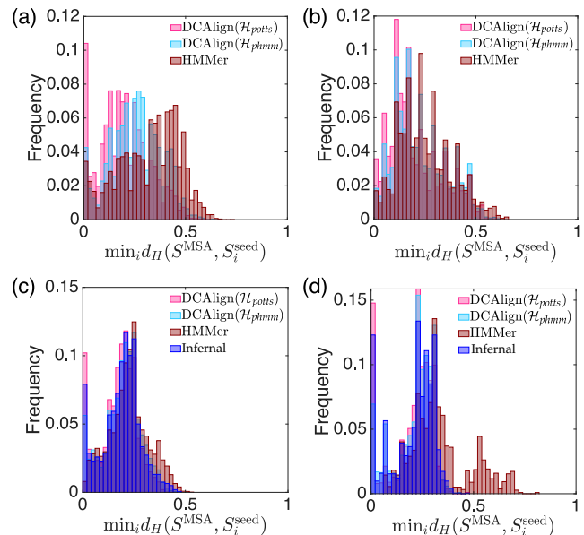
FIG. 10. Distribution of proximity measures. Histograms of the minimum distances computed according to Eq. (32) for the full set of aligned sequences obtained by DCAAlign- potts , DCAAlign- phmm , HMMer, and Infernal, against the seed. Panels (a), (b), (c) and (d) refer to the families PF00677, PF00684, RF00162, RF01734 respectively.
