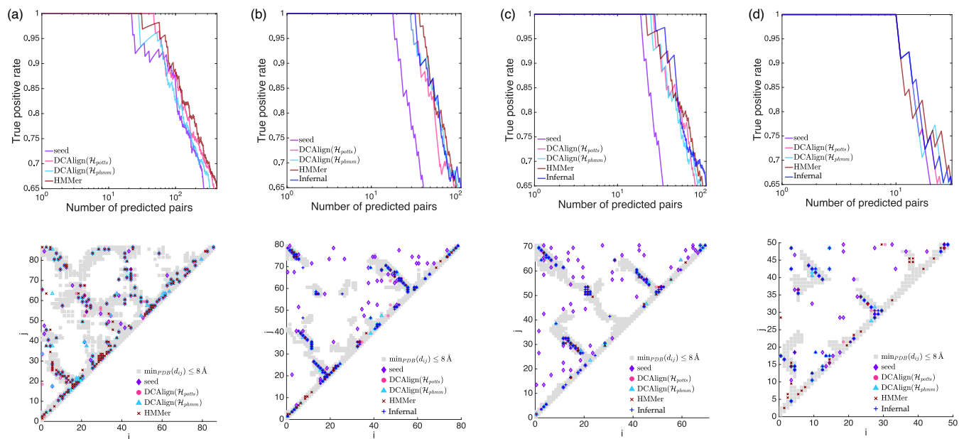
FIG. 14. Contact predictions. We show the Positive Predictive Value curves on the top panels and, on the bottom ones, the contact map retrieved by a set of known crystal structures (gray squares) and the Frobenius norms (computed from the full set of aligned sequences or the seed), for (a) PF00677, (b) RF00059, (c) RF00167 and (d) RF01734.
