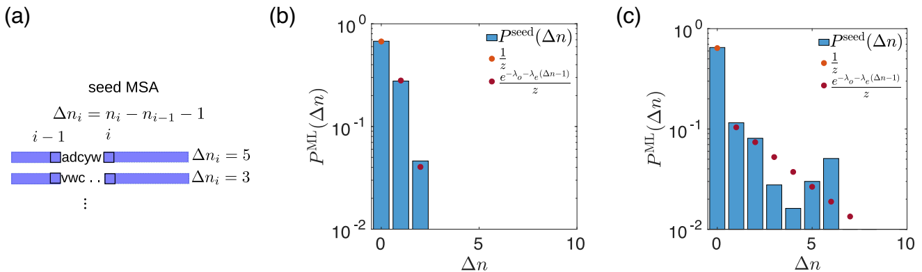
FIG. 3. Inference of Insertion penalties. (a) Schematic representation of the \Delta n variables: the number of insertions between two consecutive positions in the alignment can be computed from the pointer variables \mathbf{n} . (b),(c) Examples of fitting of the empirical probability of \Delta n using our maximum likelihood approach for (b) position 25 and (c) position 92 for RF00162. In (c) the data distribution does not show an exponential profile but our approximation fits well the empirical probability for most of the observed \Delta n .
