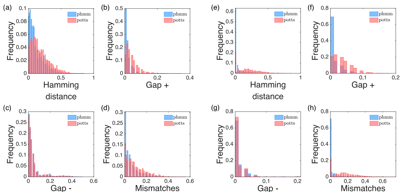
FIG. 7. DCAlign vs state-of-the-art methods for PF00035 and RF00167. We plot here the histograms of the Hamming distances, \text{Gap}_+ , \text{Gap}_- and Mismatches for the protein family PF00035 (a, b, c, d) using as reference the HMMer results and as target the DCAlign results, and for the RNA family RF00167 (e, f, g, h) using as reference the Infernal results and as target the DCAlign results.
