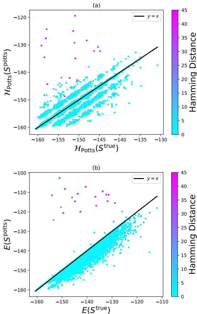
FIG. 6. Energies of synthetic sequences. We show here the scatter plots of the DCA energy (or Potts Hamiltonian) in (a) for the true synthetic sequences (x-axis) against the ones aligned by DCAAlign ( H_{\text{potts}} ) (y-axis). In (b), same plot using the total cost function E .
