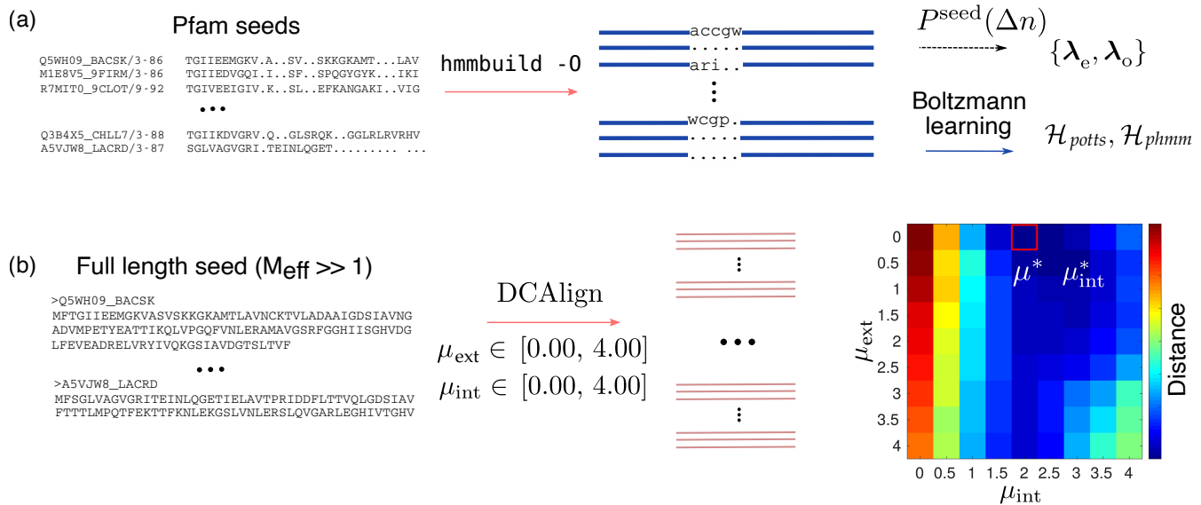
FIG. 4. Scheme of the training process for DCAAlign. In (a) we show the first step of the learning. We build the aligned seed of a Pfam family using hmmbuild -0 to detect the matched amino-acids (blue line) and the insertions (shown in lower case letters and “.”). From these data we learn the DCA Hamiltonian and the affine insertion penalties. In (b) we pictorially describe the learning of the gap penalties. Here we take into account the seed itself (not only the aligned part but the entire sequences) and we try to align it using the parameters inferred in step (a) using all the 81 possible combinations of \mu_{\text{ext}} and \mu_{\text{int}} , each spanning the interval [0.00, 4.00] . We compare each candidate alignment to the seed alignment, directly using the Hamming distance. The best set of parameters is that minimizing this metric. The plot in (b) shows the (average) Hamming distance of the true and re-aligned seed for the PF00677 family.
