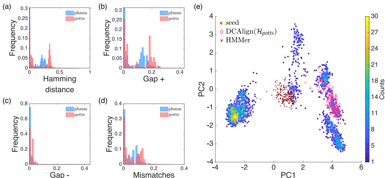
FIG. 8. DCAAlign vs HMMer for PF00677. In (a, b, c, d) we plot the Hamming distance, Gap + , Gap - and Mismatches using the sequences aligned by HMMer as reference and those obtained by DCAAlign as target. In (e) we plot the projections of the seed sequences in the first two principal components of the seed space; the color scale denotes the density of the space. The additional sequences (depicted as pink diamonds if aligned by DCAAlign- potts or as brown crosses if aligned by HMMer) are responsible for the red peak around 0.2 in panel (b).
