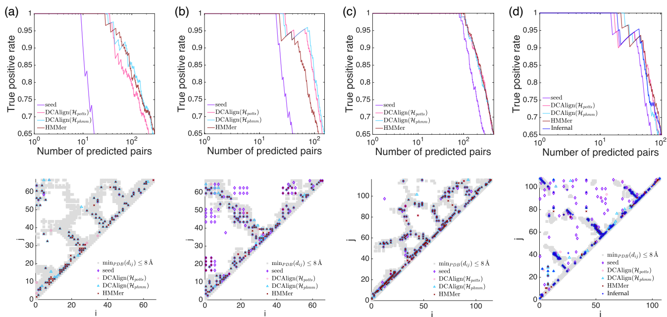
FIG. 11. Contact predictions. We show the Positive Predictive Value curves on the top panels and, on the bottom ones, the contact map retrieved by a set of known crystal structures (gray squares) and the Frobenius norms (computed from the full set of aligned sequences or the seed), for (a) PF00035, (b) PF00684, (c) PF00763 and (d) RF00162.
