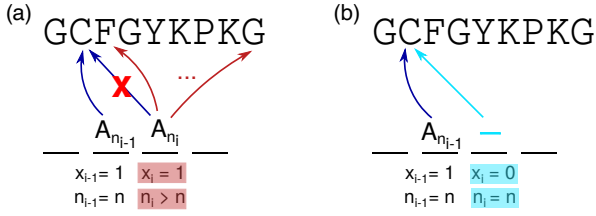
FIG. 2. Short range constraints. We plot in (a) a feasible assignment of two consecutive matched states. If in position i-1 we assign S_{i-1} = A_n , we can then align the next position i to one of the possible amino-acids S_i \in \{A_{n+1}, \dots, A_N\} . As a consequence (x_{i-1}, x_i) = (1, 1) , n_{i-1} = n while n_i \in \{n+1, \dots, N\} . In (b) we plot a feasible inclusion of a gap in position i . If the previous site i-1 points to n_{i-1} = n , we then assign (x_i, n_i) = (0, n) to keep memory of the aligned sequence. In the next position, i+1 , we can match an amino-acid in further positions (according to the constraint in (a)) or add another gap with pointer n_{i+1} = n .
