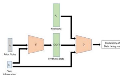
Figure 1: Visualization of the CGAN architecture. A set of prior noise and side information corresponding to sample are used to generate a synthetic sample. The discriminator then uses the side information to predict if a given sample is real or synthetic.
