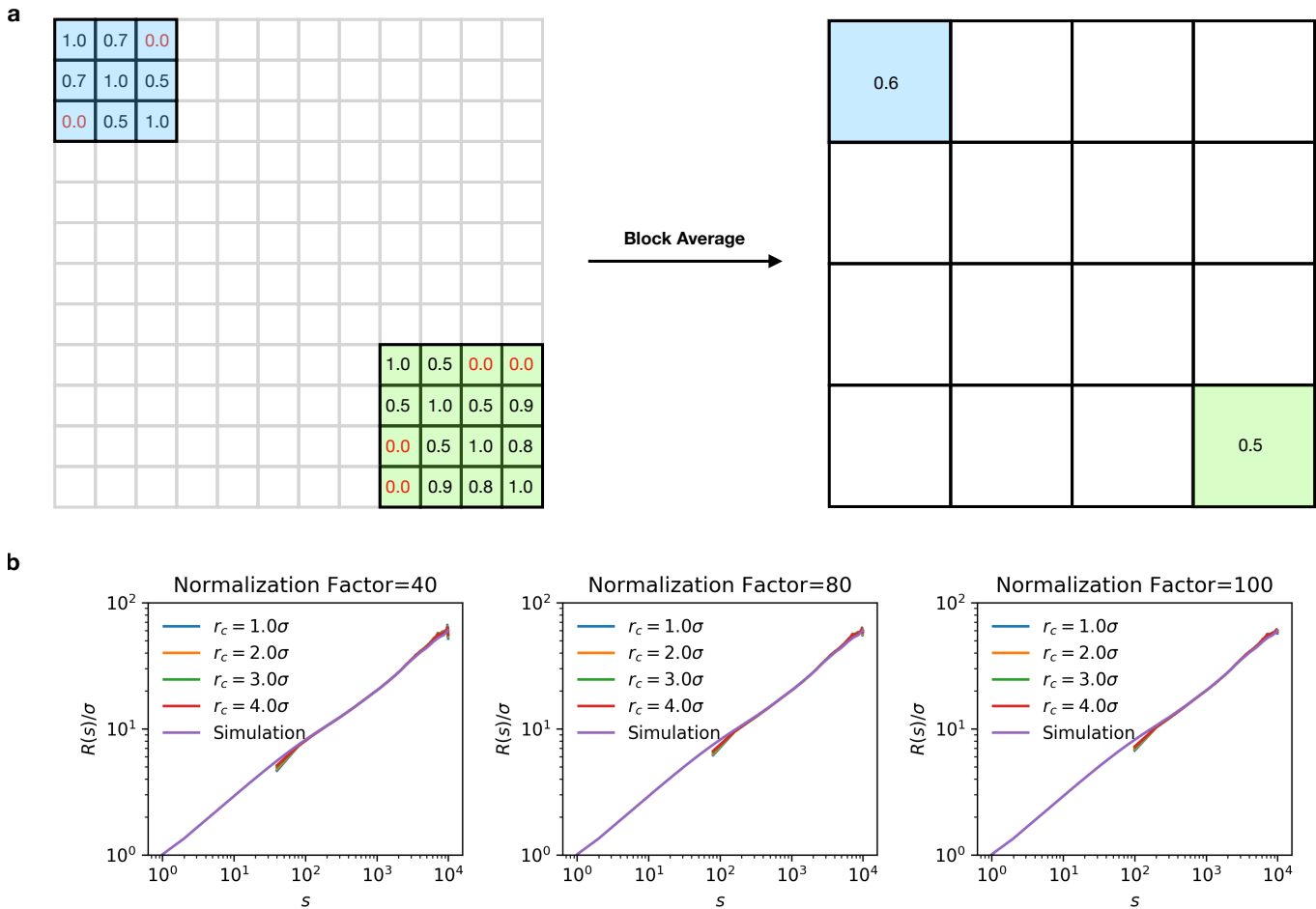
FIG. 10. (a) Illustration of block average performed on sparse contact map matrix ( \langle \mathbf{P} \rangle ). There are zero value elements in the original \langle \mathbf{P} \rangle (matrix on the left). When constructing the distance matrix, \langle \bar{\mathbf{R}} \rangle , from such \langle \mathbf{P} \rangle , the zero value contact probability would naively imply that \langle \bar{r} \rangle \rightarrow \infty . To overcome this problem, we use block averages. The original N \times N \langle \mathbf{P} \rangle are replaced by blocks with size n (red blocks on top left). The value of the matrix element in each block is computed as the mean value of the original elements in each block (matrix on the right). The size of the matrix is reduced from N to N/n where n is the normalization factor. The same procedure could also be applied to \langle \bar{\mathbf{R}} \rangle . (b) Block average does not alter the information embedded in the original \langle \mathbf{P} \rangle and the calculated \langle \bar{\mathbf{R}} \rangle . R(s) is computed for different values of the normalization factor, n . The insensitivity of the results to the block averaging justifies its use in overcoming the problem of missing data points on the \langle \mathbf{P} \rangle .
