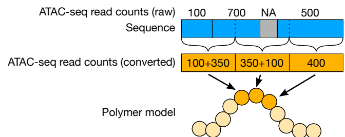
FIG. 12. The procedure for processing ATAC-seq peak data. The raw ATAC-seq read counts data is illustrated at the top track. Each chromatin segment has a read count value. The segments are not distributed uniformly, but have different lengths, and have missing parts. In our model, each locus has a fixed genomic length. Thus, to estimate the read counts associated with each locus, we calculate the contribution from the original ATAC-seq segments (blue track) to the segments represented by the locus (yellow track).
