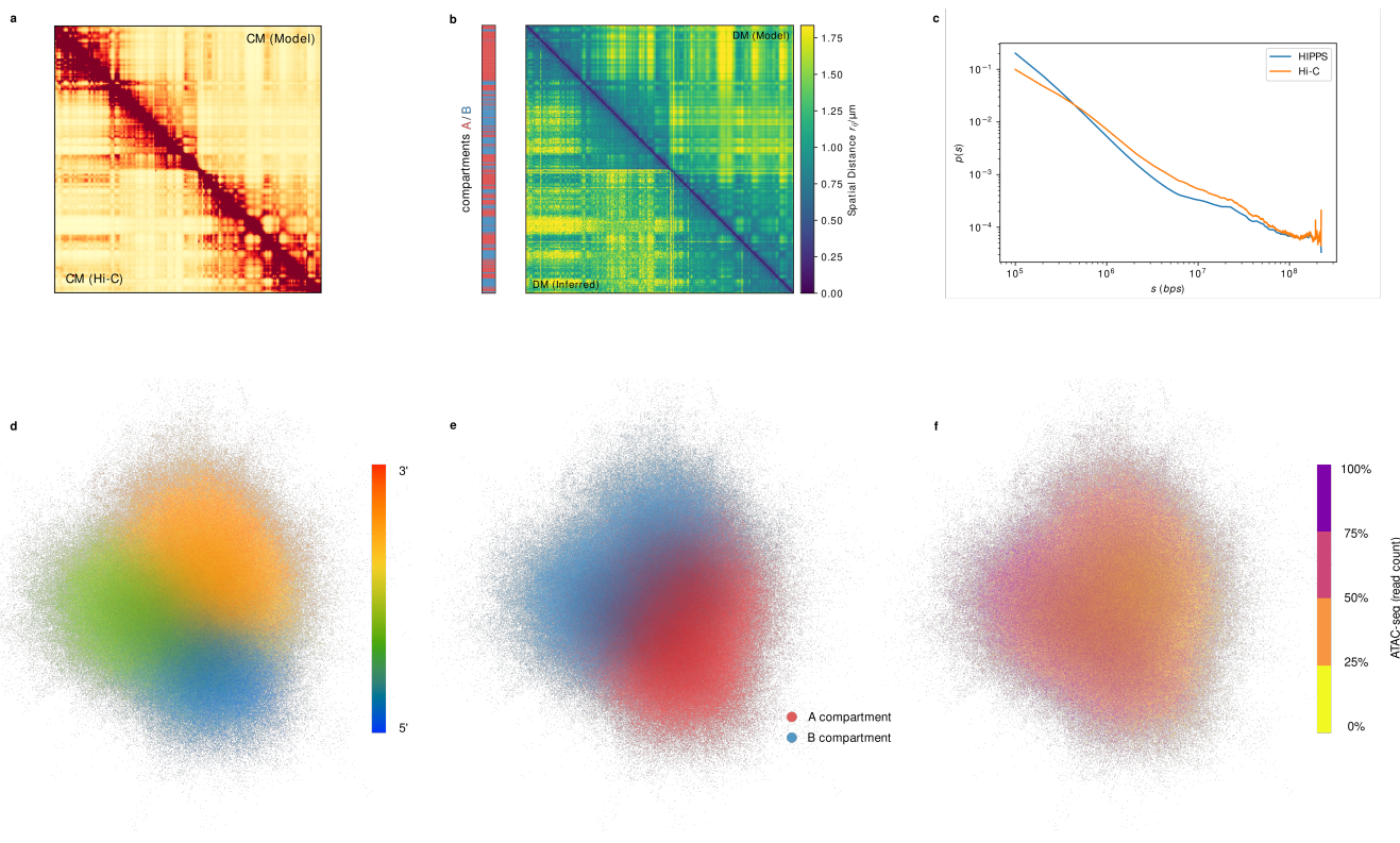
FIG. 5. (a) Comparison between the Hi-C (lower triangle) and the contact maps calculated from an ensemble of 3D structures for Chromosome 1 using the HIPPS method ( \langle\langle\mathbf{P}\rangle\rangle \rightarrow \langle\langle\mathbf{R}\rangle\rangle \rightarrow 3\text{D structures} \rightarrow \text{contact map} ). (b) Comparison between the distance matrix inferred from the Hi-C data (lower triangle) and the distance matrix calculated from an ensemble of 3D structures for Chr1 using the HIPPS method ( \langle\mathbf{P}\rangle \rightarrow \langle\mathbf{R}\rangle \rightarrow 3\text{D structures} \rightarrow \text{mean distance map} ). A/B compartments, determined using spectral biclustering [29] are also shown. (c) Comparison between the contact probability profile P(s) inferred from experiment and the calculated curve using the HIPPS method. The cloud representation demonstrates the probabilistic nature of chromosome conformation, with color representing the genomic location of the loci along the genome. The resolution of the locus is 100 kbps. (e) Same cloud point representations as (d) with colors indicating the A/B compartments. Phase separation between A/B compartments is vividly illustrated. (f) Same as (d) and (e) but with ATAC-seq read counts coded in color
