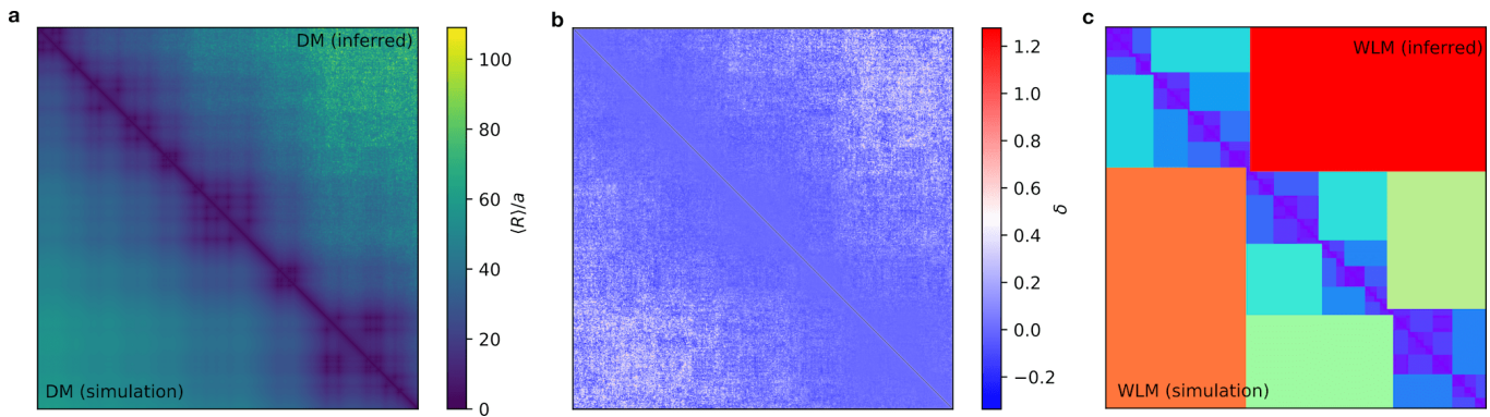
FIG. 1. Comparison of the distance matrices (DM or \bar{\mathbf{R}} ) for the GRMC. (a) The simulated \bar{\mathbf{R}} (lower triangle) and the constructed \bar{\mathbf{R}} (upper triangle) are compared side by side. The color bar indicates the value of the mean spatial distance, \langle R_{mn} \rangle . The constructed \bar{\mathbf{R}} is obtained by solving Eq.3 using the contact probability \mathbf{P} (calculated using Eq.12). The matrix size is 2000 \times 2000 after the block averaging is applied to the raw data (Appendix C). The threshold value for contact is r_c = 2.0a . The location of the loop anchors are derived from experimental data [6] over the range from 146 Mbpts to 158 Mbpts for Chromosome 5 in the Human GM12878 cell line. (b) Relative error \delta is represented as a heatmap. The relative error is calculated as, \delta = (d_i - d_s)/d_s , where d_i and d_s are the inferred and simulated distances, respectively; \delta increases for loci with large genomic distance indicating the tendency to overestimate the distances for loci pairs with small probabilities. (c) Ward Linkage Matrices (WLMs) from the simulation and theoretical predictions, shown in the lower and upper triangle, respectively, are in excellent agreement with each other.
