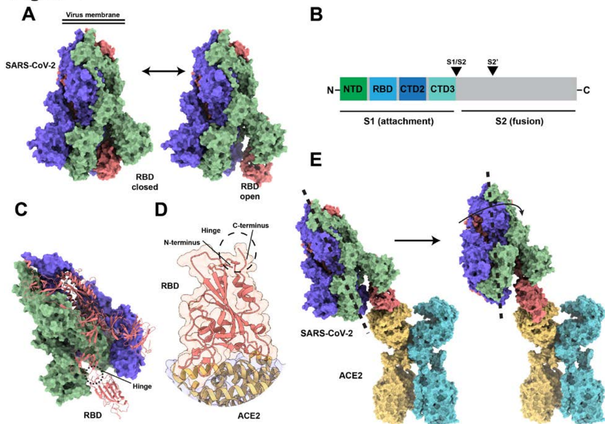
Figure 1. Structural comparison of SARS-CoV-2 S protein conformational states. (A) Surface diagram of SARS-CoV-2 homotrimeric structure in the unbound- closed and open conformations. (B) Structural illustration of S protein, including functional domains (NTD, N-terminal domain; RBD, receptor-binding domain; CTD2, C-terminal domain 2; CTD, C-terminal domain 3; and proteolytic cleavage sites (S1/S2, S2')). (C) S trimer with one RBD in the open conformation and (D) RBD-ACE2 complex shown as a cartoon. (E) Superposed structures depicting the conformational changes between the unbound-open (left) to the ACE2-bound state.
