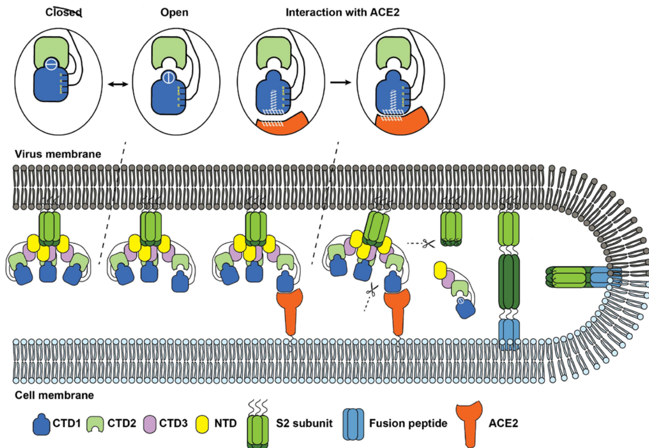
Figure 7. Proposed model for the pre- to post-fusion transition of SARS-CoV-2 S protein. The closed and open transitions are associated with the dissociation of RBD and CTD2 and conformational changes in the hinge region, including disulfide bond rearrangement. The complex of SARS-CoV-2-RBD with ACE2 induces conformational changes and rearrangement of the disulfide bonds that stabilize the S protein in the active form. The Activated S protein is cleaved by host proteases and induces the pre- to post-fusion transition of the S2 subunit, and initiates the fusion of viral and cellular membranes.
