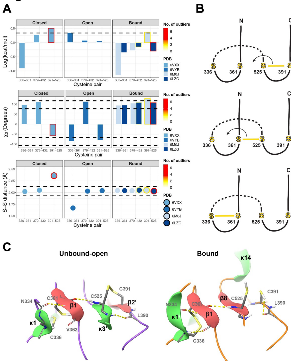
Figure 5. Characterization of the conserved SARS-CoV-2-RBD cysteine pairs. (A) Shown are the disulfide bond energy (top), \chi_3 torsional angle (middle), and S-S distance (bottom) in different conformational states of SARS-CoV-2-RBD (closed – 6VXX:B; open – 6VYB:B; bound – 6MOJ:E and 6LZG:B). Dashed lines show the threshold for ideal disulfide bonds (top panel – below the line; middle and bottom panel – between the lines). The number of outliers, including RSRZ (root-mean-square of Z score) outliers, non-rotameric sidechains, clashes, and bond length and angle outliers, were summarized
