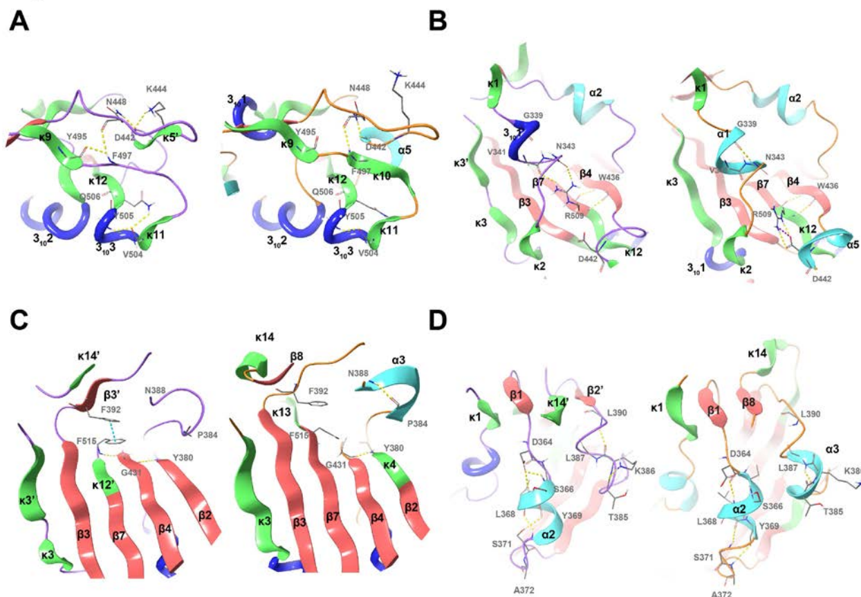
Figure 4. Detailed structural comparison between the unbound and bound SARS-CoV-2-RBD and ACE2.
