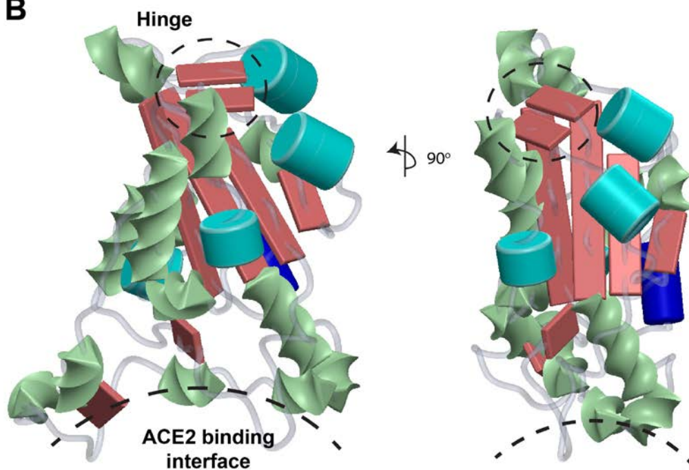
Figure 6. Dynamical features of the SARS-CoV-2-RBD. A summary of the conformational changes between the unbound-closed (6VXX:B in blue) and the bound (6M0J:E in red) RBD states are shown as an interpolated trajectory. (B) A simplified model, demonstrating the association between the secondary structures and the relationship between the distal part (ACE2 binding interface) and the hinge region. \alpha -helices (cyan), \beta -strands (red), and \kappa -helices (green) are illustrated as shown as 3D shapes.
