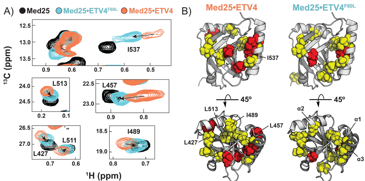
Figure 4. Structural shifts in the Med25 ABD accompany the conformational changes of ETV/PEA3•Med25 complexes. A) Examples of Med25 resonances undergoing shifts toward the unbound position (black) upon ETV4 F60L (cyan) mutation. B) Chemical Shift Perturbations from binding of ETV4 (left) and ETV4 F60L (right). Residues shown in A. are labeled on the structures. Yellow = 0.040–0.080 ppm, red > 0.080 ppm.
