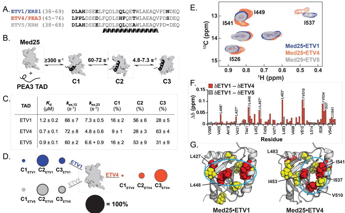
Figure 1. ETV/PEA3 activators differentially engage with Med25. A) Alignment of ETV/PEA3 family activation domains. The helix denotes the residues that undergo coupled folding and binding with Med25, as determined by NMR chemical shift analysis.(30) B) Mechanism of binding of ETV/PEA3 activators to Med25, determined here for ETV1 and ETV4, and previously for ETV5.(32) The range of exchange rates between analogous steps for ETV/PEA3 TADs are shown. C) Table of relevant binding parameters for each ETV/PEA3 TAD, including the equilibrium affinity, exchange rates between C1 and C2 ( k_{\text{ex},12} ) and between C2 and C3 ( k_{\text{ex},23} ), and equilibrium populations of each state. All values represent the average of 3-4 biological replicates, and the error is the standard deviation. D) Equilibrium populations of the three ETV/PEA3•Med25 conformations scaled relative to the diameter of the black circle. Standard deviations of the values are shown as the dark gray outer circle. E) Overlay of the Ile C \delta region of the ^1\text{H} , ^{13}\text{C} -HSQC of Med25 in complex with 1.1 equivalents unlabeled ETV1 (blue), ETV4 (orange), or ETV5 (grey). Peaks that have chemical shift differences between complexes are labeled. Note: I449 and I541 form a single overlapped peak for the ETV1 and ETV5 complexes. Full spectra are in the supporting information. F) Chemical shift differences of Med25 methyl resonances between ETV1 and ETV4 (orange) and ETV1 and ETV5 (grey). G) Chemical shift perturbations induced by binding of ETV/PEA3 activators plotted on the structure of Med25 (PDB ID 2XNF)(34). Yellow = 0.040–0.080 ppm, red > 0.080 ppm. Cyan circles highlight general distinctions in perturbation patterns. Several residues with chemical shift differences >0.030 ppm between the ETV1•Med25 (or ETV5•Med25) and ETV4•Med25 complexes are labeled.
