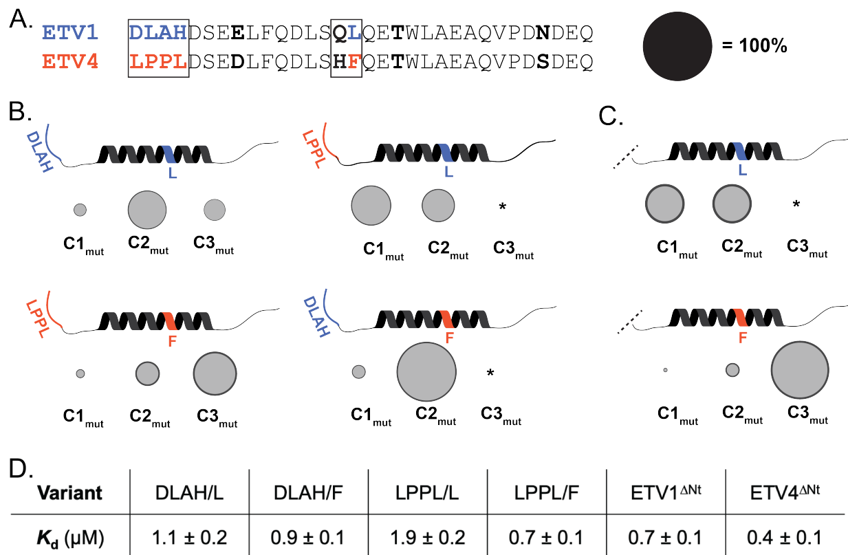
Figure 2. Variable residues in the disordered N -terminus and the helical binding region mediate differences in ETV/PEA3•Med25 conformational behavior. A) Alignment of ETV1 and ETV4 activators with regions that were selected for mutational analysis boxed. Regions/residues that affected the conformational ensemble are color coded to ETV1 (blue) or ETV4 (orange). Effects of the Gln/His residues in the variable motif were also tested but did not affect conformational populations and are thus omitted in B. and C. for clarity. Populations of conformational states in B. and C. are scaled relative to the diameter of the black circle. B) Results from kinetics experiments of mutant TADs, for native (left) and non-native (right) combinations of variable N -termini and helical binding regions. Variants were made based on the ETV4 sequence. The data shown is the average across all the variants tested from each group, with the error (dark grey outer circle) representing the standard deviation. C) Results from kinetics experiments with ETV1 ΔNt (left) and ETV4 ΔNt (right). D) Average equilibrium K_d values of variants tested. *Conformer was undetectable in kinetics experiments (see SI Discussion of Kinetic Data Analysis for further details).
