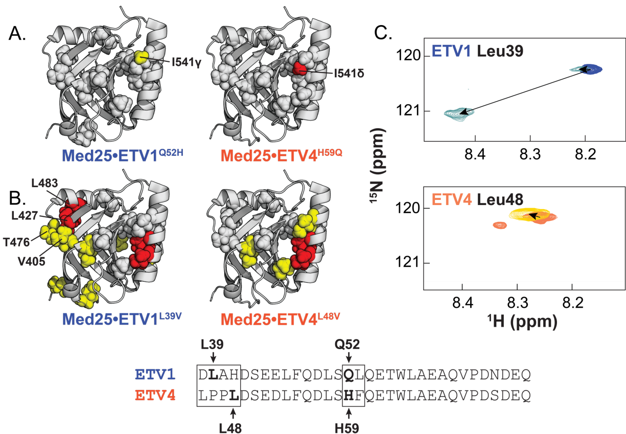
Figure 2. ETV/PEA3 variable regions engage in unique interactions with the Med25 surface. Effects of conservative mutations in the A) helical binding region and B) N -termini are plotted on the structure of Med25. Yellow = 0.015 – 0.030 ppm. Red ≥ 0.030 ppm. Residues discussed in the text are labeled. Grey spheres denote residues that undergo identical perturbations in both parent and mutant complexes. Residues chosen for mutation are bolded and labeled in the alignment. C) Chemical shift perturbations of 150 μM ETV1 (above) and ETV4 (below) TADs in the absence (blue and orange, respectively) and presence (light blue and maroon, respectively) of 280 μM unlabeled Med25. TADs were selectively 15 N labeled at the positions noted. Small secondary peaks in free ETV4 spectra were observed and likely arose from isomerization of the two tandem Pro residues in the N -terminal region.
