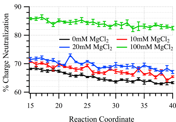
Figure 2. Percent charge neutralization (%CN) based on an 8 Å cutoff from all heavy atoms of twister at various stages of the reaction coordinate.
