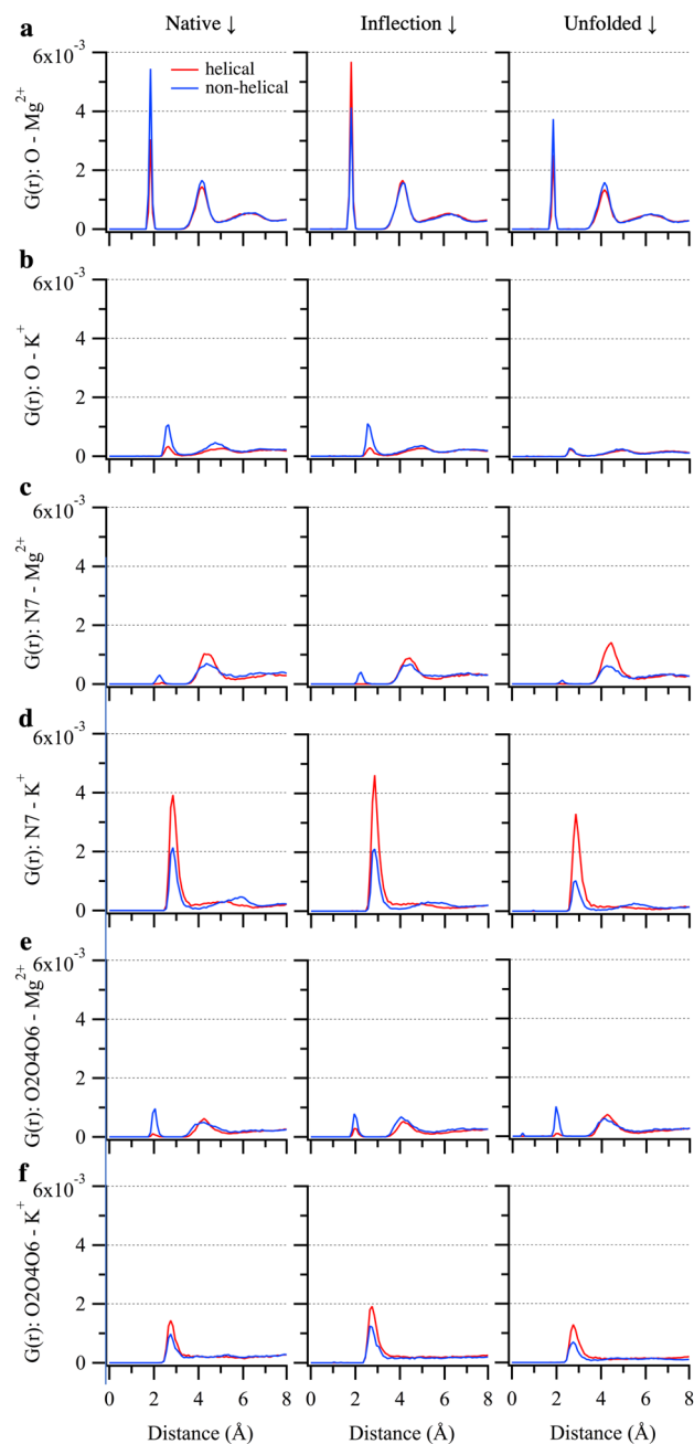
Figure 8. Radial Distribution Functions (RDF) of Mg^{2+} (a, c, e) and K^+ (b, d, f) around NBPOs, Ade-N7/Gua-N7, and O2/O4/O6 atoms of nucleobases that participate or don't participate in helical structures, respectively. From left to right the plots correspond to RDFs calculated at native state (RC=14-16), inflection point (RC=19-21) and unfolded state (RC=38-40) for 100mM MgCl_2 . Red line – Helical region, Blue line – Non-helical region.
