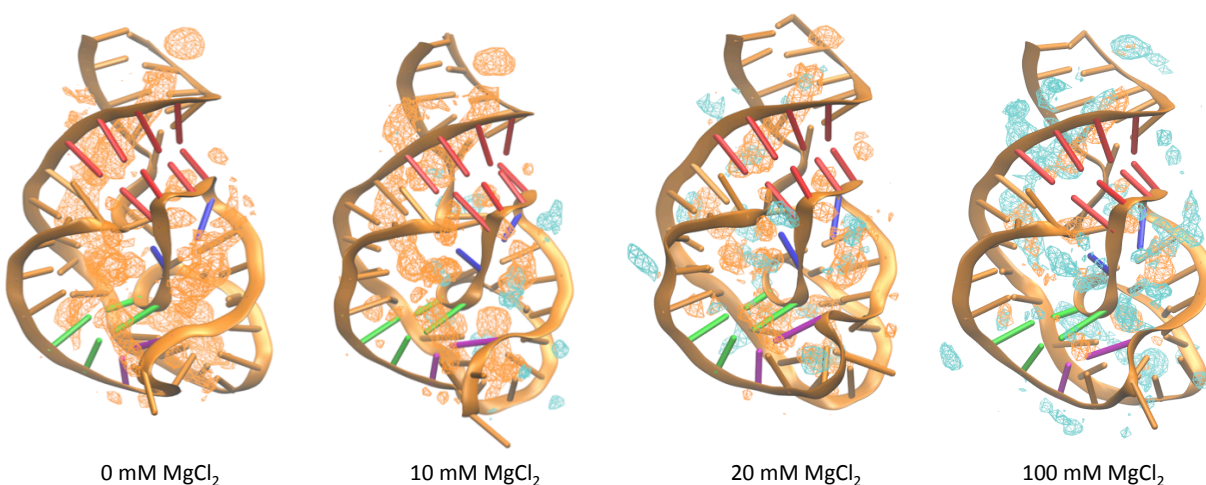
Figure 3. GFE maps for Mg^{2+} (cyan mesh) and K^+ (orange mesh) distributions around the native state of Twister at different Mg^{2+} concentrations. The GFE maps are contoured at -2.5 kcal/mol.
