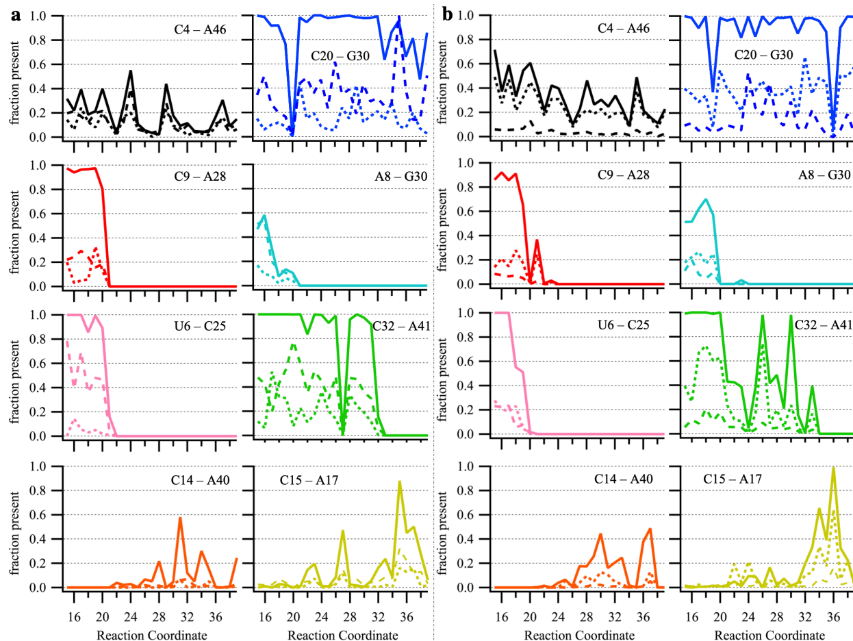
Figure 5. Adjacent NBPO pairs in contact with Mg^{2+} and K^+ ions at a) 20mM and b) 100 mM MgCl_2 . Shown is the probability of selected NBPO pairs within 9 Å (solid line) and the probability of Mg^{2+} (dotted line) or K^+ ions (dashed line) within 6.5 Å of NBPOs of both phosphates.
