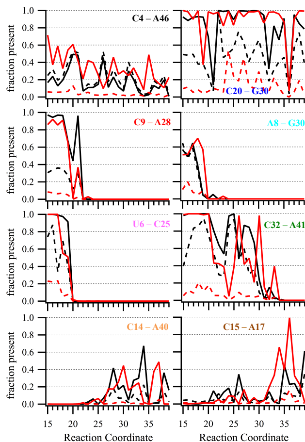
Figure 4. Adjacent non-bridging phosphate oxygen (NBPO) pairs in contact with K^+ ions at 0 mM MgCl_2 (black lines) and at 100 mM MgCl_2 (red lines). Shown is the probability of selected NBPO pairs within 9 Å (solid lines) and the probability of K^+ ions (dashed lines) within 6.5 Å of NBPOs of both phosphates.
