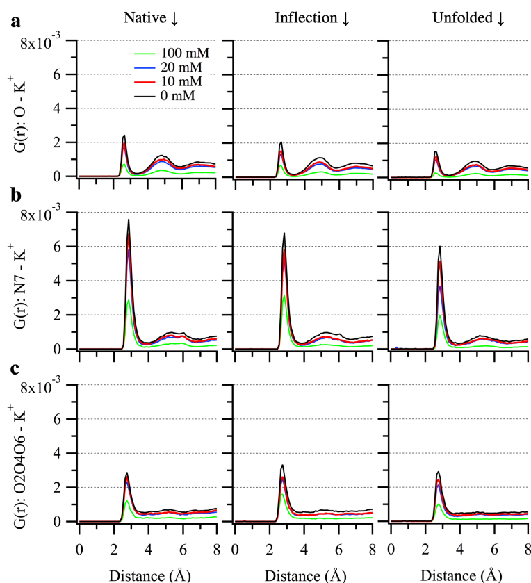
Figure 7. Radial distribution functions of K^+ around a) the non-bridging phosphate oxygens (NBPO), b) the Gua-N7/Ade-N7 atoms, and c) O2/O4/O6 atoms of the nucleobases at native state (RC=14-16), inflection point (RC=19-21) and unfolded state (RC=38-40).
