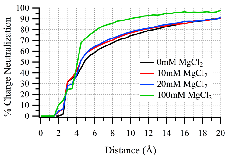
Figure 1. Percent charge neutralization by counterions at the native state (RC = 14 – 16 Å) at different MgCl_2 concentrations as a function of distance from all non-hydrogen atoms of Twister. The dashed line indicated the 76% charge neutralization predicted by counterion condensation theory (see text).
