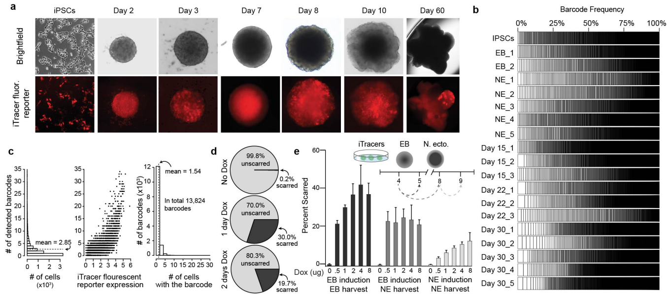
Extended Fig. 1. Assessment of iTracer readouts in iPSC and iPSC-derived cerebral organoids. a) Brightfield and fluorescence imaging of iTracer reporter (RFP) in organoids during cerebral organoid development. b) Stacked barplots showing frequency of unique barcodes detected in bulk targeted amplicon sequencing libraries throughout cerebral organoid development. c) Barplots of the number of iTracer barcodes detected from single-cell transcriptomes. The left panel shows frequencies of cells with different numbers of detected barcodes. The dashed line shows the average number of detected barcodes per cell (2.85). The middle panel shows numbers of barcodes in relation to fluorescent reporter detection. Each dot represents one cell. The right panel shows frequencies of barcodes detected in different numbers of cells. The dashed line indicates that on average one barcode is detected in 1.54 cells. d) Scar detection in iPSCs treated with no doxycycline, 2ug of doxycycline for one day, and 2ug of doxycycline for two days. e) Stacked barplots showing frequencies of different scars detected in 3D cultures treated with 0-8ug of doxycycline at EB and Neuroectoderm stages.
