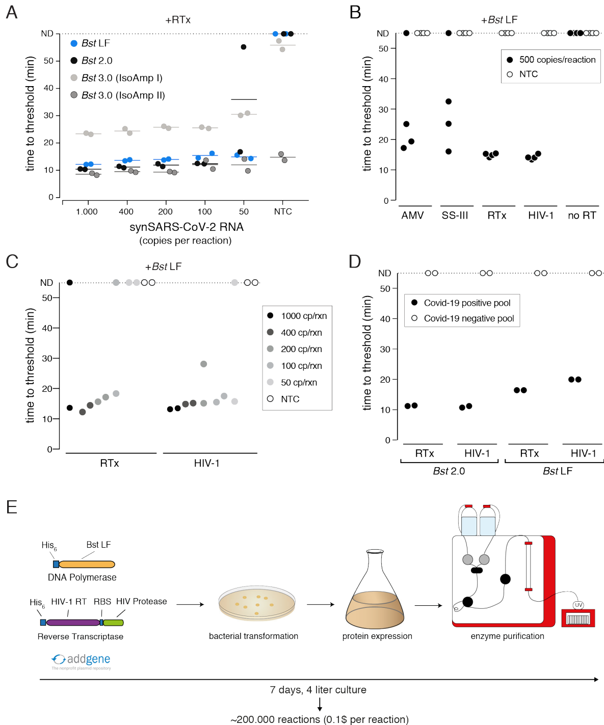
Figure 6: A sensitive RT-LAMP assay based on open-access enzymes.
