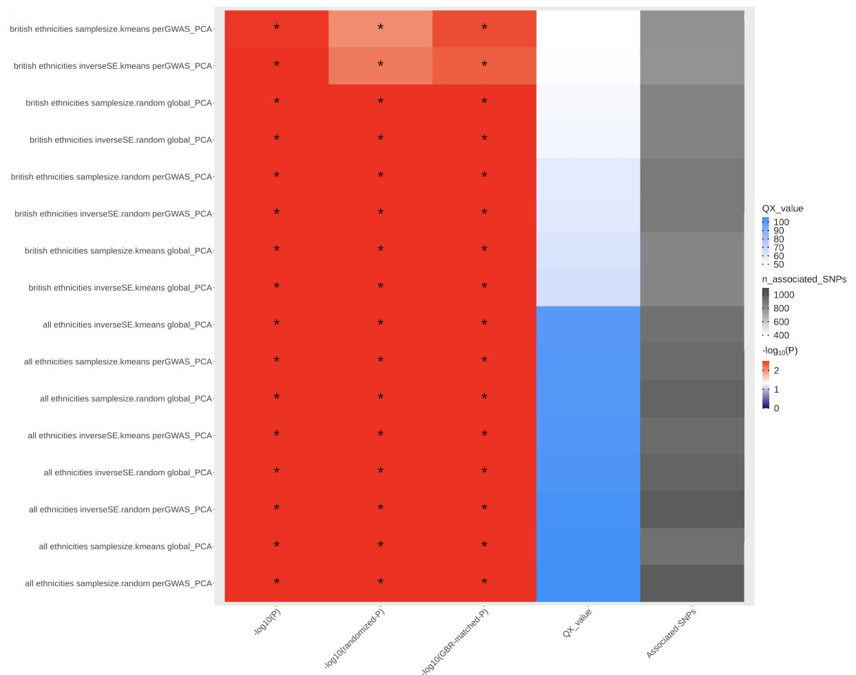
Figure S25: Q_X statistics and P-values for the trait height, obtained by using different types of meta-analysis methods on the UKBB data (inverse variance and sample size based) and two PCA correction approaches (global vs. per-GWAS). The meta-analyses were performed in "all ethnicities" as well as "White-British" set of individuals. The asterisk denotes a significance cutoff for Q_X of P < 0.05 . " -\log_{10}(\text{Chi squared } P) " = -\log_{10}(\text{P-value}) , obtained assuming a chi-squared distribution for the Q_X statistic. " -\log_{10}(\text{randomized } P) " = -\log_{10}(\text{P-value}) , obtained using the effect sign-randomization scheme. All other P-values were obtained by sampling random SNPs from the genome using the allele frequency matching scheme in different populations, as described in the Methods section.
