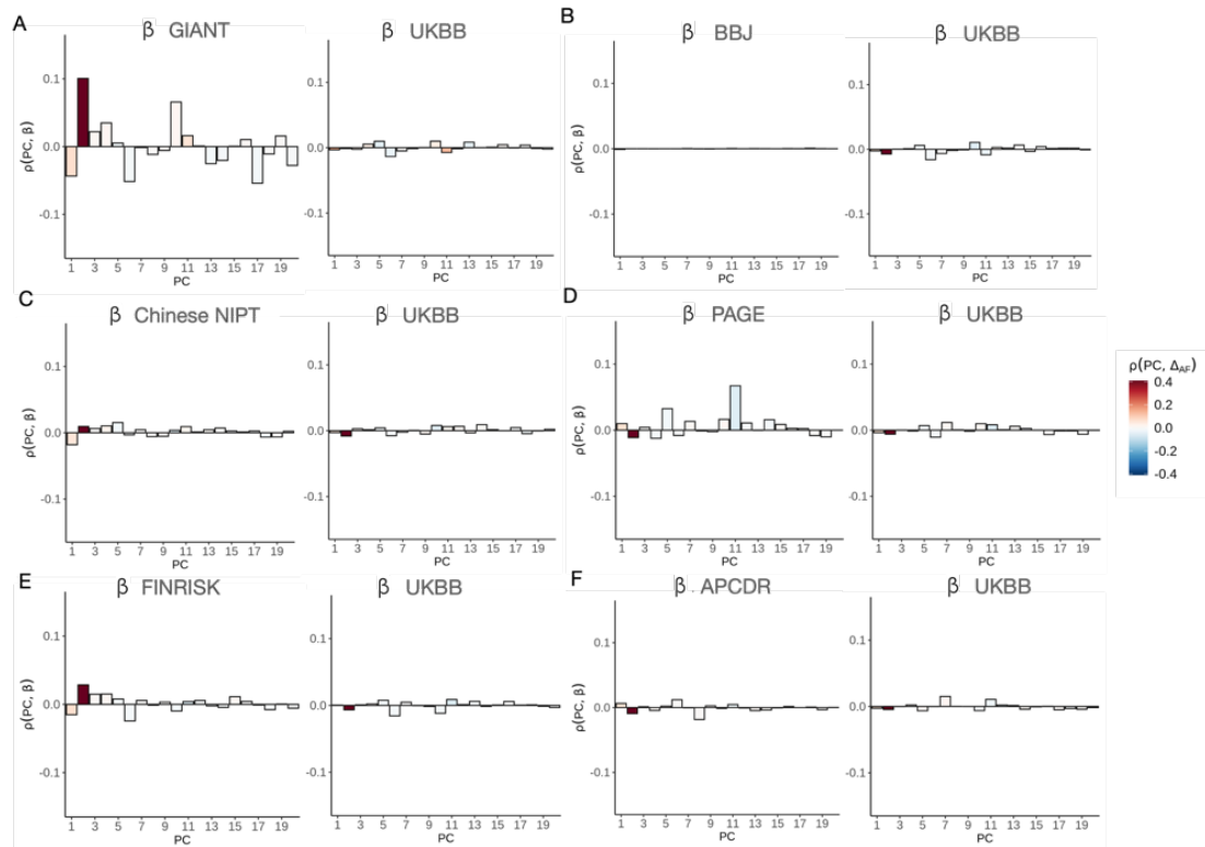
Figure S24: Pearson correlations between 20 PC loadings and height effect size estimates from a non-UKBB GWAS, compared to the same correlation using effect size estimates from the UKBB GWAS, for different choices of non-UKBB GWAS. The correlations were computed using SNPs that are present in both the UKBB and non-UKBB GWAS cohorts, and in the 1000 Genomes Project. The barplots are coloured by the correlation between each loading and the allele frequency difference between GBR and CHB. A) GIANT vs. UKBB. B) BBJ vs. UKBB. C) Chinese NIPT vs. UKBB. D) PAGE vs. UKBB. E) FINRISK vs. UKBB. F) APCDR vs. UKBB.
