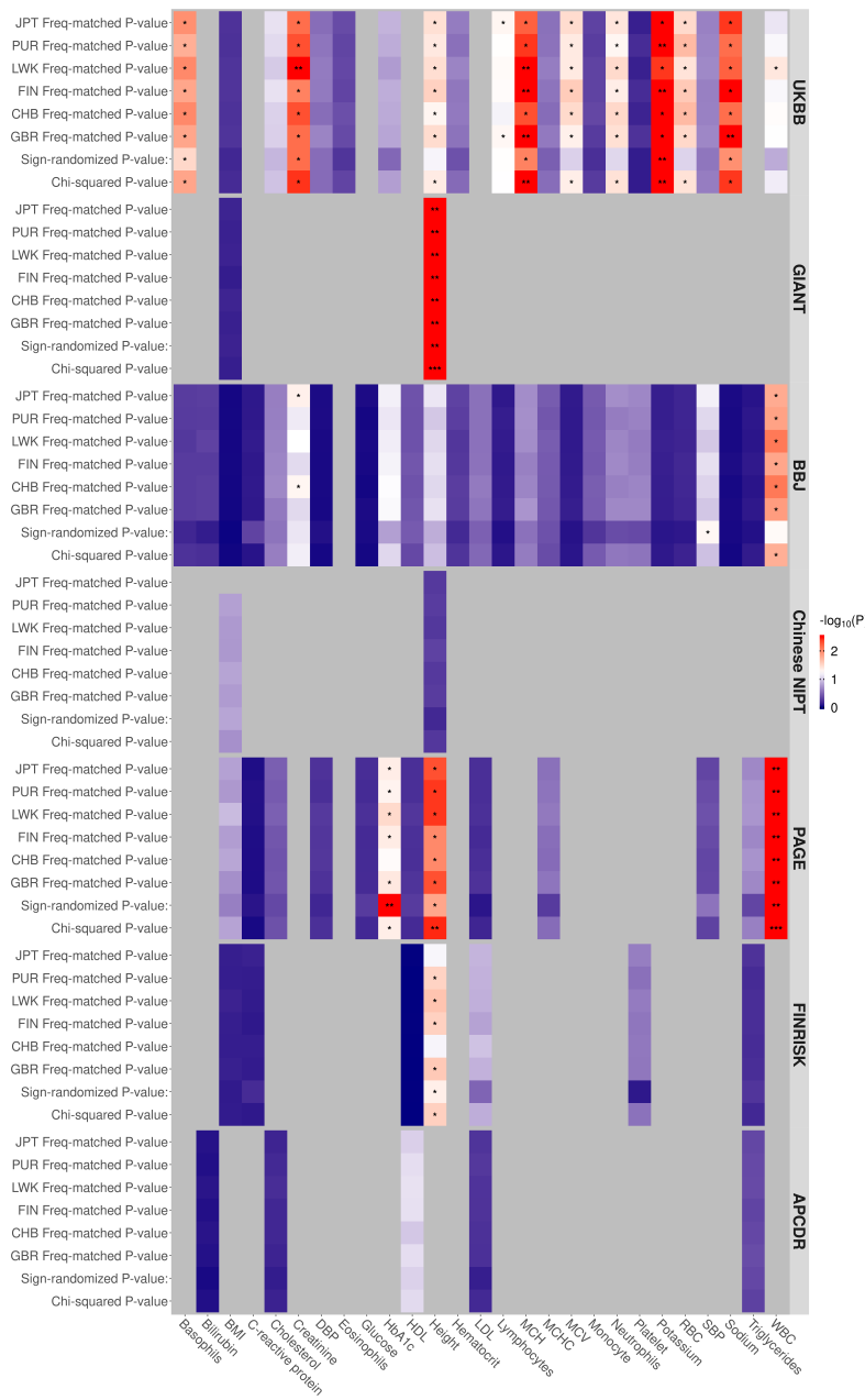
Figure S3: Evidence for polygenic score overdispersion on trait-associated SNPs ( -\log_{10}(P\text{-value}) ), using the Q_X test statistic. Each row in the heatmap corresponds to a specific GWAS cohort and a specific type of scheme to determine the significance of the Q_X statistic. The columns correspond to the different traits for each GWAS cohort that have SNPs with a P-value lower than 5e-8 . "Freq-matched P-value" = P-value obtained by sampling SNPs with matching frequencies to the trait-associated SNPs in a particular cohort. "Sign-randomized P-value" = P-value obtained by randomizing the signs of the effect size estimates. "Chi-squared P-value" = P-value obtained by assuming the Q_X statistics has a chi-squared distribution.
