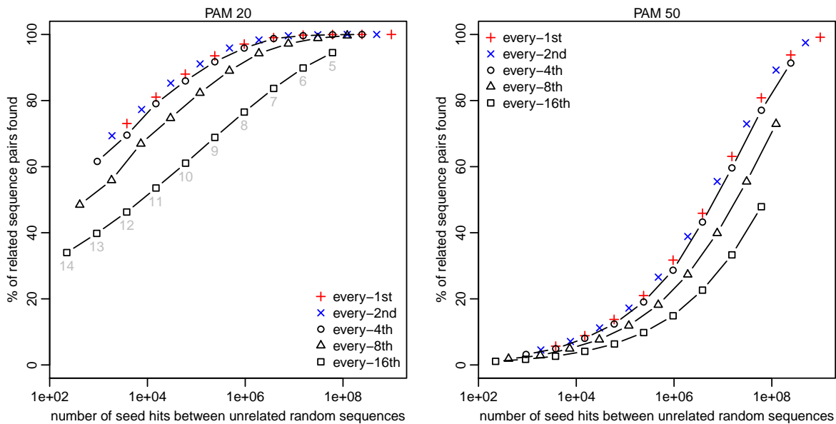
Figure 1: Sensitivity (y-axis) and spurious hit count (x-axis) for exact-match seeds with every- n th sparsity. Seed lengths 5–14 were tested, shown in grey in the left panel.
