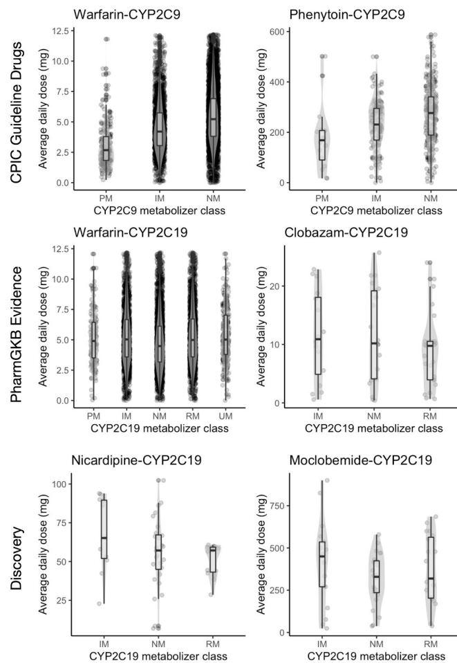
Figure 1. Box plots of maintenance dose for most significant drug-gene pairs. The top two most significant pairs are shown for each group. Enzyme metabolizer classes are represented along the x-axis and the distribution of maintenance dose along the y-axis.
