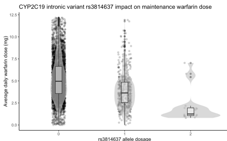
Figure 2. CYP2C19 intronic variant rs3814637 has a strong influence on warfarin maintenance dose. The x-axis indicates the alternate allele dosage (the sum of alternate alleles in each participant). The y-axis is the maintenance dose for each individual.
