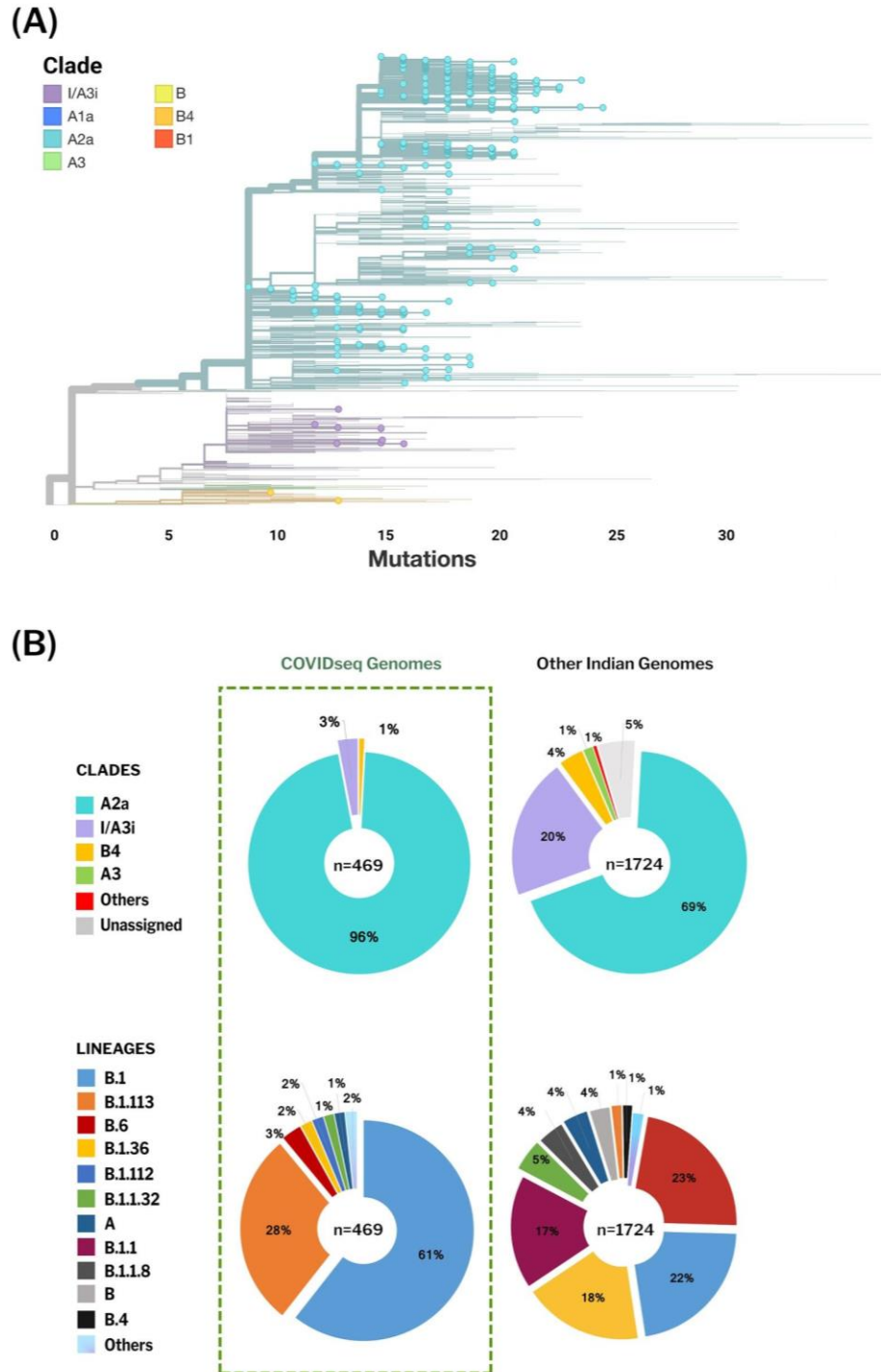
Figure 5. Phylogenetic map of Indian SARS-CoV-2 genomes. 469 genomes reported from this study are highlighted (A) and the proportion of the clades and lineages representing the genomes (B)
