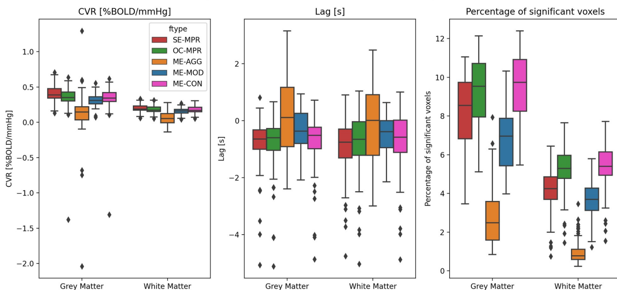
Figure 7: Average values of CVR, lag, and percentage of significant voxels, for voxels in the grey and white matter tissues separately, for all denoising strategies. The dots correspond to a singular session of a singular subject considered an outlier in the distribution. Note that all maps were thresholded before plotting. SE-MPR: single-echo; OC-MPR: optimally combined; ME-AGG: aggressive; ME-MOD: moderate; ME-CON: conservative.
