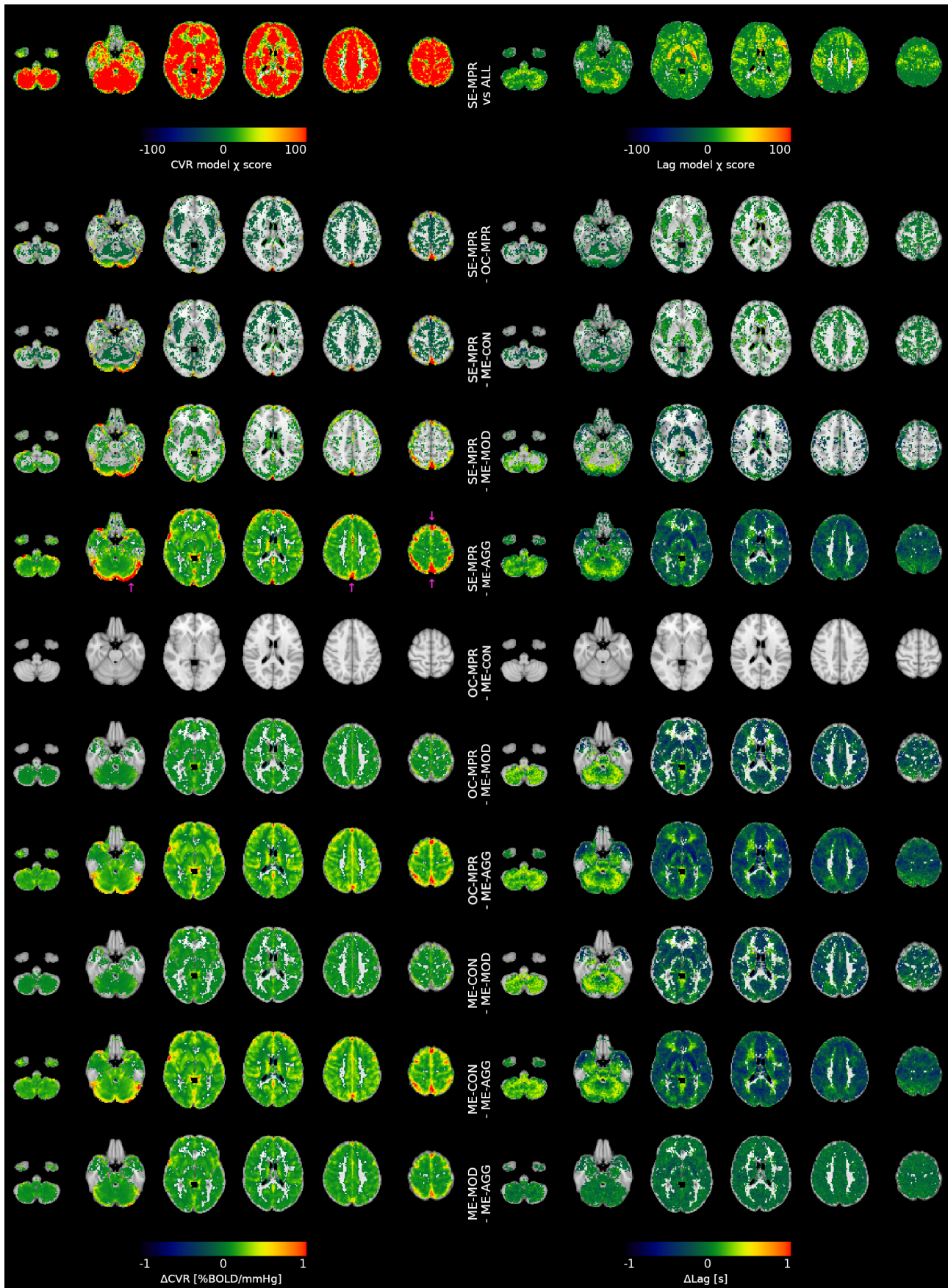
Figure 8: Top row: Thresholded \chi value of the LME model used for the comparison of CVR and lag maps across all denoising strategies. Arrows indicate areas vascularised by big vessels. Other rows: pairwise comparison between denoising strategies. Arrows indicate SE-MPR: single-echo; OC-MPR: optimally combined; ME-AGG: aggressive; ME-MOD: moderate; ME-CON: conservative.
