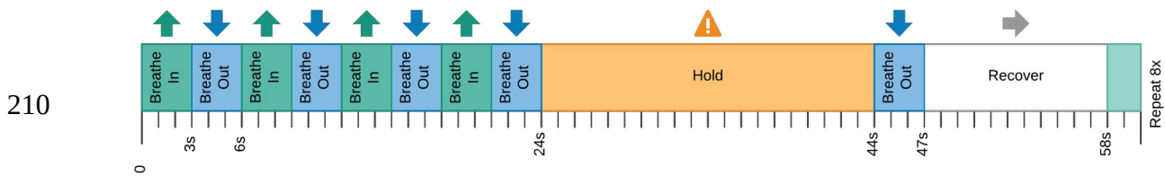
Figure 1: Schematic of Breath-Hold trial. Apnoea was preceded and followed by exhalations.
