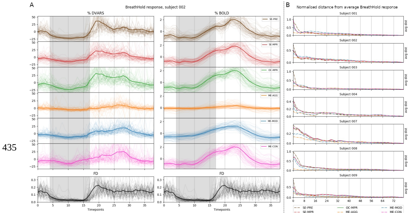
Figure 4: (A) Average GM %DVARS and %BOLD response of all BH trials across ten sessions for the same representative subject. The apnoea period is highlighted in grey. Each transparent line is a trial, the solid line is the average across all the trials. (B) Manhattan distance between the average of N trials and the average of all 80 BH trials as N increases from 1 to 80 for each subject. Each vertical line divides the number of trials in each session. SE-PRE: raw data; SE-MPR: single-echo; OC-MPR: optimally combined; ME-AGG: aggressive; ME-MOD: moderate; ME-CON: conservative. The average %DVARS and %BOLD response of the other subjects can be found in the Supplementary Material (Supplementary figure 2)
