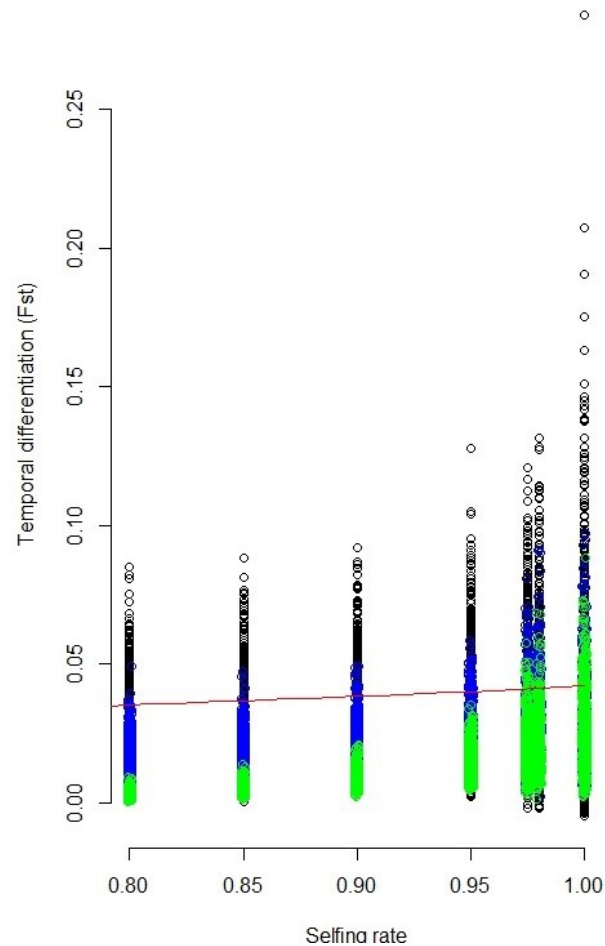
Figure S4. Estimates of temporal differentiation ( F_{ST} ) using all loci and assuming independence (in black) or using the MLG (concatenated genotype) as alleles of a single locus, with (green) or without (blue) exclusion of the MLGs with residual heterozygosity. The red line stands for the expected value for the F_{ST} where F_{ST} = \frac{\tau}{4N^2\sigma + \tau} with \tau the number of generations between the two temporal samples, \sigma the selfing rate and N the simulated population size.
