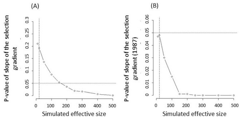
Figure 4. Test of selection for increasing values of N_e . P -value, defined as the proportion of simulated datasets where the slope of the selection gradient is steeper than the observed slope, for the simulations of drift-alone (A) considering all the homozygous MLGs ( n = 48 ) or (B) considering only the MLGs that were already present in 1987 ( n = 12 ). The dotted line indicates the 0.05 threshold value for significance. The vertical dashed line is the effective size estimated using the temporal F_{ST} and considering the 16 microsatellite loci as independent ( N_e = 19 ; p = 0.182 with n = 48 (A); p = 0.047 with n = 12 (B)).
