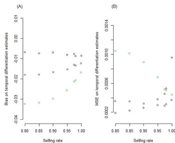
Figure S5. Average bias (A) and MSE (B) for the estimation of temporal differentiation ( F_{ST} ) using all loci and assuming independence (in black) or using the MLG (concatenated genotype) as alleles of a single locus, with (green) or without (blue) exclusion of the MLGs with residual heterozygosity.
