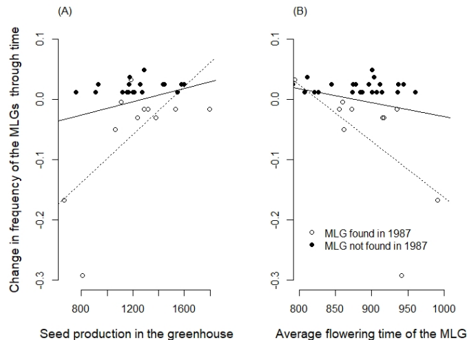
Figure 3. Analyses of the “realised fitness”, estimated as the absolute change in frequency of the MLGs through time. MLGs with residual heterozygosity were removed from this analysis. (A) Relationship with the average number of seeds produced by plants of a given MLG in the greenhouse. (B) Selection gradient for flowering time. Each point stands for the average flowering date for a given MLG. The black regression lines are estimated using all points ( n = 48 ; A: slope = 5.10^{-5} points of frequency per seed p = 0.094 ; B: slope = -0.0002 95% confidence interval: -0.0006; 0.0001 p = 0.179 ). This includes MLGs that were not observed in 1987 (black dots), for which the change in frequency is necessarily always positive. The dotted lines are the regression lines for the analysis restricted to the MLGs present in 1987 (white dots only; n = 12 ; A: slope = 0.0002 p = 0.024 ; B: slope = -0.0009 95% confidence interval: -0.0017; -0.0002 p = 0.038 ). Q-Q plots for the selection gradients are provided in Fig. S3.
