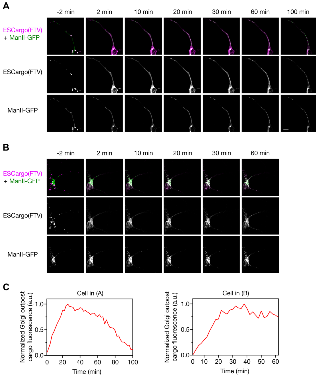
FIGURE 3: Traffic of ESCargo(FTV) in rat cortical neurons. Isolated neurons were cultured for 15 days in vitro , and were transfected with constructs encoding ManII-GFP and ESCargo(FTV) 48 h before imaging. SLF was added at time zero to a final concentration of 50 \mu\text{M} . For each of two representative cells, the top row shows the merged images while the other two rows show the red and green channels. Average projected Z-stacks were taken from the second part of Supplemental Movie S2. (A) Example of a neuron with a long tubular extension from the somatic Golgi into a dendrite. Two Golgi outposts were initially visible, and the tubule progressively fragmented to create additional Golgi outposts. Scale bar, 10 \mu\text{m} . (B) Example of a neuron that initially contained multiple punctate Golgi outposts. Scale bar, 10 \mu\text{m} . (C) Quantification of Golgi outpost-associated cargo fluorescence in the cells in (A) and (B). The ManII-GFP
