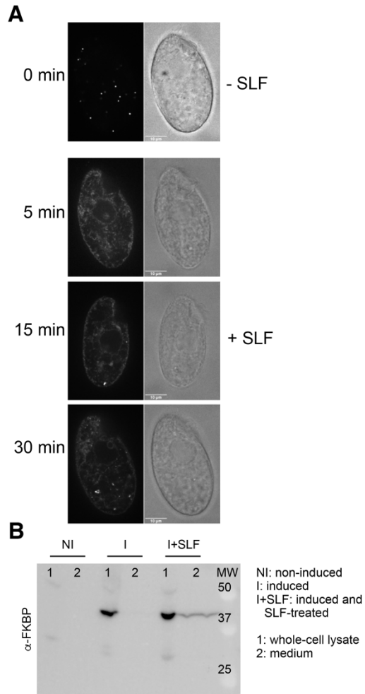
FIGURE 5: Traffic of ESCargo* in Tetrahymena thermophila . (A) Confocal cross sections of fixed Tetrahymena cells expressing ER-targeted ESCargo*, with paired differential interference contrast images. Protein expression was induced with CdCl 2 prior to addition of 12.5 \mu M SLF. The top panel shows cells fixed immediately after SLF addition (0 min), and the other panels show cells fixed after treatment with SLF for 5, 15, or 30 min. The fluorescence exposure times were 100 ms for the 0 min image or 400 ms for the other images. Bright fluorescent puncta were visible initially but disappeared within 5 min after SLF addition, resulting in dispersed fluorescence in ER-like membranes that included the nuclear envelope. By 30 min, some punctate fluorescence had reappeared. Scale bars, 10 \mu m. (B) Immunoblot analysis of ESCargo* secretion. Tetrahymena cells expressing ESCargo* were treated with 12.5 \mu M SLF for 5 min. After centrifugation, TCA-precipitated cell pellet and cell-free culture medium samples were analyzed by SDS-PAGE and immunoblotting with anti-FKBP antibody. The cargo protein was detected in whole cell lysates for induced untreated and induced SLF-treated cells, and in the medium only for induced SLF-treated cells. No cargo protein was detected in non-induced cells.
