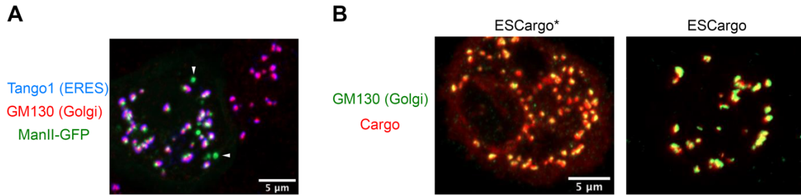
FIGURE S1: Golgi labeling in Drosophila S2 cells. (A) Incomplete colocalization of ManII-GFP puncta with Golgi and ER exit site (ERES) compartments. S2 cells expressing ManII-GFP were fixed and immunostained for GM130 (Golgi marker) and Tango1 (ERES marker). A subset of the ManII-GFP puncta did not have associated GM130 or Tango1 signal. Two examples are marked with arrowheads. Scale bar, 5 μm. (B) Accumulation of secretory cargo in all Golgi stacks. S2 cells expressing ESCargo* or ESCargo were treated with 50 μM SLF for 5 min, fixed, and immunostained for GM130 (Golgi marker). All of the GM130 puncta had cargo signal. Scale bar, 5 μm.
