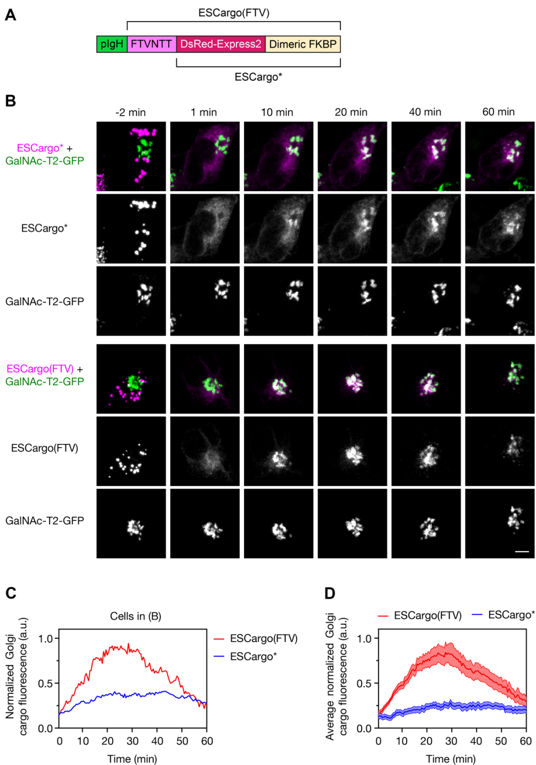
FIGURE 2: Traffic of ESCargo variants in cultured mammalian cells. (A) Functional segments of the ESCargo(FTV) and ESCargo* constructs. pIgH (green): mammalian ER signal sequence. FTVNTT (pink): tripeptide ER export signal followed by tripeptide N -linked glycosylation signal. For further details, see
