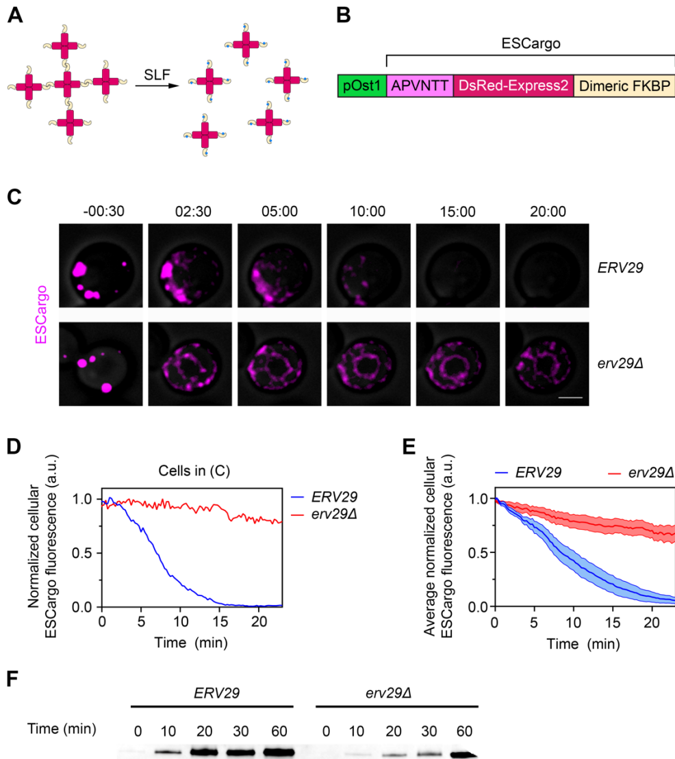
FIGURE 1: ESCargo as a tool for monitoring secretion in Saccharomyces cerevisiae . (A) Strategy for generating and dissolving fluorescent aggregates. DsRed-Express2 tetramers (red) fused to a dimeric variant of FKBP (gold) associate to form aggregates. Addition of the FKBP ligand SLF (blue) blocks dimerization, thereby dissolving the aggregates into soluble tetramers. (B) Functional segments of the ESCargo construct. pOst1 (green): ER signal sequence that directs cotranslational translocation in yeast. APVNTT (pink): tripeptide ER export signal followed by tripeptide N -linked glycosylation signal. DsRed-Express2 (red): tetrameric red fluorescent protein. Dimeric FKBP (gold): reversibly dimerizing FKBP RD (C22V) variant. The lengths of the segments are not to scale. (C) Secretion of ESCargo in yeast cells containing or lacking Erv29. ERV29 wild-type and erv29Δ strains expressing ESCargo were grown overnight to mid-log phase and then imaged by confocal and brightfield microscopy. SLF was added at time zero to a final concentration of 100 μM. Average projected Z-stacks are taken from Supplemental Movie S1. Scale bar, 2 μm. (D) Quantification of the intracellular ESCargo fluorescence from the cells in (C). At each time point, the brightfield image was used to select the cell profile and quantify the total ESCargo fluorescence.
