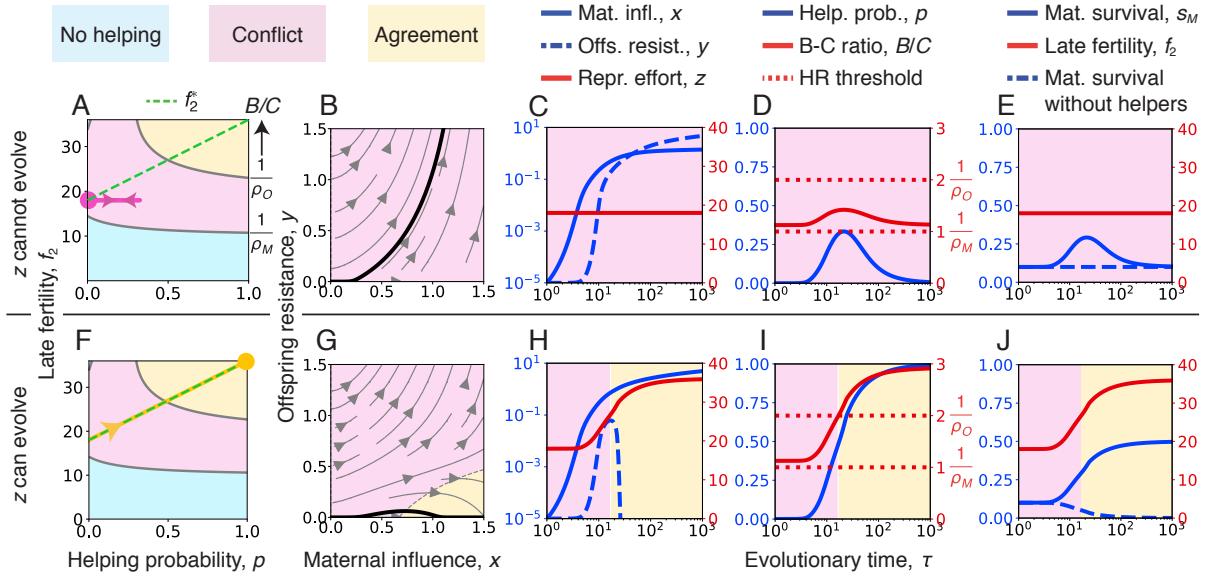
Figure 2: Conflict dissolution via maternal reproductive specialization (evolutionary model). (A-E) Co-evolution of maternal influence x and offspring resistance y when maternal reproductive effort z —and hence late fertility f_2 —cannot evolve (i.e., the genetic variance of z , G_z , is zero). (A) Phase portrait showing the evolution of the helping probability p under constant late fertility f_2 . Starting from conflict, helping evolves temporarily but is eventually lost due to the evolution of resistance (start and end points are given by the circle ; the pink trajectory ends in the conflict zone). (B) Stream plot showing the co-evolution of maternal influence and offspring resistance. The black line shows the trajectory for the initial conditions used. (C-E) Time series of: (C) the evolving traits; (D) the resulting helping probability p , benefit-cost ratio B/C , and the Hamilton's rule (HR) threshold from the mother and offspring perspective; and (E) the vital rates s_M , f_2 , and s_M with zero helpers. (F-J) Analogous plots but now z can evolve as the mother chooses it optimally for the number of helpers she has (i.e., as if G_z \rightarrow \infty ). In this case, fertility evolves along the optimal path, f_2^* . (F) Phase portrait showing the co-evolution of the helping probability p and optimal late fertility f_2^* . Starting from conflict, helping emerges and is maintained through the evolution of z yielding agreement (end point is given by the circle ; the yellow trajectory ends in the agreement zone). (G) Stream plot showing the co-evolution of maternal influence and offspring resistance. The black line shows the trajectory for the initial conditions used; such a trajectory starts at conflict but converges to agreement. (H) Resistance reversal. (I) B/C evolves and the Hamilton's rule threshold from the offspring perspective is crossed. (J) The mother becomes highly fertile and reliant on helpers for her own survival. The genetic system is diploid, both sexes help, and helping is under shared control with sequential determination of the joint helping phenotype. Here, the life-history trade-off is between maternal survival s_M and late fertility f_2 , as illustrated in Fig. 3. Second-brood offspring survival s_2 is constant. The remaining details of the functional forms and parameter values used are given in SI Appendix, section 8.
