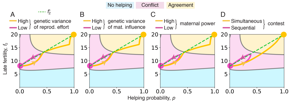
Figure 4: Promoters of conflict dissolution. Resistance wins (trajectory ending at the pink circle ) or conflict dissolution occurs (trajectory ending at yellow circle ), respectively for (A) low or high genetic variance of reproductive effort, (B) low or high genetic variance of maternal influence, (C) low or high maternal power, and (D) sequential or simultaneous determination of the joint helping phenotype. The genetic system is diploid and both sexes help. Functional forms and parameter values are as in Fig. 2 except as follows. For A, G_z = 225 for low genetic variance of z and G_z = 250 for high genetic variance of z . For B, G_x = 0.9 for low genetic variance of x and G_x = 1 for high genetic variance of x (and G_z = 250 for both). For C, \chi = 0.9 for low maternal power and \chi = 1 for high maternal power (and G_z = 250 for both). For D, sequential contest and simultaneous contest (and G_z = 225 for both). A very high genetic variance of z is used here for visualization, but is not necessary for conflict dissolution (cf. SI Appendix, Fig. S14).
