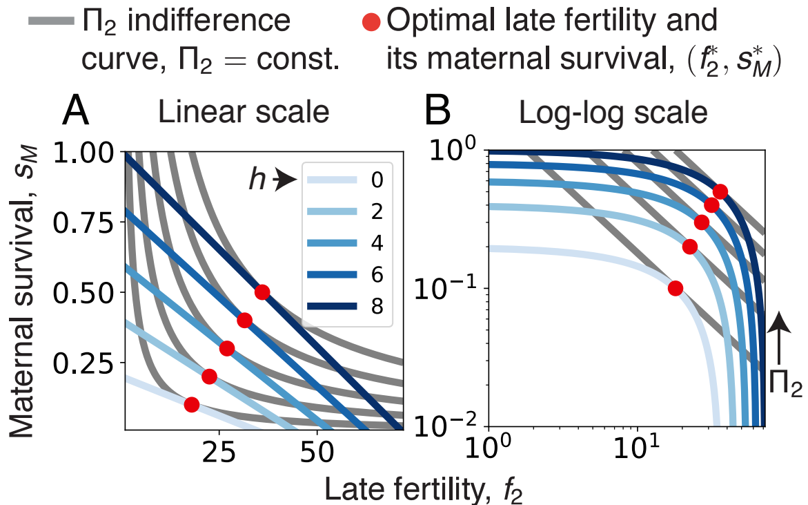
Figure 3: Survival-fertility trade-off alleviation by helpers. Here, maternal survival s_M decreases with late fertility f_2 due to the assumed trade-off (blue lines; linear trade-off in (A) linear scale or (B) log-log scale) whereas second-brood survival s_2 is constant. For a given number of helpers h , an optimal late fertility f_2^* (red dots) occurs when a s_M curve has the same slope as a \Pi_2 indifference curve (gray lines, where late productivity \Pi_2 is constant). In log-log-scale, all \Pi_2 indifference curves have the same slope, namely -1 , as \partial\Pi_2/\partial f_2 = 0 is equivalent to \epsilon_{f_2}(s_M) + \epsilon_{f_2}(s_2) = -1 (see SI Appendix, section 5). Since here, \epsilon_{f_2}(s_2) = 0 , the alleviation condition states that (in log-log scale) the slope of s_M with respect to f_2 increases with increasing h at an optimal f_2^* . Equivalently, the alleviation condition states that f_2^* increases with h (red dots move to the right as h increases). Functional forms and parameter values are as in Fig. 2.
