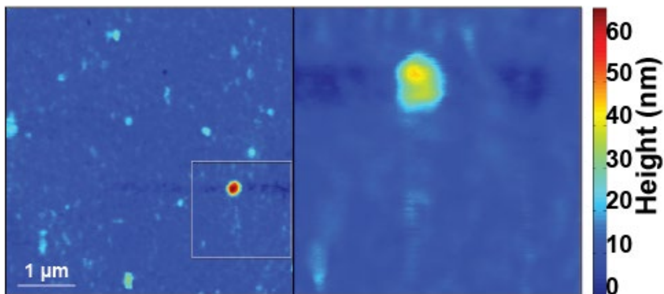
Fig. 2 Sars-CoV-2 VLP disintegrates readily when AFM scanned at 34 C. Surface features consistent with individual VLPs are extremely rare. Even when such features are found in large area surveys (left), they cannot be scanned a second time, e.g. to obtain a zoomed in view (right). Zoom are is highlight on the left via a rectangle outline. The particles become flatter and show lateral spread consistent with mechanical VLP destruction [10].
