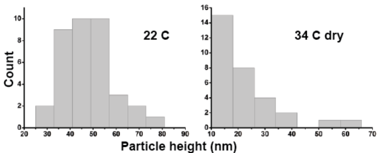
Fig 3. Temperature dependence of Z-height distributions of surface features. (A) Surface features have a strongly peaked height distribution consistent with air dried VLPs at 22°C. The median height of the particles is 43.4-51.4 nm (n=37). (B) Features observed at 34°C have median height 14.6-22.3 nm (n=31). CI estimated via bootstrap with 1e3 resamplings.
