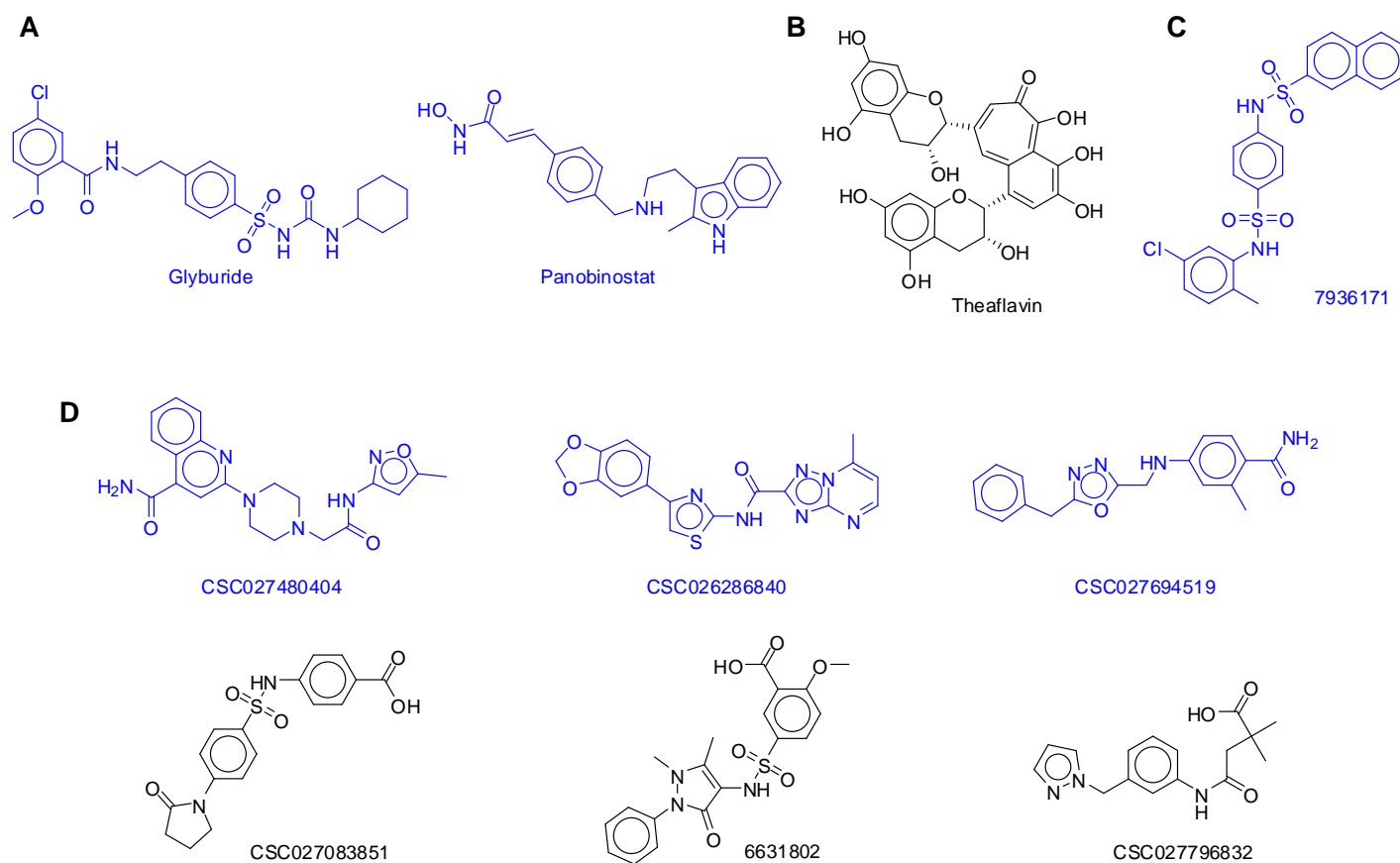
Figure 2. Chemical structures of ten compounds from different sources experimentally tested. Compounds are grouped by their source A ) approved drugs; B ) dietary source (natural product); C ) Inhibitor of the viral NS5 RNA methyltransferase; D ) DNMT focused library.
