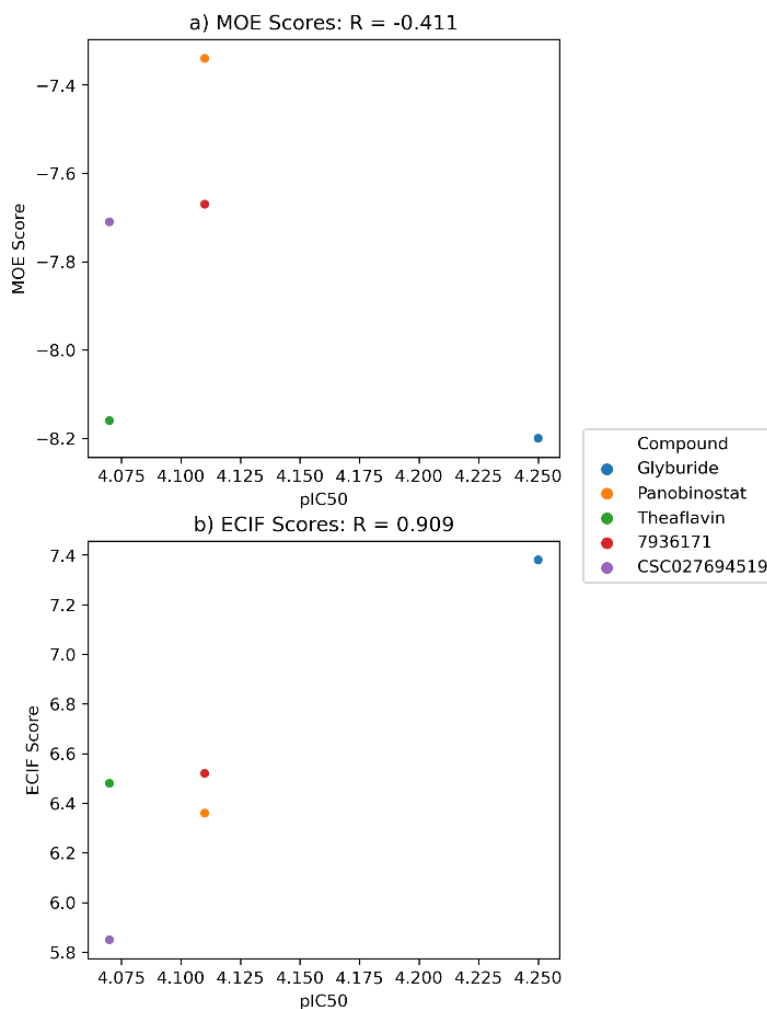
Figure 4. Correlation between the experimental pIC 50 of the five compounds evaluated in biochemical inhibition assays of DNMT1 with A) the docking scores calculated with MOE, and B) the ECIF6::LD-GBT scores.
