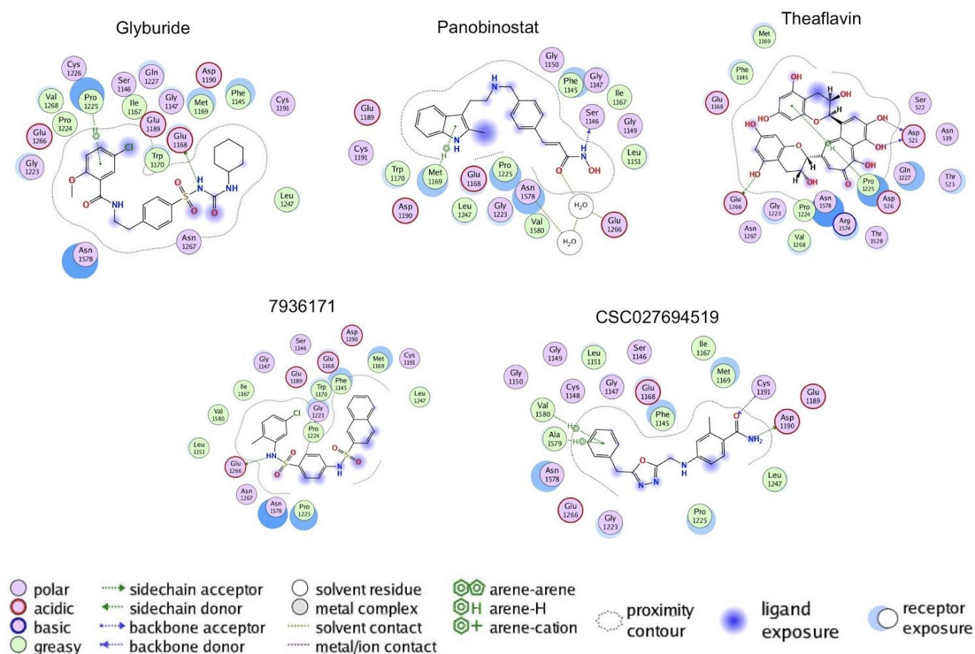
Figure 3. Binding poses predicted with the Molecular with Molecular Operating Environment v.2018 of the five active compounds with the catalytic domain of DNA methyltransferase 1.
