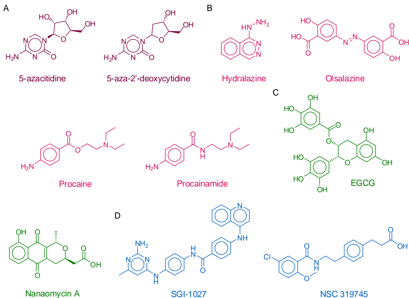
Figure 1. Chemical structures of representative DNMT inhibitors and other compounds with associated hypomethylating properties, from different sources. A) approved drugs; B) drug repurposing; C) Natural products and dietary components; D) Small molecules: synthetic compounds.
