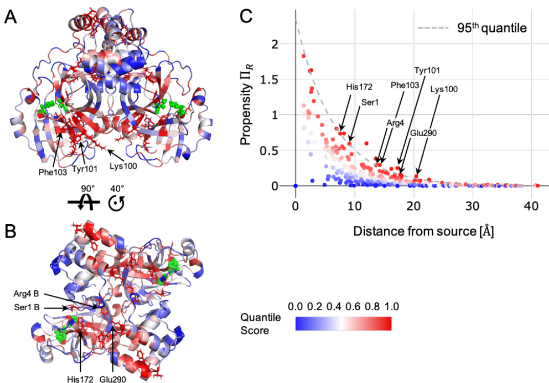
Figure 1: Bond-to-bond propensities of M^{Pro} sourced from the orthosteric sites. The source sites have been chosen as the catalytically active residues His41 and Cys145 in both chains of the homodimer and are shown in green (front A) and top B) view). All other residues are coloured by quantile score as shown in the legend and reveal two main areas of interest with important residues labelled. C) The propensity of each residue, \Pi_R , is plotted against the residue distance from the orthosteric site. The dashed line indicates the quantile regression estimate of the 0.95 quantile cutoff used for identifying relevant residues.
