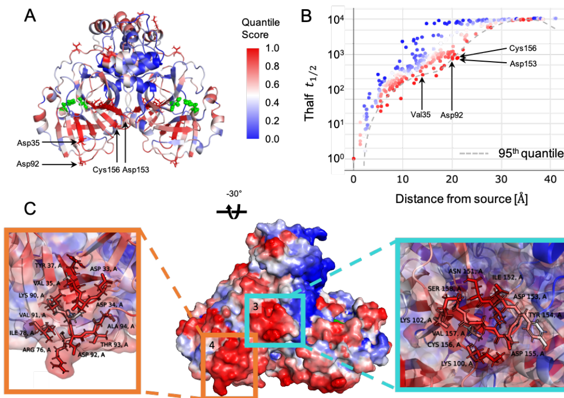
Figure 3: Markov transient analysis of M PrO sourced from the orthosteric sites. The orthosteric sites are shown in green and include His41 and Cys145 in both chains of the homodimer (front A) view. B) The t_{1/2} values of each residue are plotted against their distance from the orthosteric site. The dashed line indicates the quantile regression estimate of the 0.95 quantile cutoff used for identifying significant residues. The quantile scores of all residues are mapped onto the surface of the M PrO dimer (front A) view), coloured as shown in the legend. C) Surface representation of a rotated front view the M PrO dimer coloured by quantile score. Site 3 (turquoise) and 4 (orange) are located on the opposite site of the active site (coloured in green). A detailed view of both sites is provided with important residues labelled.
