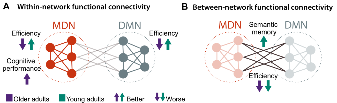
Figure 8. The different effects of within- and between network functional connectivity on task performance in each age group. (A) Young adults improved their efficiency in the form of faster response times whereas older adults performed slower when functional connectivity within the MDN or DMN increased. Moreover, strengthened connectivity within the MDN was related to a better performance in executive measures for older adults. (B) Strengthened between-network functional connectivity led to a decline in efficiency in both age groups. However, it was also associated with an improved performance in semantic memory only for young adults. Abbrev.: MDN Multiple-demand network; DMN Default mode network.
