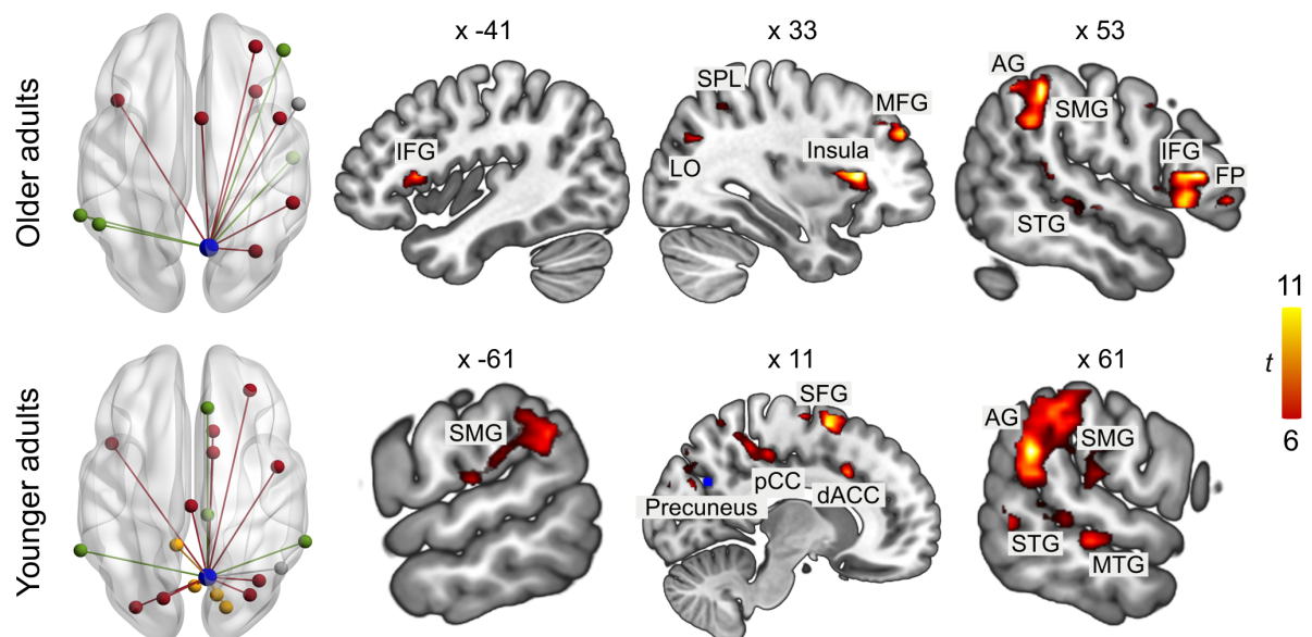
Figure 6. Functional connectivity for seeds from contrast Counting > Semantic fluency. All results are FWE-corrected at p < 0.05 at peak level with a minimum cluster size = 20 voxel. Abbreviations: IFG inferior frontal gyrus; TP temporal pole; SFG superior frontal gyrus; SMG supramarginal gyrus; LO lateral occipital cortex; SPL superior parietal lobe; MFG middle frontal gyrus; AG angular gyrus; FP frontal pole; STG superior temporal gyrus; pCC posterior cingulate cortex; dACC dorsal anterior cingulate cortex; MTG middle temporal gyrus. Unthresholded statistical maps are available at https://neurovault.org/collections/9072/ .
