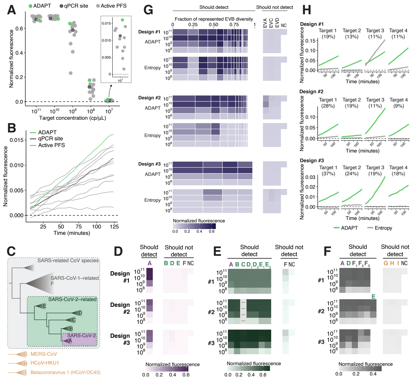
Figure 4 — Experimental evaluation of designs. (a) Fluorescence at varying target concentrations in the US CDC's SARS-CoV-2 N1 qPCR amplicon. Compared Cas13a guides are from our approach using ADAPT (green); a guide with an active (non-G) PFS at the site of the qPCR probe (dark gray); and 10 randomly selected guides with an active PFS (light gray). All were constrained to the amplicon. (b) Fluorescence over time for guides from (a) at target concentration of 10 7 cp/μL. (a) shows final time point (124 minutes). (c) Phylogeny within SARS-related CoV species based on ref. 43, and 3 related betacoronaviruses. (d) Fluorescence for ADAPT's top-ranked SARS-CoV-2 designs in detecting representative targets of the clades in (c). Rankings reflect ADAPT's predicted performance. Left label indicates target concentration (cp/μL). NC, no template control. In (d–f), colors refer to (c). (e) Same as (d), but for SARS-CoV-2-related taxon. Empty column with dashes indicates sequence in the design's amplicon has high ambiguity and was not tested. Clades D and E sometimes have two representative targets in these amplicons; when two target labels were tested with one representative sequence, the same value is plotted for each. (f) Same as (d), but for SARS-related CoV species. Clade F 1 is SARS-CoV-1, and F 2 and F 3 are related bat SARS-like CoVs. E requires a separate representative target in only one amplicon. G, H, and I are defined in (c). (g) Fluorescence for ADAPT's top-ranked EVB designs in detecting EVB and representative targets for Enterovirus A/C/D (EVA/C/D). Each band is an EVB target having width proportional to the fraction of EVB genomic diversity represented, within the amplicon of ADAPT's design. Under each ADAPT design is a baseline guide ("Entropy") from the site in the amplicon with an active PFS and minimal entropy. (h) Fluorescence over time at target concentration of 10 8 cp/μL, for the 4 EVB targets representing the largest fraction of EVB genomic diversity. (g) shows middle time point (59 minutes). In all panels, fluorescence is reference-normalized and background-subtracted (Methods).
