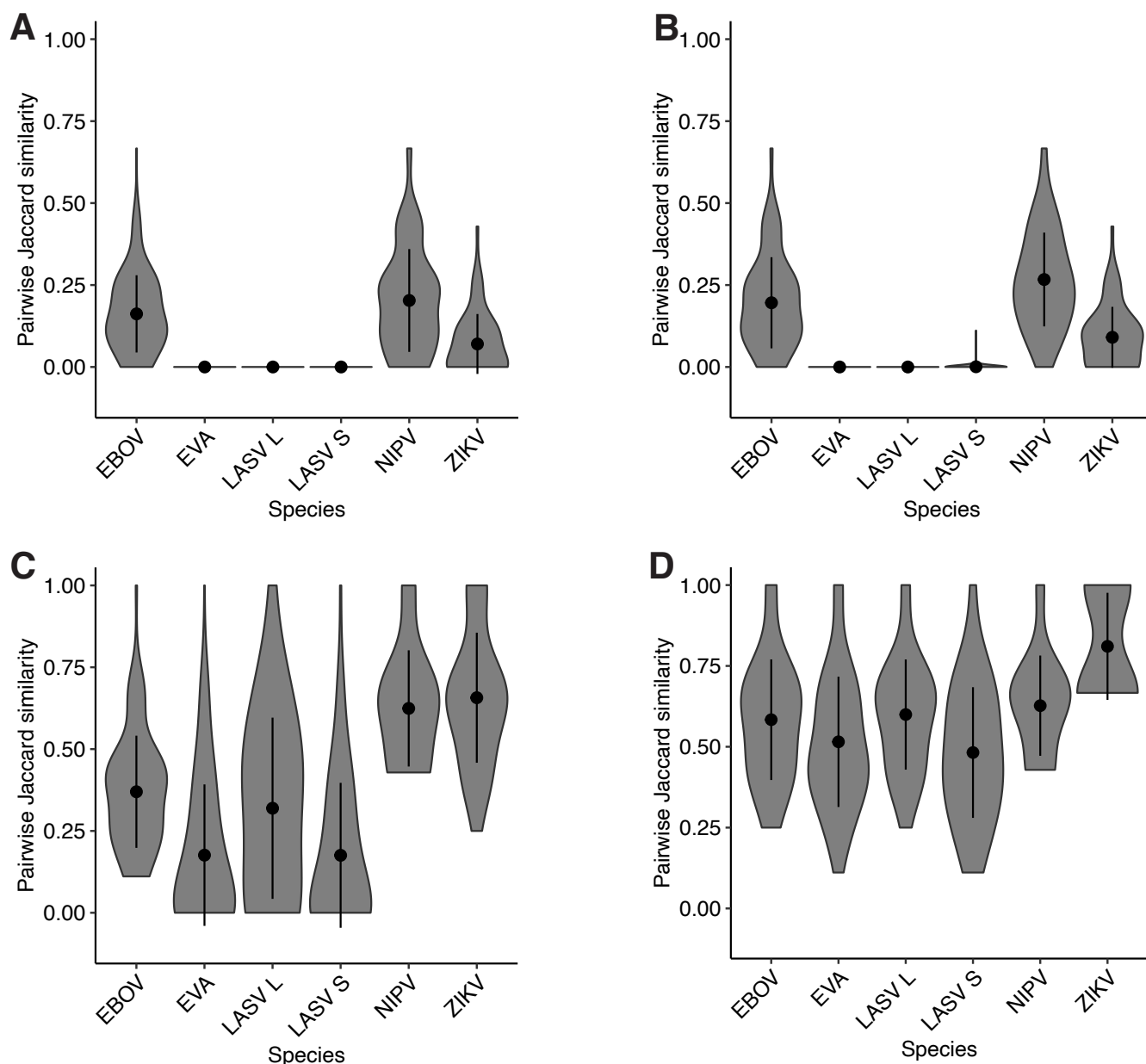
Supplementary Figure 23 — Dispersion in ADAPT's designs. For each species, we ran ADAPT 20 times. For each pair of runs, we calculated the Jaccard similarity comparing the top 5 design options from each. Violin plots show a smoothed density estimate of the pairwise Jaccard similarities; dot indicates the mean and bars show 1 standard deviation around the mean. (a) Using resampled input genomes for each run and considering two design options to be equal if they have exactly the same primers and probes. (b) Using the same input genomes for each run and considering two design options to be equal if they have exactly the same primers and probes. (c) Using resampled input genomes for each run and considering two design options to be equal if their endpoints are within 40 nt of each other. (d) Using the same input genomes for each run and considering two design options to be equal if their endpoints are within 40 nt of each other. When using resampled input genomes, the comparisons account for algorithmic randomness and input sampling. When using the same input genomes, the comparisons account only for algorithmic randomness. EBOV, Zaire ebolavirus; EVA, Enterovirus A; LASV L/S, Lassa virus segment L/S; NIPV, Nipah virus; ZIKV, Zika virus.
