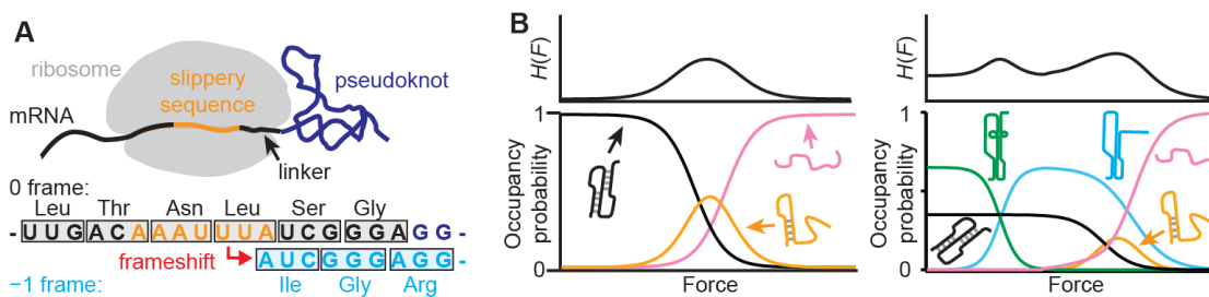
Figure 1: -1 PRF and conformational Shannon entropy. (A) -1 PRF is stimulated by a structure in the mRNA (here, a pseudoknot) just downstream of a slippery sequence, leading to a shift in the ribosome reading frame. (B) The Shannon entropy of the stimulatory structure as a function of force on the mRNA is illustrated notionally for a simple case where a pseudoknot unfolds via an intermediate (left) and a more complex case where multiple structures can be formed (right).
