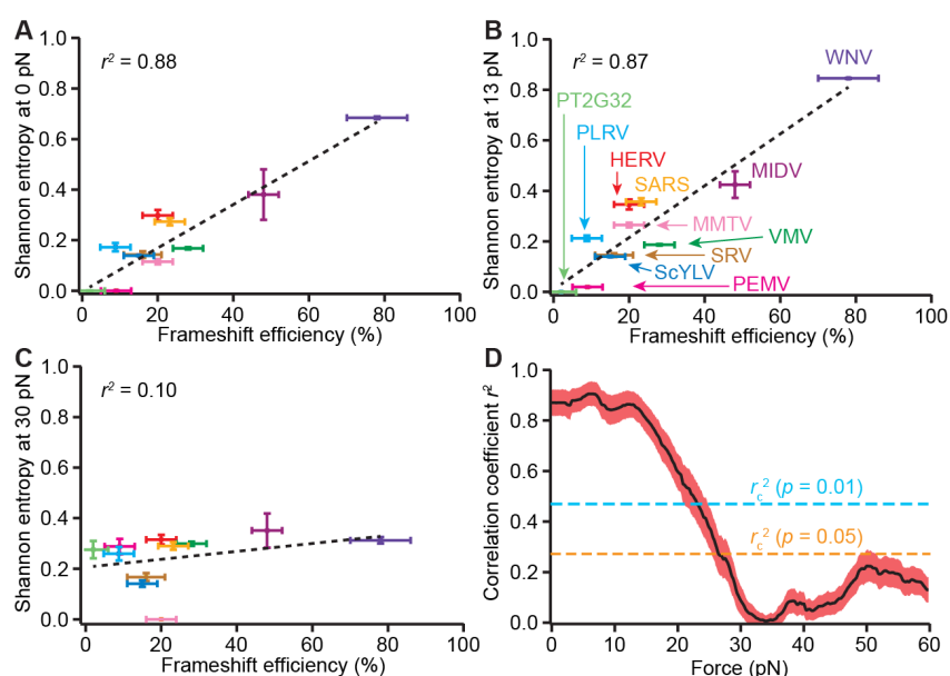
Figure 3: Correlation between Shannon entropy and -1 PRF efficiency for wild-type stimulatory structures. (A-C) Shannon entropy and -1 PRF efficiency vary linearly at low force (A: 0 pN, B: 13 pN) but are poorly correlated at high force (C: 30 pN) for the whole panel of wild-type stimulatory structures. (D) The Pearson correlation coefficient is strongly force-dependent, with the correlation vanishing above \sim 20 pN, which is higher than the maximum force applied by the ribosome during translation ( \sim 13 pN). Dashed lines show critical r^2 value (cyan: 99% confidence level, orange: 95% confidence level), shaded region shows standard error in r^2 .
