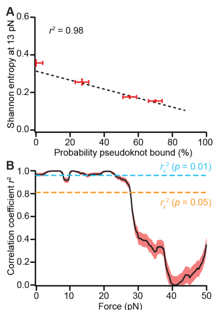
Figure 5: Correlation for pseudoknot bound with anti-frameshifting ligand. (A) Shannon entropy at 13 pN varies linearly with the fraction of SARS-CoV pseudoknot bound by a -1 PRF-inhibiting ligand. (B) The Pearson correlation vanishes above the maximum biologically relevant force. Dashed lines shows critical r^2 values at 99% (cyan) and 95% (orange) confidence levels, shaded region shows standard error in r^2 .
