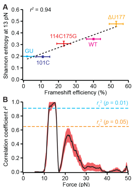
Figure 4: Correlation for mutant pseudoknots (color online). (A) Shannon entropy and -1 PRF efficiency vary linearly at 13 pN for mutants of the human telomerase pseudoknot. (B) The Pearson correlation again vanishes above the maximum biologically relevant force. Dashed lines show critical r^2 values at 99% (cyan) and 95% (orange) confidence levels, shaded region shows standard error in r^2 .
