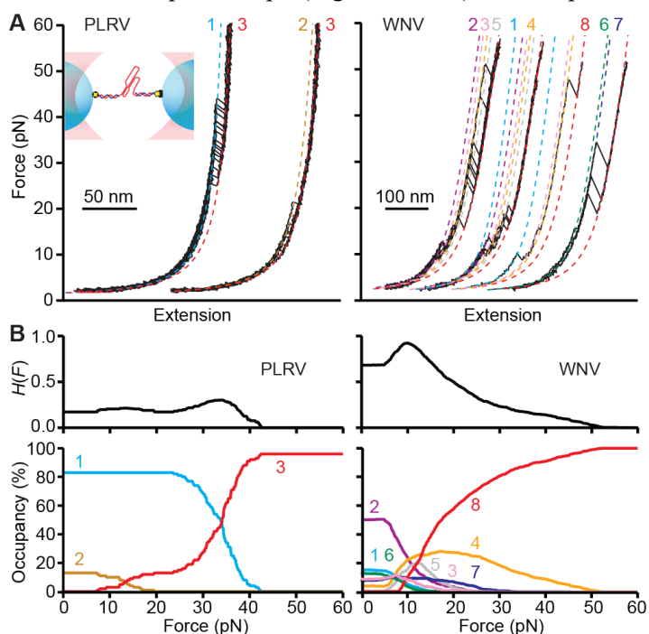
Figure 2: Force spectroscopy measurements of frameshift stimulatory structures. (A) Sample force extension curves of the stimulatory structures from PLRV (left) and WNV (right). For PLRV, 3 different states are seen (as numbered), whereas for WNV, 8 are seen. Sets of curves containing different states are offset for clarity. The states seen in stimulatory structures from different viruses are generally unrelated. Inset: schematic of measurement showing RNA connected by double-stranded handles to beads held in optical traps. (B) Fractional occupancy of each state as a function of force (lower panels) and force-dependent conformational Shannon entropy (upper panels) for PLRV (left) and WNV (right).
