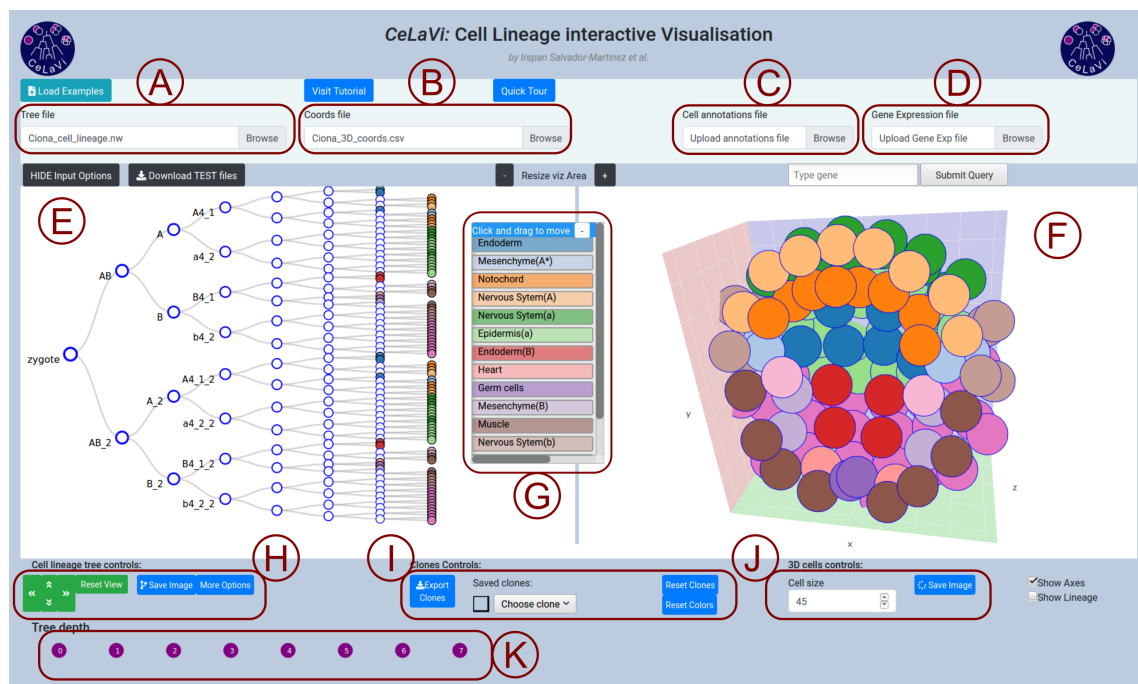
Fig. 1. The CeLaVi user interface, loaded with the Ciona gastrula dataset. The main areas of the interface are labelled: A) tree file input; B) cell coordinates file input; C) cell annotations file input; D) gene expression file input; E) lineage viewer; F) 3D viewer; G) cell annotations table; H) cell lineage tree controls; I) clones controls; J) 3D cells controls; K) tree depth area. Cells show cell fates with a colour code based on the cell annotations table. For more details visit the tutorial ( http://www.celavi.pro/tutorial.html ).
