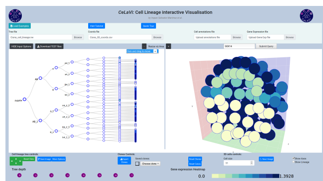
Fig. 2. Ciona gastrula example dataset showing the expression pattern of gene Sox14 as a heatmap (colour code below the 3D viewer area).
