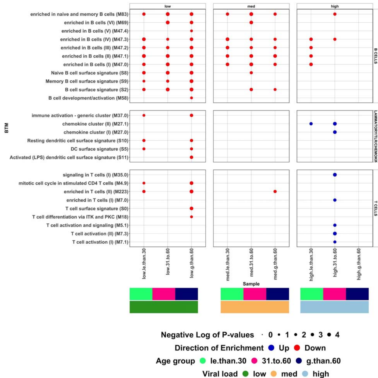
Figure 5. Plot showing -\log_{10}(\text{p-values}) of differentially enriched B cell, inflammatory/TLR/Chemokine and T cell modules (y-axis) of the surveillance data (Lieberman et al. 2020) stratified by age and viral load. The size of the circles corresponds to the magnitude of the -\log_{10}(\text{p-value}) , while their colour corresponds to the direction of enrichment as indicated by the MROAST function of ROAST R package (see key).
