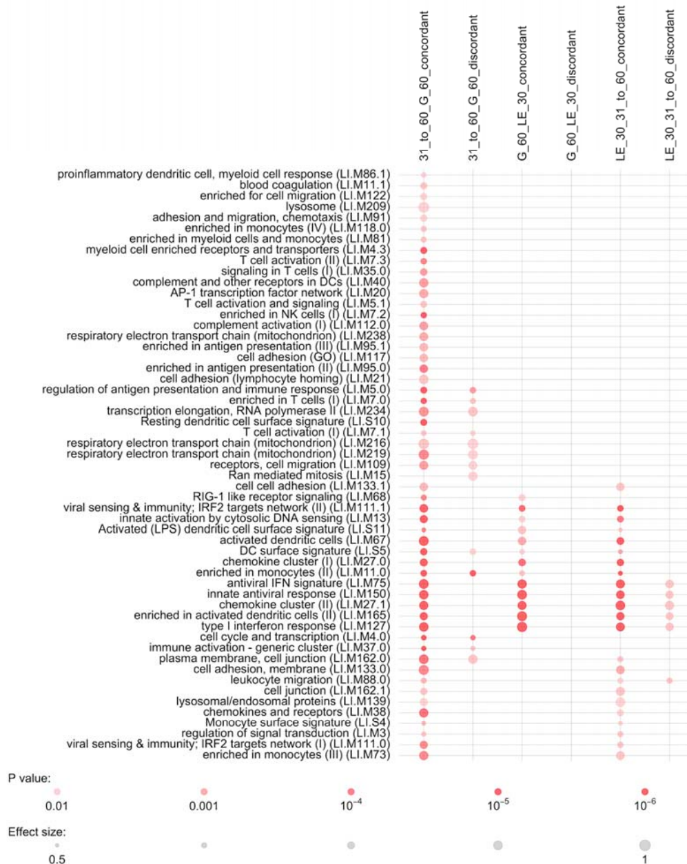
Figure 11. Dotplot of p-values of concordant and discordantly enriched modules identified by the tmod package in R, based on the disco score of the differential co-expressed member genes of WGCNA modules.
