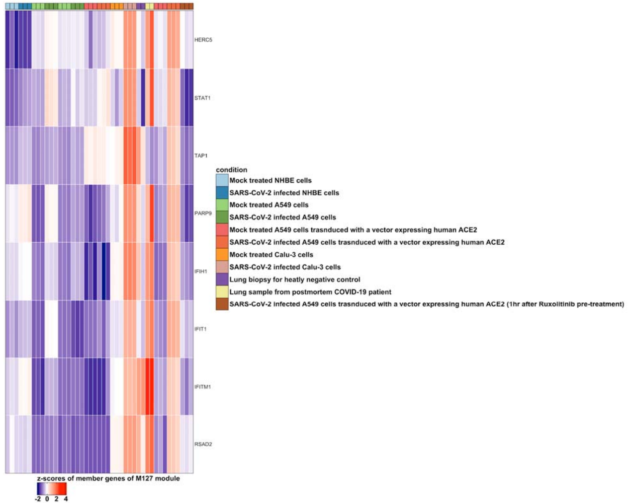
Supplementary figure 5. Heatmap of the scaled expression values of the member genes of the type I interferon module (M127) of lung biopsy and cell line samples, generated using ComplexHeatmap ( Gu et al. 2016 ).
