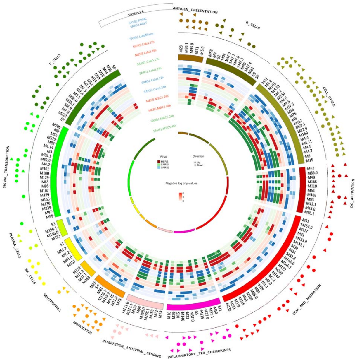
Figure 13. Circos plot showing enrichment of modules in SARS-CoV-2 clinical samples and SARS-CoV-2, SARS-CoV-1 and MERS-CoV infected cell lines. Each circle represents the negative log of p-values of enriched modules in each sample, coloured by virus (see 'samples' legend at 11 o'clock). The 3 outer circles represent the direction of enrichment of modules of the clinical samples of SARS-CoV-2 (PBMC, BALF and lung samples) as predicted by the MROAST function of ROAST R package; a circle indicates down-regulation, while an arrow indicates up-regulation of the module.
