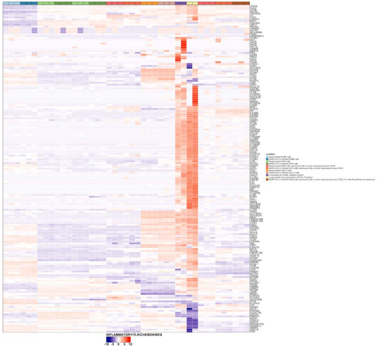
Supplementary figure 1. Heatmap of the scaled expression values of the member genes of the modules belonging to the Inflammatory/TLR/Chemokine group of Lung biopsy and cell line samples, generated using ComplexHeatmap ( Gu et al. 2016 ).
