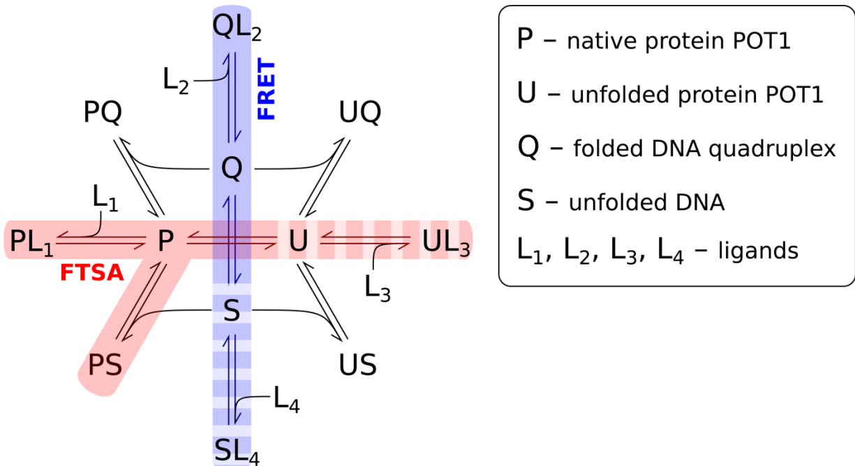
Scheme I. POT1 (P) binding equilibria and possible inhibition pathways. U is unfolded POT1, Q represents folded G4 structures, S is unfolded (or single-stranded) G4 structures and L is a small molecule binding ligand. By using different detection probes, FTSA can monitor the fate of different reactants. Sypro Orange allows POT1 to be monitored, while the G4 is “invisible”. Conversely, a FRET-labeled G4 allows the G-quadruplex to be monitored, while POT1 is “invisible”. Sypro Orange would be sensitive to POT1 denaturation, to stabilization by interactions with ssDNA or small molecule ligands, and FRET labeled G4 would directly sense G-quadruplex unfolding and stabilizing interactions arising from ligand binding or destabilizing interactions with POT1
