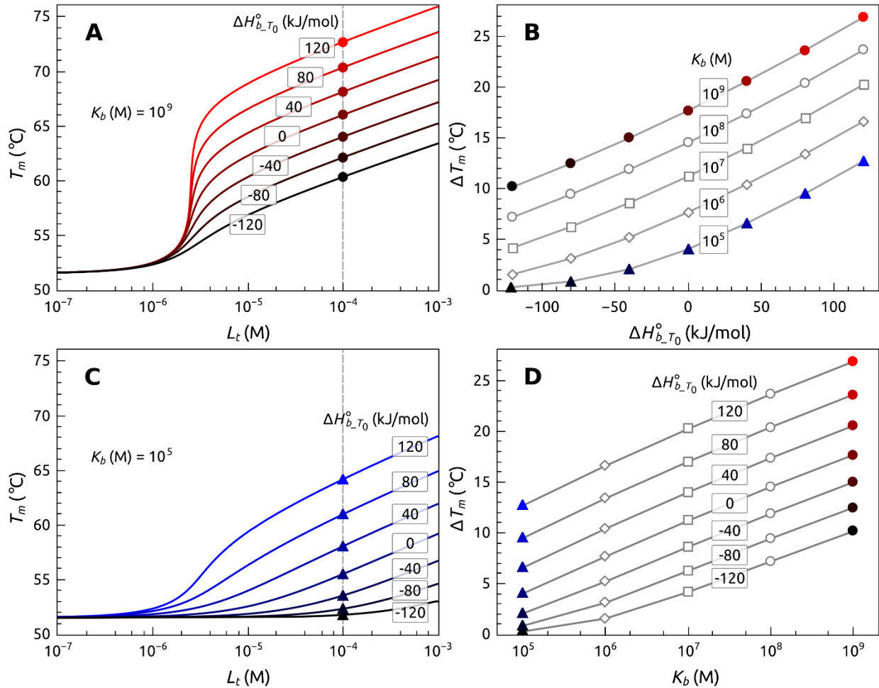
Figure 3. Simulations of expected T_m changes as a function of ligand binding enthalpy ( \Delta H_{b\_T_0}^0 ) and association constant ( K_b ). (A) Simulated titration curves for K_b = 10^9 \text{ M}^{-1} with enthalpy values varied from -120 to 120 kJ mol -1 . (C) Simulated titration curves for K_b = 10^5 \text{ M}^{-1} with enthalpy values varied from -120 to 120 kJ mol -1 . (B) T_m shifts as a function of enthalpy ([POT1] = 5 \mu\text{M} ; [Lt] = 50 \mu\text{M} ). (C) The same T_m shift can arise from many combinations of K_b and \Delta H_{b\_T_0}^0 . These simulations used: \Delta H_{U\_T_r}^0 = 44200 \text{ J/mol} , \Delta C_{p\_U} = 15000 \text{ J/mol-K} , \Delta S_{U\_T_r}^0 = 1361.5 \text{ J/mol-K} , T_m = 51.5 \text{ }^\circ\text{C} , \Delta C_{p\_b} = -500 \text{ J/mol-K} and [POT1] = 5 \mu\text{M} . Other parameters were varied as indicated.
