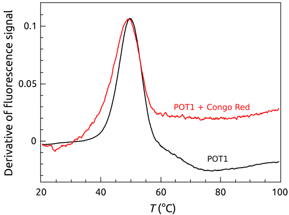
Figure 7. Effect of Congo Red on the thermal denaturation of POT1. There is no appreciable shift in T_m between POT1 (black curve) and POT1 + Congo Red (red curve). Conditions: [POT1] = 5 \mu M and [Congo Red] = 50 \mu M.
