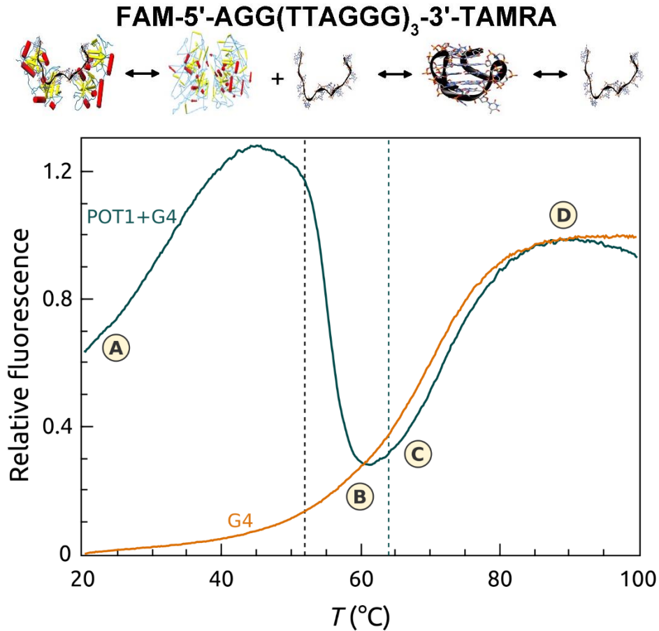
Figure 9. FTSA using FRET-labeled G4 DNA in the presence (green) and absence (orange) of POT1. This approach monitors the transition from the frame of reference of the G4 DNA. POT1 transitions would be invisible. The melting of the POT1-G4 complex is explained in the text. The dashed black vertical line shows the transition midpoint of POT1 from the protein frame of reference (Figure 1). The dashed green vertical line shows the transition midpoint of the POT1-G4 complex from the protein frame of reference (Figure 1).
