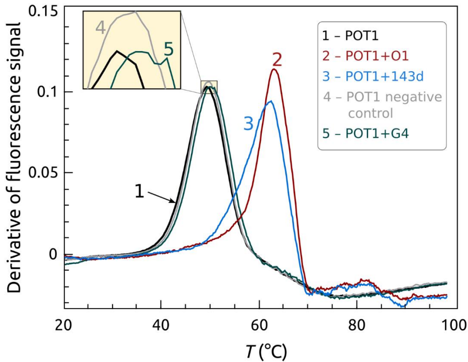
Figure 5. Binding of POT1 to a human telomeric G4 structure. POT1 binds to the initially folded telomeric sequence 5'AGGG(TTAGGG) 3 (143D) in a coupled reaction to form a single-stranded DNA-POT1 complex. The G4 is initially in a hybrid ("3+1") conformation under these conditions. FTSA monitors the T_m shift resulting from the stabilization of POT1 upon complex formation. POT1 will not unfold, or bind to, a non-telomeric G4 structure. The curves are: POT1 alone (1), POT1+O1 (2), POT1 + 143D (3), POT1 negative control (4), POT1 + G4 1XAV (5). POT1 = 5 \mu M and DNA = 50 \mu M.
