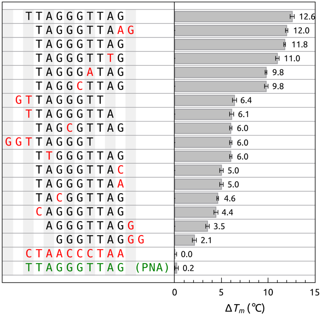
Figure 4. Screening of the binding of oligonucleotide sequence variants to POT1 by FTSA. The \Delta T_m for POT1 binding to O1 (5'-TTAGGGTTAG) and several sequence variants is shown. Conditions: [POT1] = 5 \mu M and [DNA] 50 = \mu M. The PNA sequence shows a \Delta T_m of only +1°C with [POT1] = 5 \mu M and [PNA] = 125 \mu M.
