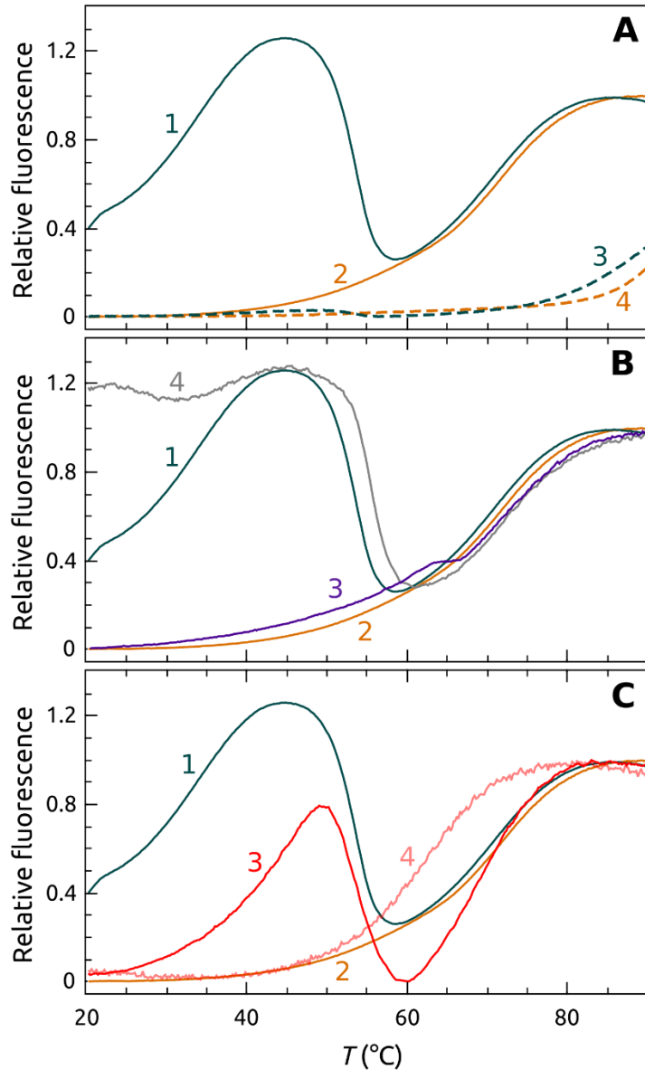
Figure 10. Three ways to inhibit POT1-G4 unfolding. (A) Inhibition of POT1 binding and unfolding by stabilizing G4 by ligand binding. The orange curve shows denaturation of G4 alone. The curve 1 shows the complicated melting of the POT1-G4 complex. Curve 2 shows melting of the G4 alone. Curves 3 and 4 show the denaturation of POT1 + G4 and G4 alone, respectively, in the presence of the G4 stabilizing ligand BRACO 19 at 1:100 (G4:BRACO 19). (B) Inhibition of POT1 by addition of 5'TTAGGGTTAG (O1), which binds competitively to POT1 to prevent G4 binding and unfolding. The curves 1 and 2 are the same as panel A. The curve 3 shows the denaturation curve for G4 + POT1+O1 at a ratio 1:10. The curve 4 is a control using the oligonucleotide 5'CTAACCTAA which does not bind to POT1. (C) Inhibition of POT1 by Congo Red (CR). The curves 3 and 4 show mixtures of G4+POT1+Congo Red. at 1:100 (POT1:CR) and 1:10 (POT1:CR), respectively. Curve 1 is the POT1 control; curve 2 is the G4 alone control.
