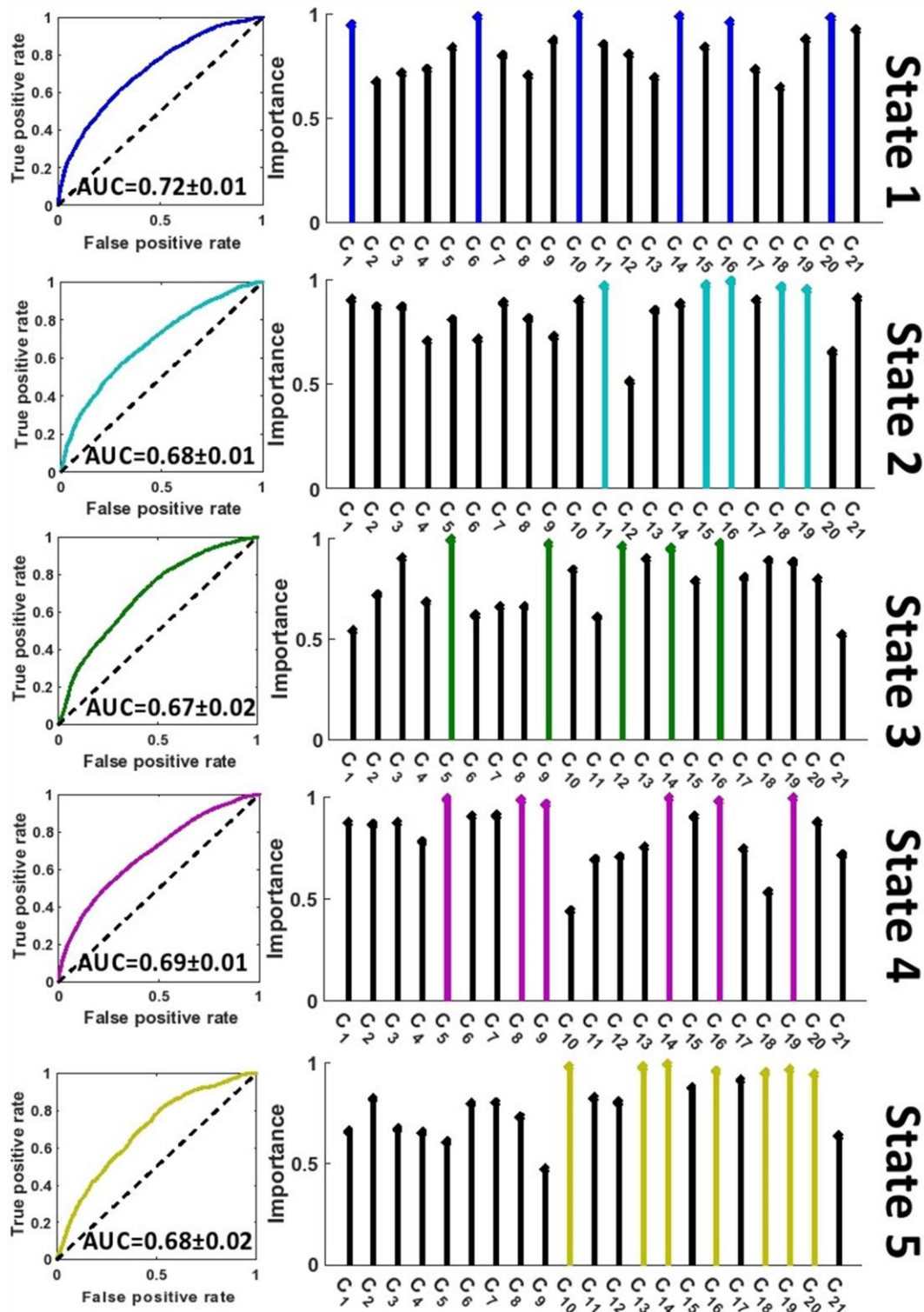
Figure 5. Feature selection results in FBIRN dataset. The left panel shows the receiver operating characteristic curve of the classification between SZs and HCs in each state. The right panel shows the relative importance of the features to the classification. The colorful features are groups of equally important features that were found to be of greater importance than the remaining features by a multiple comparison ANOVA test. The features (C 1 – C 21 ) are defined in Figure 2. AUC: Area under the curve.
