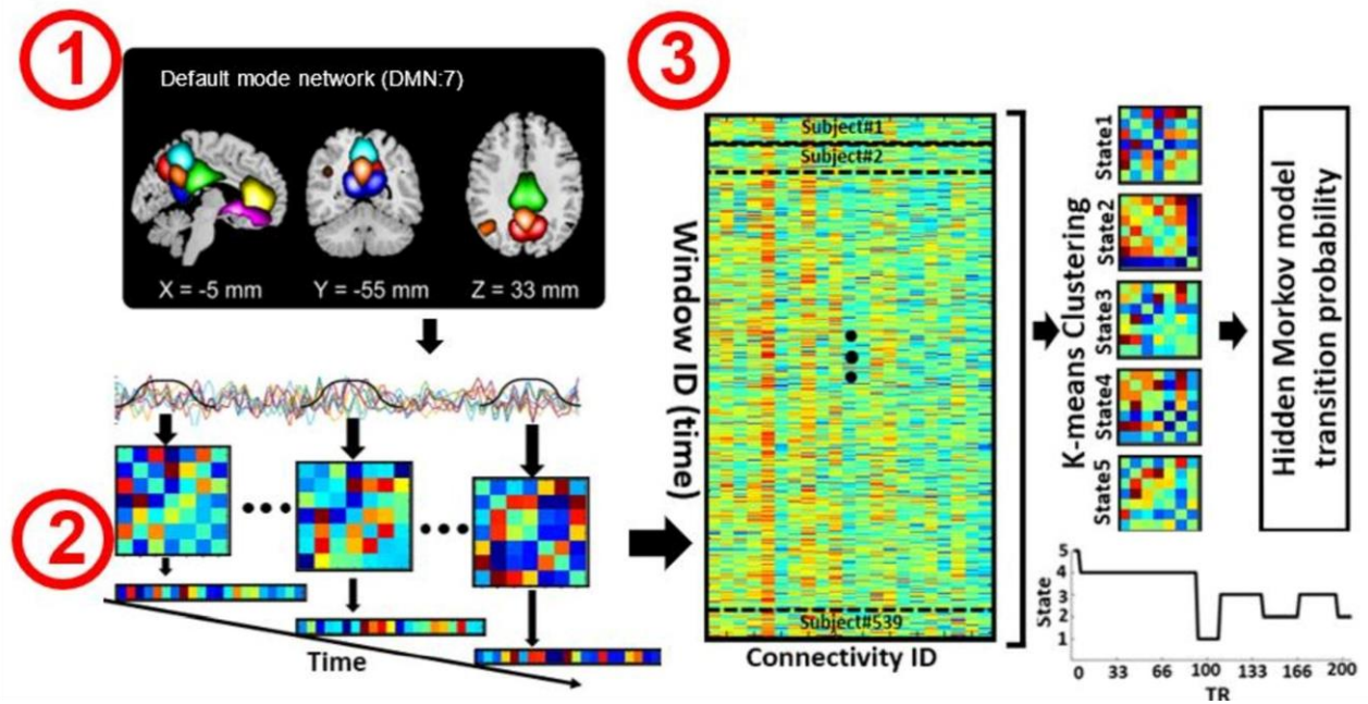
Figure 1. Analytic pipeline. Step1: The time-course signal of seven regions in the default mode network (DMN) has been identified using group-ICA. Step2: After identifying seven regions in the DMN, a taper sliding window was used to segment the time-course signals and calculate the FC matrix. Each FC matrix contains twenty-one connectivity features. Each feature represents the connectivity between a pair of DMN subnodes. Step3: After vectorizing the FC matrixes, we concatenated them applied and k-means clustering to group the FCs into five distinct clusters. Then, 25 hidden Markov model (HMM) features were calculated from the state vector of each subject. We investigated the association between HMM features and symptom severity in schizophrenia subjects.
