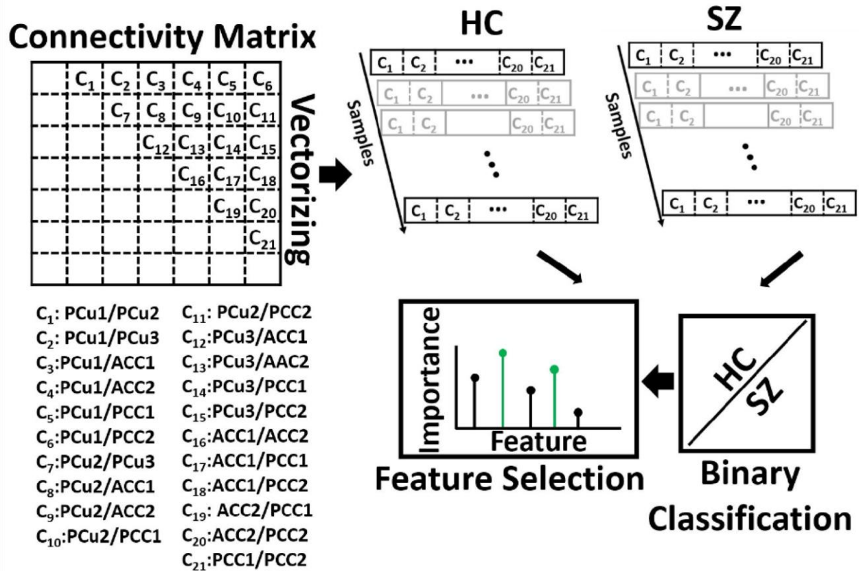
Figure 2. Feature selection. The connectivity features of seven default mode network (DMN) subnodes were used as inputs to fit a logistic regression classifier to discriminate SZs from HCs. With seven subnodes of the DMN, we had twenty-one connectivity features. The feature selection method, elastic net regularization (ENR), used the model generated by the classifier and the input features to identify the most predictive features. ACC: Anterior cingulate cortex, PCC: posterior cingulate cortex, PCu: Precuneus. Table 2 provides more information about different subnodes.
