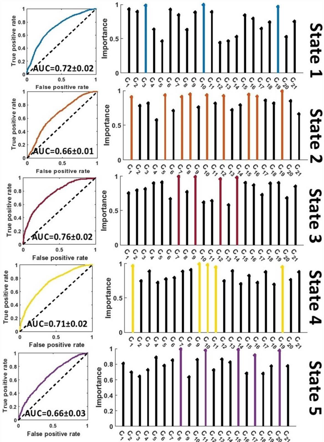
Figure 4. Feature selection results in COBRE dataset. The left panel shows the receiver operating characteristic curve of the classification between SZs and HCs in each state. The right panel shows the relative importance of the features to the classification. The colorful features are groups of equally important features that were found to be of greater importance than the remaining features by a multiple comparison ANOVA test. The features ( C_1 - C_{21} ) are defined in Figure 2. AUC: Area under the curve.
