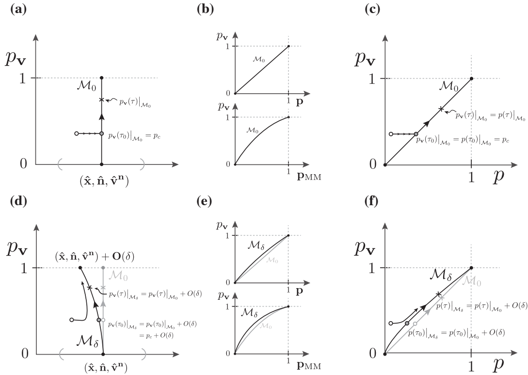
Figure 2: Panels (a)-(c) depict the fast and slow subsystems and the critical manifold \mathcal{M}_0 (89)-(90) (where \delta = 0 , Sections 6.1-6.2), and, panels (d)-(f) depict their singular perturbations and the slow manifold \mathcal{M}_\delta (where \delta small but non-zero, Section 7). (a) The phase-plane for the fast variables (\mathbf{x}, \mathbf{n}, \mathbf{v}^n) (the “ x -axis”) and the slow variable p_v . In the fast subsystem (Section 6.1) the slow variable p_v stays constant while the fast variables converge to (\hat{\mathbf{x}}, \hat{\mathbf{n}}, \hat{\mathbf{v}}^n) whenever \mathbf{x}(t_0) is in the neighborhood (indicated by gray semi-circles) of \hat{\mathbf{x}} for some initial time t_0 . A specific solution for the fast subsystem is depicted with small arrows and where the empty circle shows the initial condition for t_0 . The slow subsystem (Section 6.2) is constrained on \mathcal{M}_0 , and a particular solution is constructed by taking the steady state of the fast subsystem (where t \rightarrow \infty ) as the initial condition for the slow subsystem (\mathbf{x}(\tau_0), \mathbf{n}(\tau_0), \mathbf{v}^n(\tau_0), p_v(\tau_0)) = (\hat{\mathbf{x}}, \hat{\mathbf{n}}, \hat{\mathbf{v}}^n, p_c) . In this example p_v(\tau) \rightarrow 1 as \tau \rightarrow \infty . (b) The shape of \mathcal{M}_0 on the (\mathbf{p}, p_v) -plane where \hat{\mathbf{p}} = \mathbf{1}p_v (top panel) and (\mathbf{p}_{MM}, p_v) -plane where \hat{\mathbf{p}}_{MM} = \hat{\mathbf{r}}p_v + (\mathbf{1} - \hat{\mathbf{r}})p_v^2 (bottom panel). Note that the shape of \mathcal{M}_0 in the bottom panel depends on the steady state for relatedness \hat{\mathbf{r}} . (c) Phase-plane for the fast (and slow) arithmetic mutant frequency p (58) and the slow reproductive value weighted mutant frequency p_v (the notation is identical to panel (a)). Note that p = p_v on \mathcal{M}_0 and that their dynamics on \mathcal{M}_0 is as given in (91) and (94). (d) The phase plane for (\mathbf{x}, \mathbf{n}, \mathbf{v}^n, p_v) as a singular perturbation of (a) where, in particular, the slow manifold \mathcal{M}_\delta is O(\delta) -close to \mathcal{M}_0 as is the initial condition (gray circle) and the solution on \mathcal{M}_\delta . Moreover, because \mathcal{M}_\delta is a stable manifold, the solutions in the neighborhood of \mathcal{M}_\delta approach the solutions on \mathcal{M}_\delta . (e) The shape of \mathcal{M}_\delta as a perturbation of \mathcal{M}_0 discussed in (b). (f) The phase plane for (p, p_v) as a singular perturbation of (c). Note that the solutions p(\tau)|_{\mathcal{M}_\delta} and p_v(\tau)|_{\mathcal{M}_\delta} are O(\delta) -distance away from each other because \mathcal{M}_\delta lies off-diagonal. The interpretation of the solutions are identical to (d).
