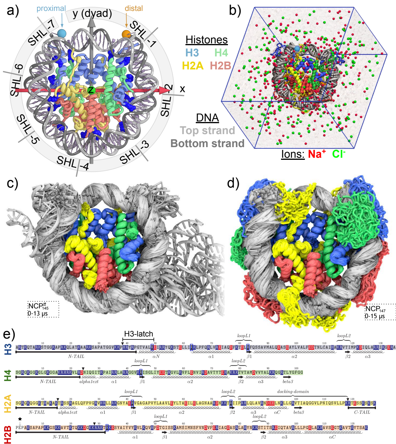
Figure 1: Overview of NCP structure and dynamics. a) NCP and its reference axes (z - superhelical, y - dyad). White arrows on DNA strands show 5'-3' direction. Spheres highlight the proximal and distal ends of the double helix. Superhelical locations (SHL) are shown for the proximal half of the DNA (SHL<0). Proximal H3-H4/H2A-H2B dimers are in the front (z>0). Key arginines inserted in DNA minor grooves are shown in dark blue. b) NCP in a simulation box with solvent. c-d) Dynamics of NCP with truncated and with full-length histone tails (NCP tt 145 and NCP 147 systems, respectively). Overlay of MD snapshots spaced 0.1 μs apart. e) Sequences of the core histones and their secondary structure features: α-helices, β-strands, loops, flexible histone tails, etc. For simulations with truncated histone tails, the respective positions are marked with ▼. Positively and negatively charged residues are highlighted in blue and red, respectively. Key arginines are highlighted with dark blue frames. * - H2B residues absent in the recombinant protein.
