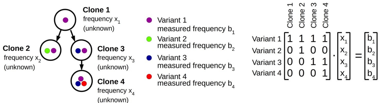
Figure 1: Computational approach. Clonal hierarchies are rooted trees. The root of the tree either corresponds to wild type cells or to the AML founder clone. The coloured dots represent different alleles or mutations. From bulk sequencing the allele frequencies b_i in the sample are known. The frequencies x_i of the different clones are unknown. The tree structure is represented by a triangular matrix. The measured data is compatible with the tree structure if the system Ax=b has a non-negative solution.
