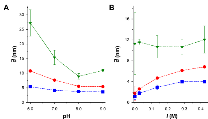
Figure 4. DLS measurements on SMAc co-polymers X25 (circles), X30 (squares) and C30 (triangles). SMAc particle sizes ( n = 3 ) are reported as a function of pH at constant buffer composition (A) and ionic strength at constant buffer pH (B). Buffer compositions are given in Table 2.
