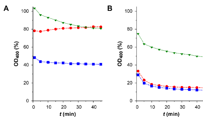
Figure 5. Turbidimetric profiles of SMALP formation for wt-HEK293T membrane suspensions (2%, m/v) mixed 1:1 (v/v) with different SMAc co-polymers (1% in KP10 buffer, pH 8.0, m/v): X25 ( circles ), X30 ( squares ) and C30 ( triangles ). (A) Membranes suspended in SB500 buffer. (B) Membranes suspended in SB0 buffer.
