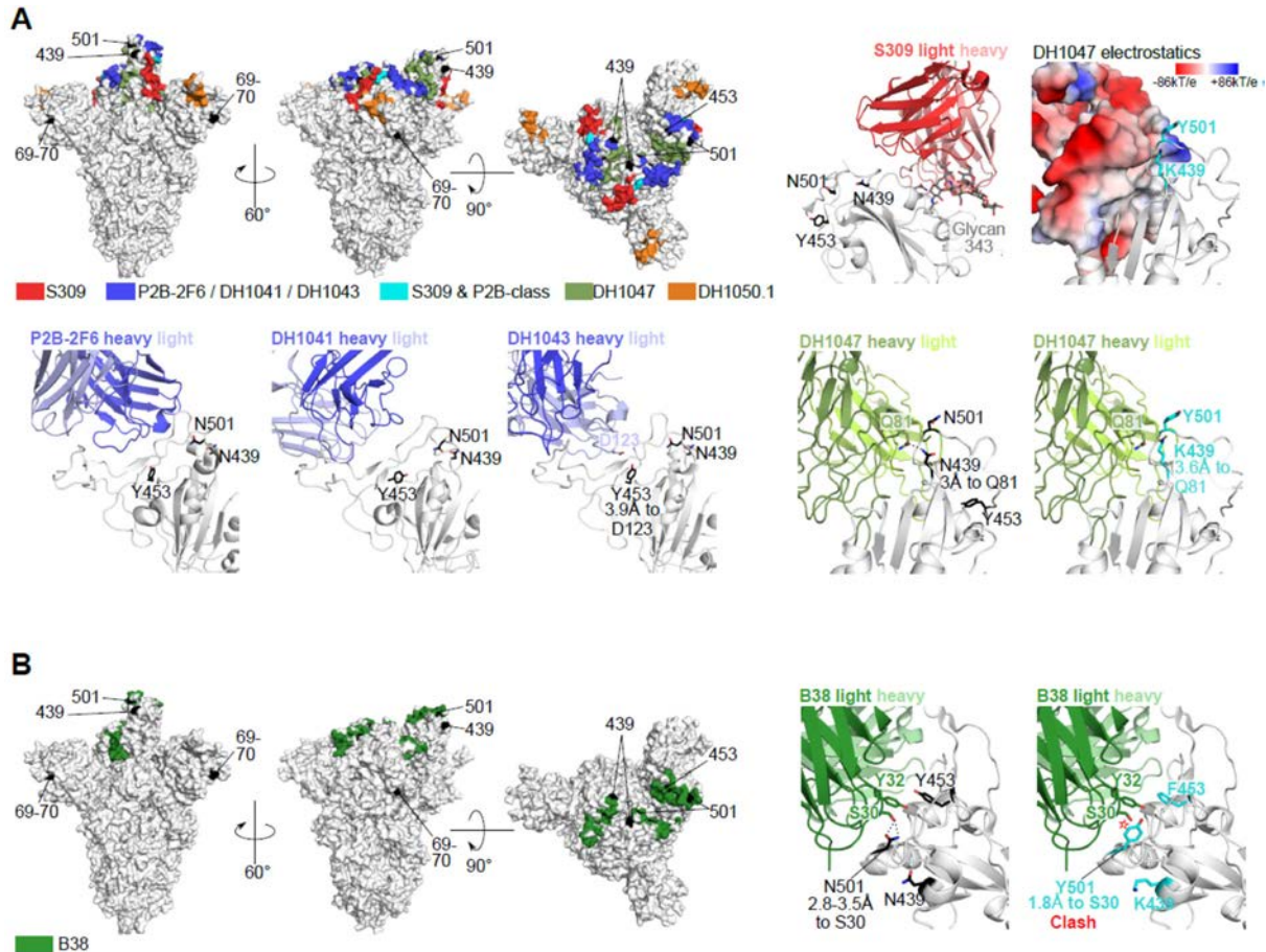
Fig 3. Structural analyses for antibody resistance mutations. (A) Top left 3 panels: Full spike trimer with antibody epitopes for S309, P2B-2F6, DH1041, DH1043, DH1047 and DH1050.1. Epitopes for P2B-2F6, DH1041 and DH1043 are similar and are grouped together. Top row, second from right panel shows location of spike sites 439, 453 and 501 with respect to S309. These spike sites are not close to S309 ( >11\text{\AA} ). Top row rightmost panel shows the DH1047 antibody colored according to vacuum electrostatic potential, and the modeled mutations at spike sites Lys-439 and Tyr-501. Bottom row, rightmost two panels DH1047 interaction with sites 439, 453 and 501 using wildtype amino acids (second from right) and modeled mutations (rightmost). Bottom row, left 3 panels show the location of spike sites 439, 453 and 501 with P2B-2F6, DH1041 and DH1043. Polar interactions between antibody and spike residues of interest are shown with dotted black lines. (B) Similar to (A) except with B38 antibody. The modeled Tyr-501 is predicted to clash with light chain Ser-30 ( \sim 1.8\text{\AA} , red star).
