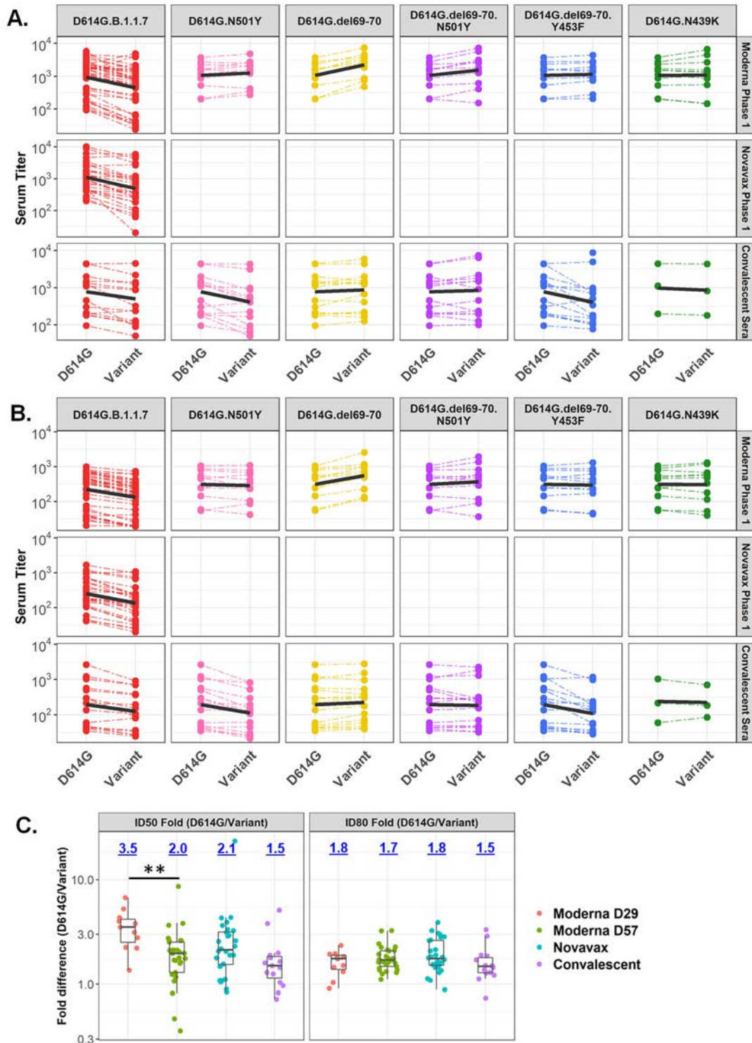
Figure 2. Neutralization of variants by vaccine and convalescent sera. Serum ID50 (A) and ID80 (B) titers of neutralization of each variant, as indicated on top of each panel, relative to D614G by vaccine sera (top 2 rows) and convalescent sera. Dashed thin lines represent individual samples, thick black lines represent geometric means of each sample group as indicated on the right. NT- not tested. Also see Table S1. (C) Fold decline of ID50 (left) and ID80 (right) titers for each variant over D614G (D614G/variant) for each serum sample set as identified. Numbers on top of each plot show median fold differences. Upper and lower border of each box represent IQR of the fold differences respectively, and the middle bars in boxes represent group median. Statistical significance of comparisons are indicated in all panels as: * p < 0.042 (corresponding to q < 0.1 ). ** p < 0.01 . *** p < 0.001 . **** p < 0.0001 . Wilcoxon signed-rank paired test for (A) and (B); Wilcoxon rank-sum test for (C). Also see Table S2.
