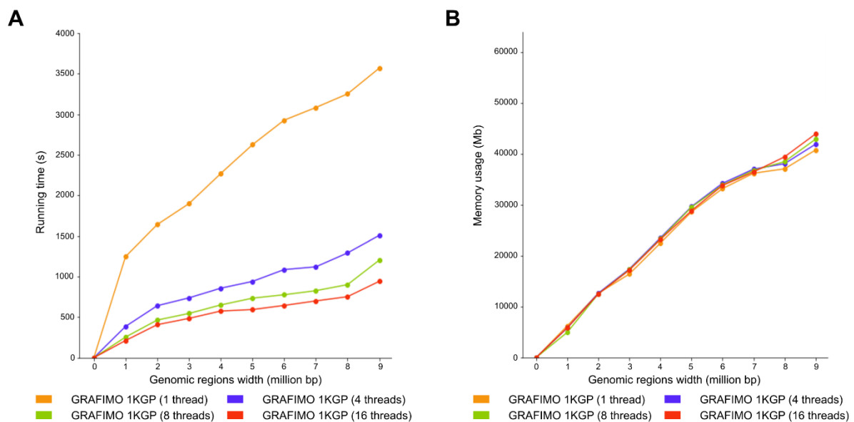
S9 Fig. GRAFIMO running time efficiently scales with the number of threads used. By running GRAFIMO with multiple threads (A) the running time significantly decreases, while (B) memory usage remains similar.
