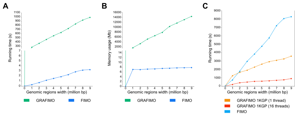
S8 Fig. Comparing GRAFIMO and FIMO performance. (A) FIMO is faster than GRAFIMO (using a single thread) when searching CTCF motif (JASPAR ID MA0139.1) on human chr22 regions (total width ranging from 1 to 9 millions of bp) and without accounting for genetic variants. (B) FIMO uses less memory resources than GRAFIMO, however it can only scan linear sequences. (C) GRAFIMO is generally faster than FIMO in searching potential CTCF occurrences after 1Mbp when considering genetic variation present in large panels of individuals as 1000GP on GRCh38 phase 3 (2548 samples), even with a single thread.
