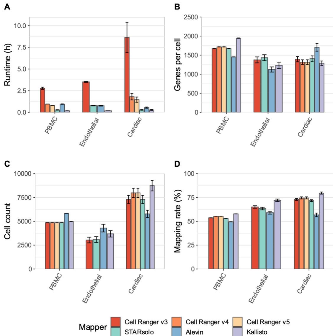
Figure 1 Summary of major measurements including runtime in hours (A), Genes per cell (B), cell count (C) and the mapping rate in percent (D). All bar plots show the mean of all samples with the standard error.
