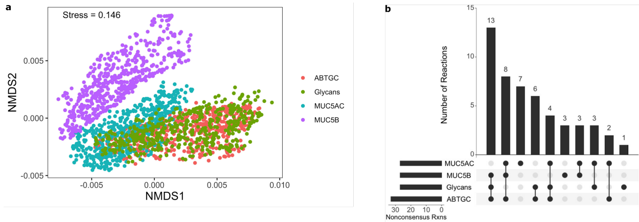
Figure 3: Contextualization of updated reconstruction shows shifts in P. aeruginosa metabolism in response to mucins and mucin components. (a) NMDS analysis of flux samples ( n = 500 ) from each contextualized model. (b) Comparison of non-consensus reactions present within models displays subsets of reactions that are shared by groups of contextualized models.
