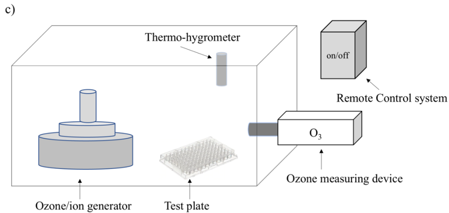
Figure Legend: ICON3 operating in a common room, with the ozone flow coming out of a 2 meters high rod from top to bottom (a); equipment for ozone gas administration in a plastic box under a biological safety cabinet (b); schematic representation of laboratory setup under biological safety cabinet (c).
