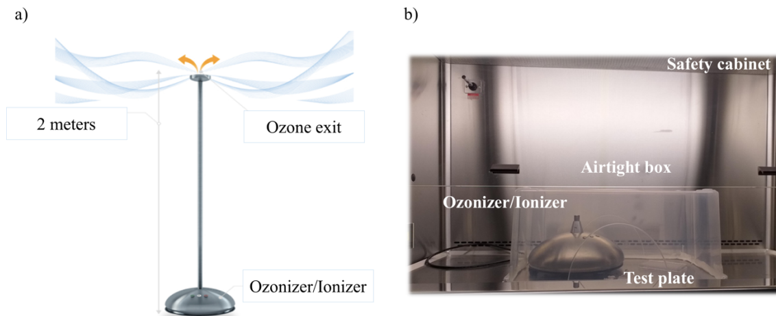
Figure 1. ICON3 ozone/negative ions generator
