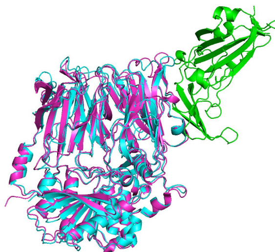
Figure 5. Putative binding mode between SARS-Cov2 (S) receptor-binding domain (RBD) (green) and dipeptidyl peptidase-4 (DPP4) (cyan). The multimeric template framework is PDB entry 4L72 (pink).
