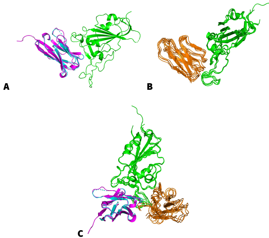
Figure 4. Putative binding modes of SARS-CoV2 receptor-binding domain (green) and (A) the top-ranking model of myelin-oligodendrocyte glycoprotein (cyan) with the homologue template of PDB entry 7C8V (pink) and (B) a cluster of secondary models (orange). (C) Display of both binding modes in complex with SARS-CoV2 receptor-binding domain.
