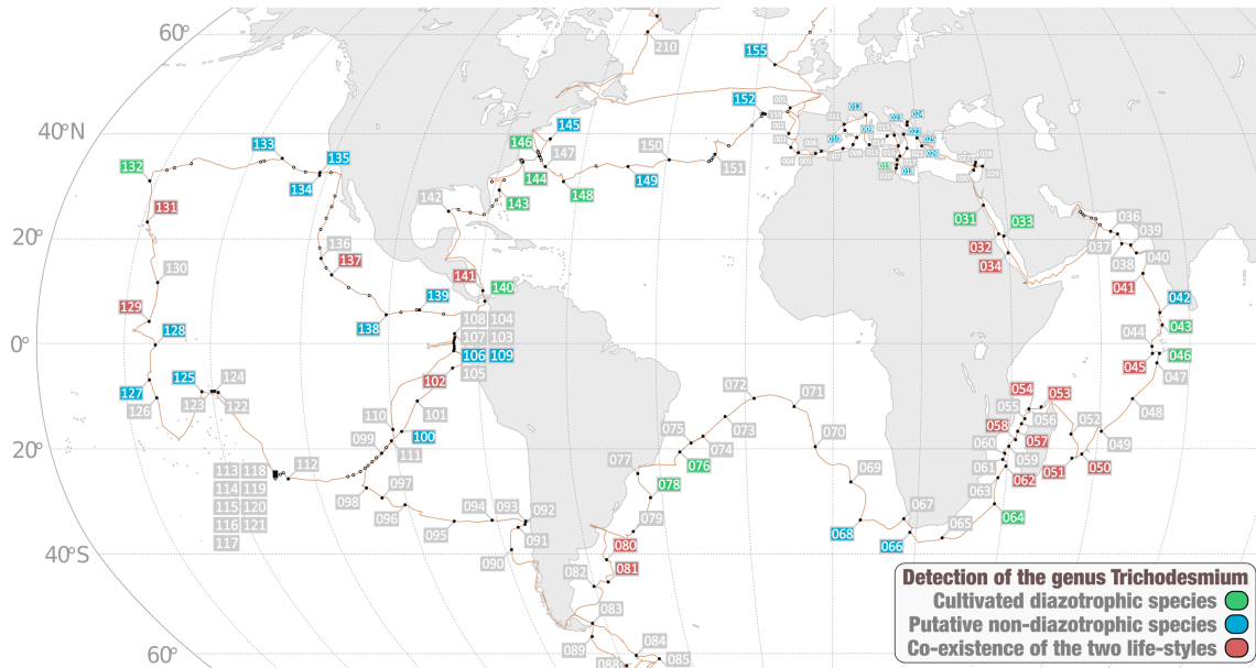
Figure 5: Detection of Trichodesmium species across the Tara Oceans stations. The world map describes stations in which we detected (1) only T. erythraeum and/or T. thiebautii (diazotrophic species), (2) only ‘ Ca. Trichodesmium miru ’ and/or ‘ Ca. Trichodesmium nobis ’ (putative non-diazotrophic species), (3) or species from both groups. This surveys covers all size fractions >0.2 \mu\text{m} .
