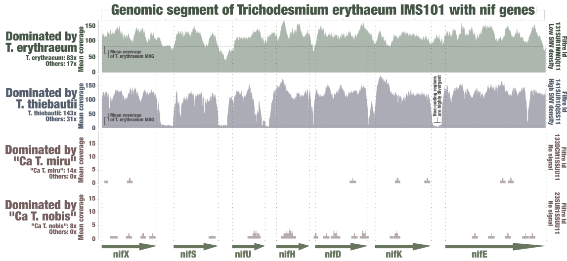
Figure 4: Metagenomic signal for the nif operon of Trichodesmium erythraeum . The figure displays read recruitment for the T. erythraeum IMS101 nif operon across four metagenomes, each dominated by a single Trichodesmium species (low mapping stringency of >70% identity over >70% of the read length; anvio visualization).
