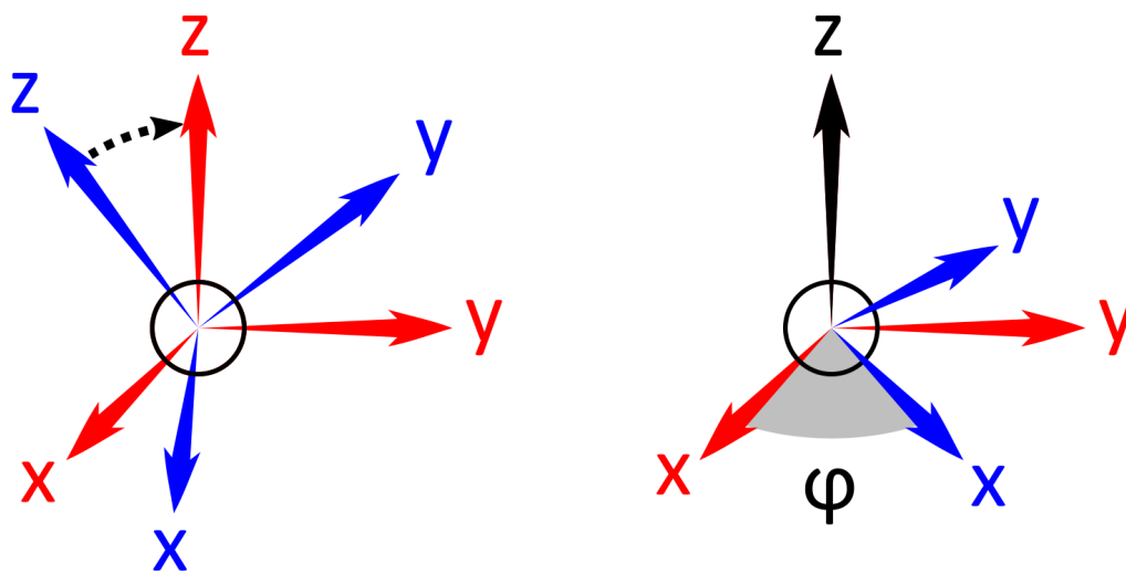
Figure 5: The torsional angle \phi is obtained by first aligning the z axes of the OFRs of the cargo and the NLSJ (left). Once the axes are aligned, \phi is given by the angle between the corresponding axes in the two OFRs (right).
