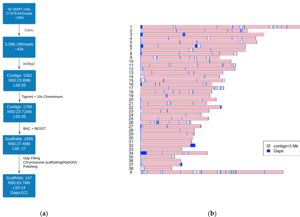
Figure 1. Dog_10k_Boxer_Tasha_1.0 assembly. (a) Assembly pipeline (b) Ideogram showing chromosomes, contigs, gaps.
