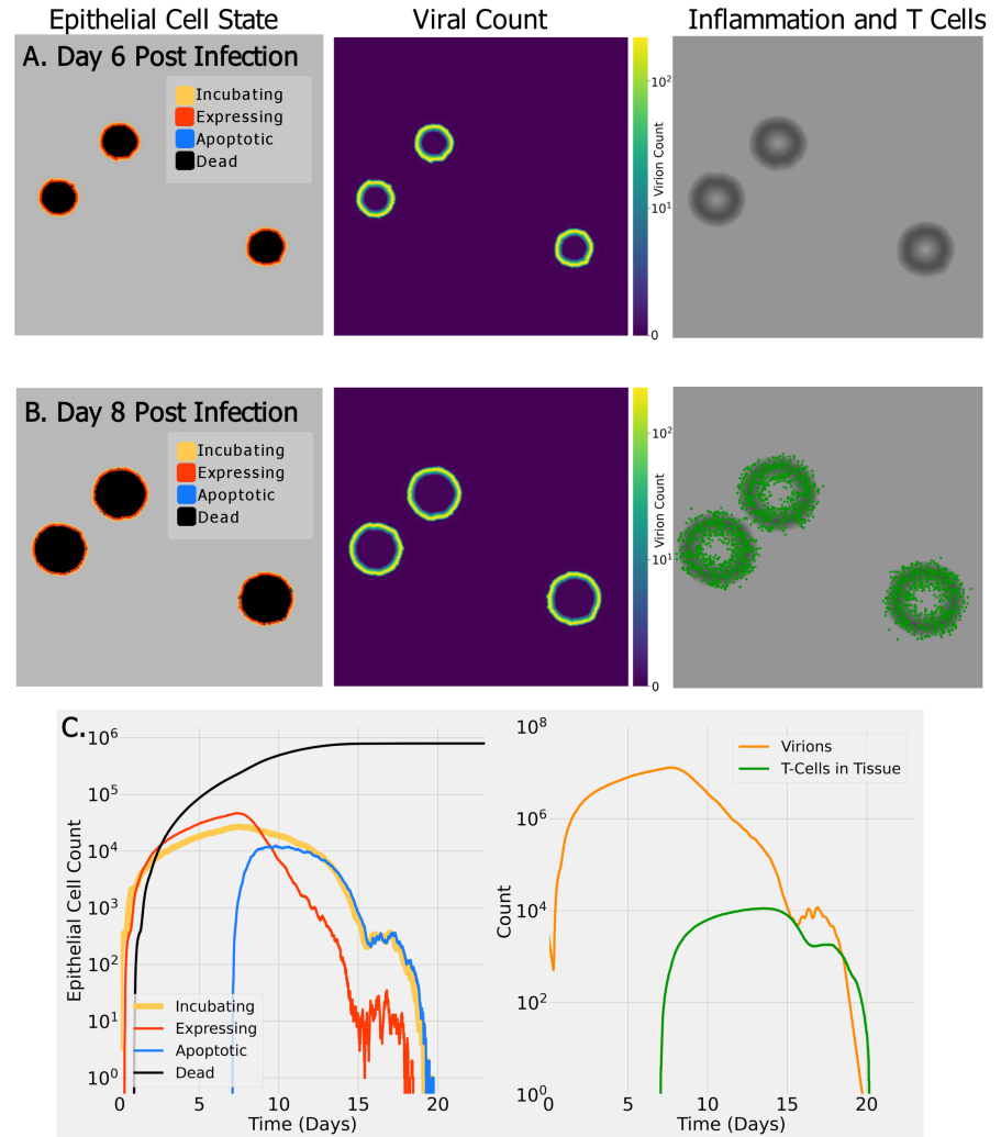
Fig 2. Example SIMCoV simulation on a 15 x 15 mm 2 layer of epithelial tissue. (A) six days post infection (dpi); (B) eight dpi. Color indicates epithelial cell state (see legend, left column), virus concentration (see scale bar, middle column), and presence of inflammatory signal (in grayscale with darker regions having a stronger signal, right column) and T cells (green); (C) (left panel) shows the dynamics of epithelial cell state, and (right panel) shows virus and T cell dynamics. A video demonstration of this simulation can be viewed at https://www.youtube.com/watch?v=5K4ZSeCn-Ks .
