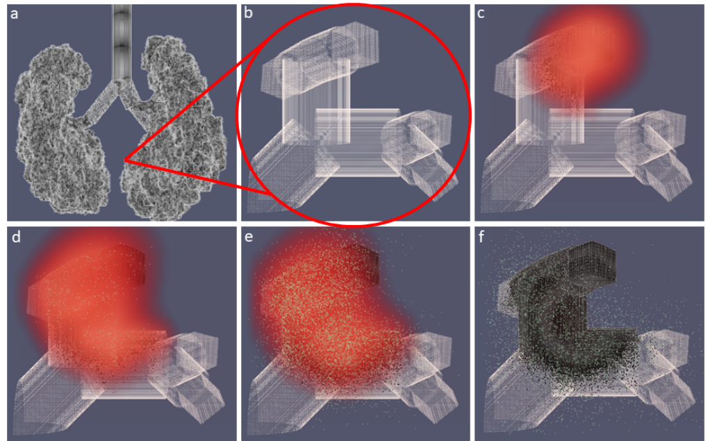
Fig 6. Simulated 3D branching airway with a single FOI. (A) shows the full lung model; (B) - (F) show T cells (green), virions (red) and a small region of epithelial cells (gray) at (B) 0 dpi, (C) 4.2 dpi, (D) 6.3 dpi, (E) 6.9 dpi, and (F) 8.3 dpi. Dead epithelial cells are indicated in black. A video corresponding to these images is available at https://youtu.be/WbiLH9NRfba .
