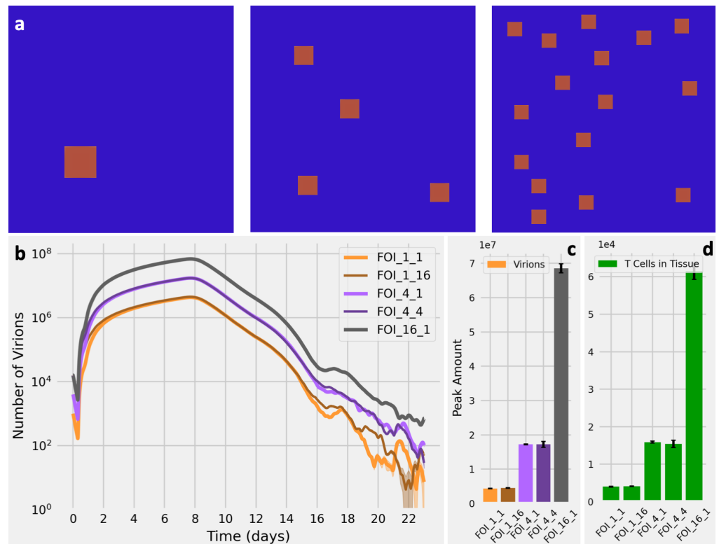
Fig 3. Effect of the number of FOI on virus and T cell dynamics. (A) Initial spatial distribution in SIMCoV for one FOI (left), four FOI (center), and 16 FOI (right). (B) Viral load over time given different FOI. The light orange line labelled FOI_1_1 represents one FOI initialized with a single infected cell, and the dark orange line labelled FOI_1_16 represents one FOI initialized with a cluster of 16 infected cells. Similarly the purple lines represent four FOI, each initialized with one or four infected cells; the black line represents 16 FOI, each with one infected cell; 30 replicates with shading showing 95% CI (which is only visible at low numbers of virions). (C) Peak number of virions for different FOI with error bars showing the standard deviation for 30 replicates. There is a 3.90-fold increase from the one FOI configuration to the four FOI configuration and a further 3.99-fold increase in the 16 FOI configuration. The peak virions given FOI_1_1 and FOI_1_16 are indistinguishable ( p = 0.68 ), as are the FOI_4_1 and FOI_4_4 cases ( p = 0.51 ); however the single FOI, 4 FOI and 16 FOI cases are distinguishable from each other ( p < 0.01 ). (D) Peak number of T cells that extravasate into lung tissue for the different FOI. Similar to panel (C), the increase is 3.95-fold for each 4-fold increase in FOI.
