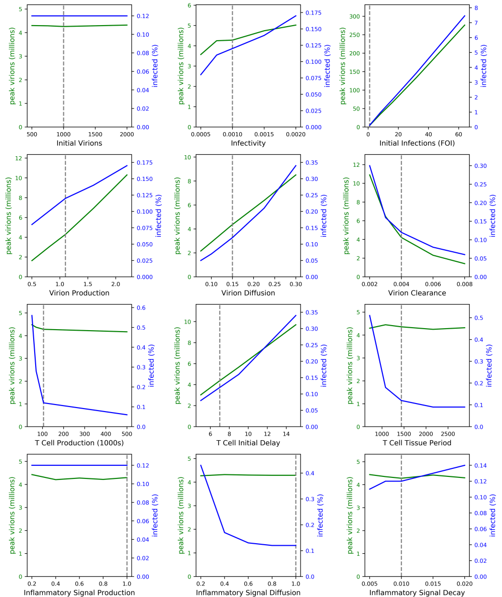
Fig 8. The effect of varying model parameters, one at a time. Each line is the average of five runs. Dashed lines indicate SIMCoV default values.
