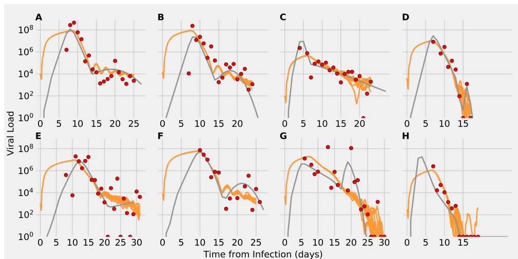
Fig 5. Viral load predictions from SIMCoV simulations (orange) compared to the extended ODE in [12] (gray), and patient data from [36] (red points). For each simulation, 10 random runs are shown.
