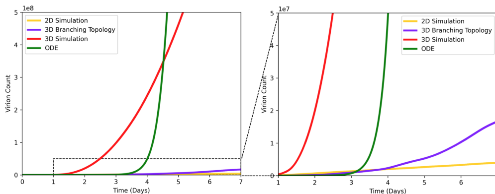
Fig 7. Viral spread given different model topologies. Virion count is plotted vs. time for four different SIMCoV configurations: 2D grid (yellow); 3D grid (red); 3D branching model (blue); ODE model (green). The right panel is zoomed in on the y-axis (showing up to 10^7 virions) to show the dotted region of the left panel (which shows up to 10^8 virions).
