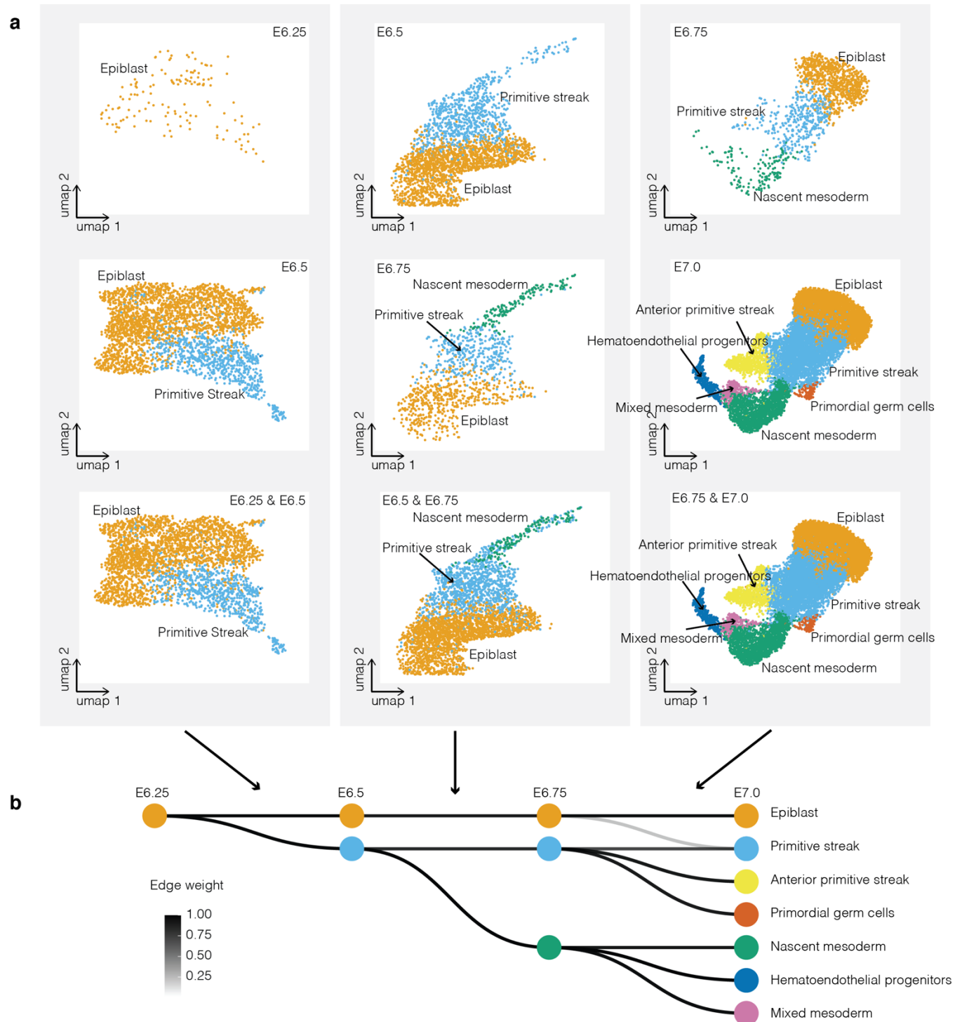
Supplementary Figure 2. Inference of epiblast derivatives between E6.25 and E7.0. a , A portion of the UMAP corresponding to the epiblast and its inferred derivatives is shown for co-embeddings of E6.25 → E6.5 (left column), E6.5 → E6.75 (middle column) and E6.75 → E7.0 (right column). Within each column is the same UMAP visualization, but showing only cells from the earlier timepoint (top row), the later timepoint (middle row) or both timepoints (bottom row). b , Directed acyclic graph showing inferred relationships between cell states amongst early epiblast derivatives. All edges with weights above 0.2 are shown in grey scale.
