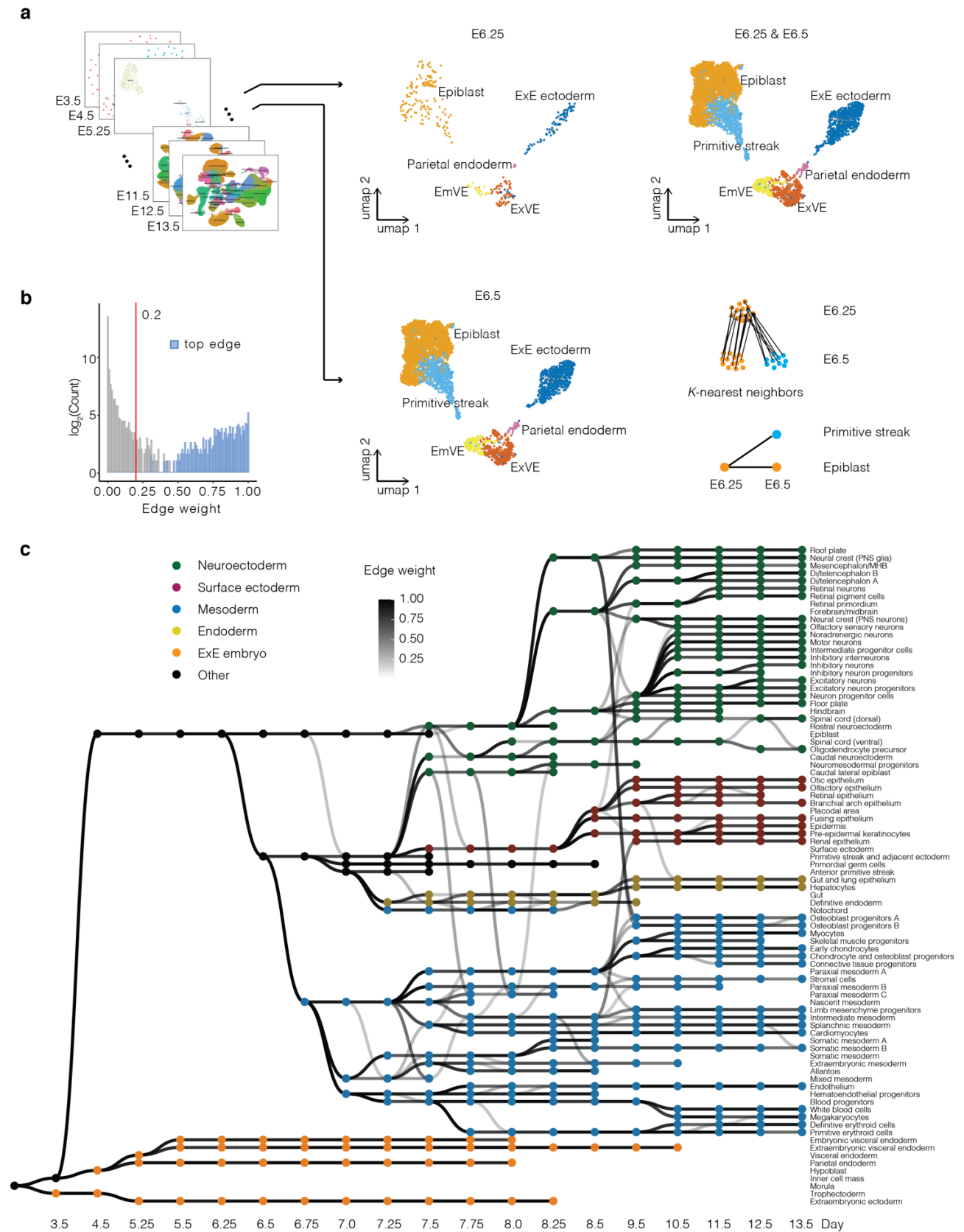
Figure 1. Systematic reconstruction of the cellular trajectories of mouse embryogenesis. a , Overview of approach. Cells from each pair of adjacent stages were projected into the same embedding space (Stuart et al. 2019). UMAP visualizations of co-embedded cells from E6.25 and E6.5 are shown separately (middle column) or
