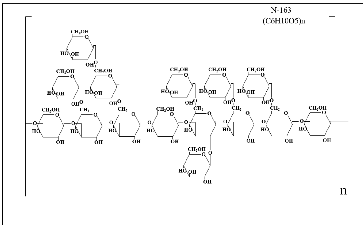
Figure 1: Structure of beta glucan derived from the AFO-202 strain with the chemical formula (C 6 H 10 O 5 ) n
