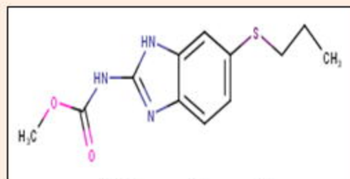
Albendazole
