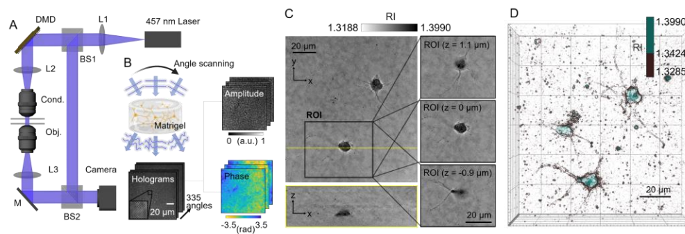
Fig. 2. 3D RI measurement of cultured neurons using ODT. A Schematic of the ODT system based on the Mach-Zehnder interferometry with a DMD. B The neurons were cultured inside a Matrigel scaffold and imaged in 3D using ODT. The laser beam illuminated the sample from 335 different angles and each illumination generated a hologram. From the 335 holograms, the amplitude and the phase information of the sample were retrieved, from which the 3D RI tomogram was reconstructed. C Representative tomogram of a cultured neuron in a Matrigel scaffold. The ROI indicates a neuron and its 2D sections at various axial positions. D RI-based 3D-rendered volume of the tomogram shown in Fig. 2C. The measured RI values were higher (1.3424–1.3990) in the soma than those in the neurites (1.3285–1.3424).
